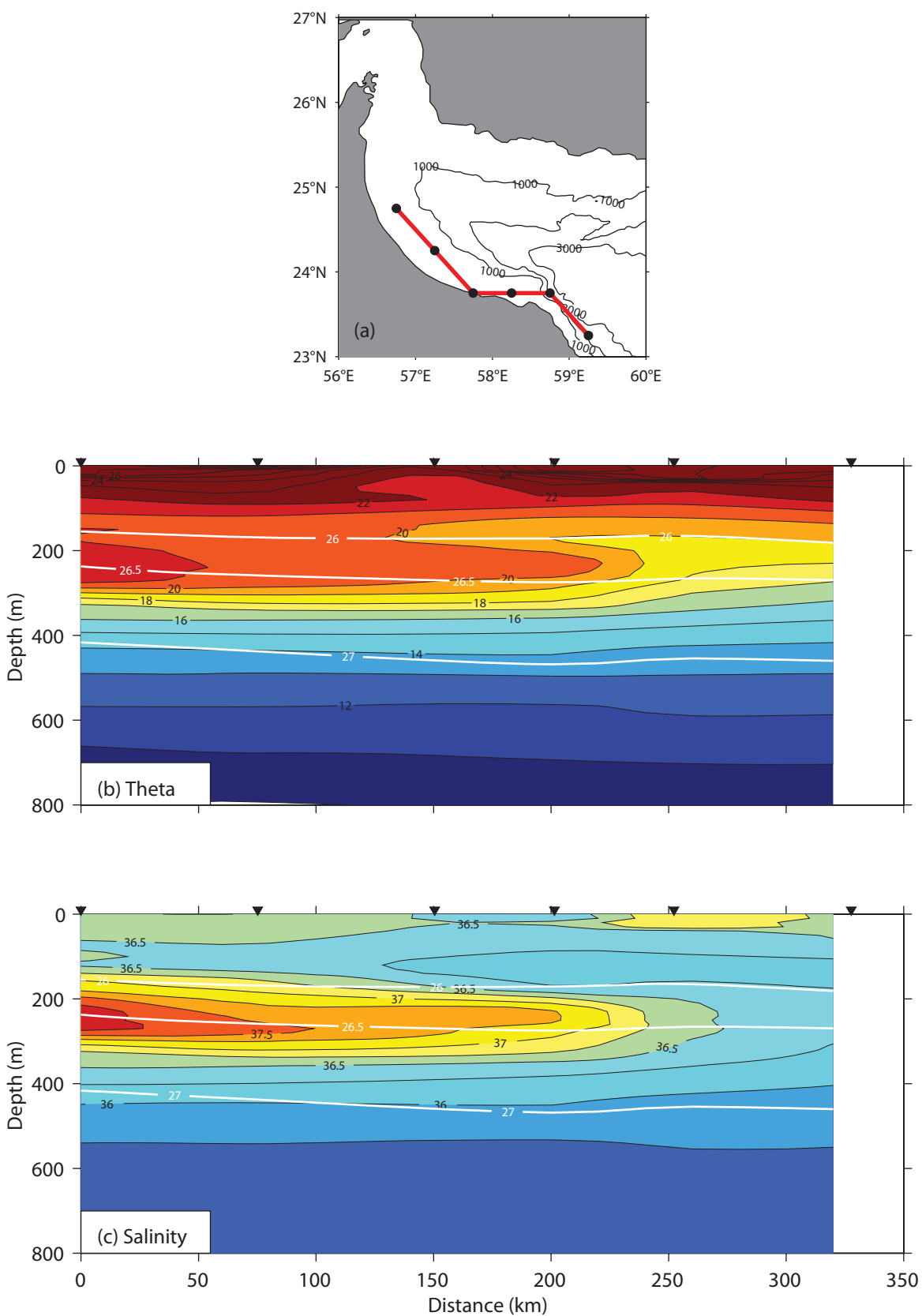
FIGURE 10 "Character and Dynamics of the Red Sea and Persian Gulf Outflow" JGR 2000 Bower et al.
