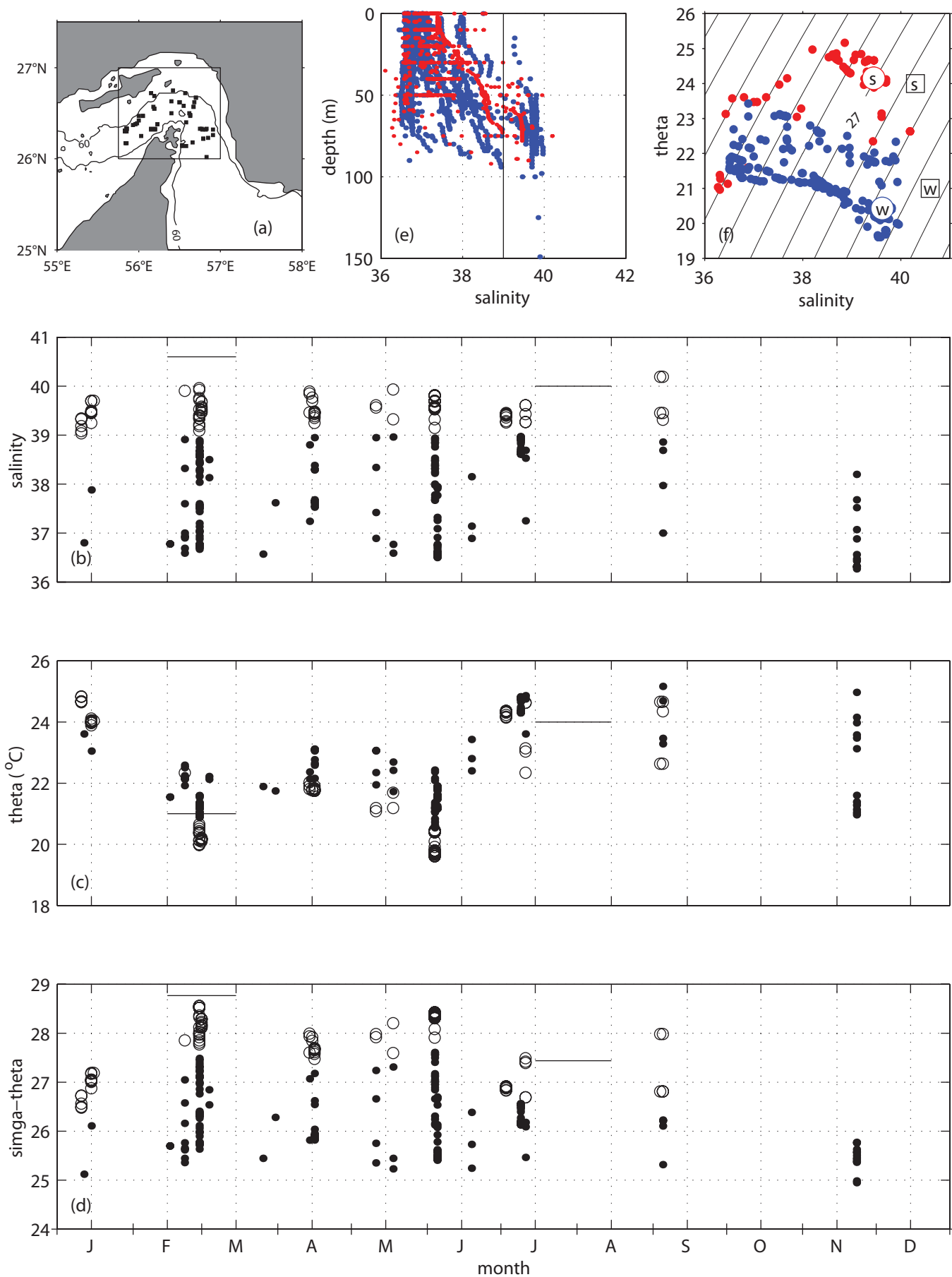
FIGURE 9 "Character and Dynamics of the Red Sea and Persian Gulf Outflow" JGR 2000 Bower et al.
