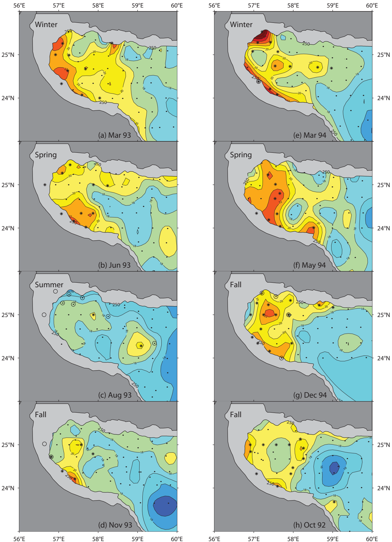
FIGURE 13 “Character and Dynamics of the Red Sea and Persian Gulf Outflow” JGR 2000 Bower et al.
