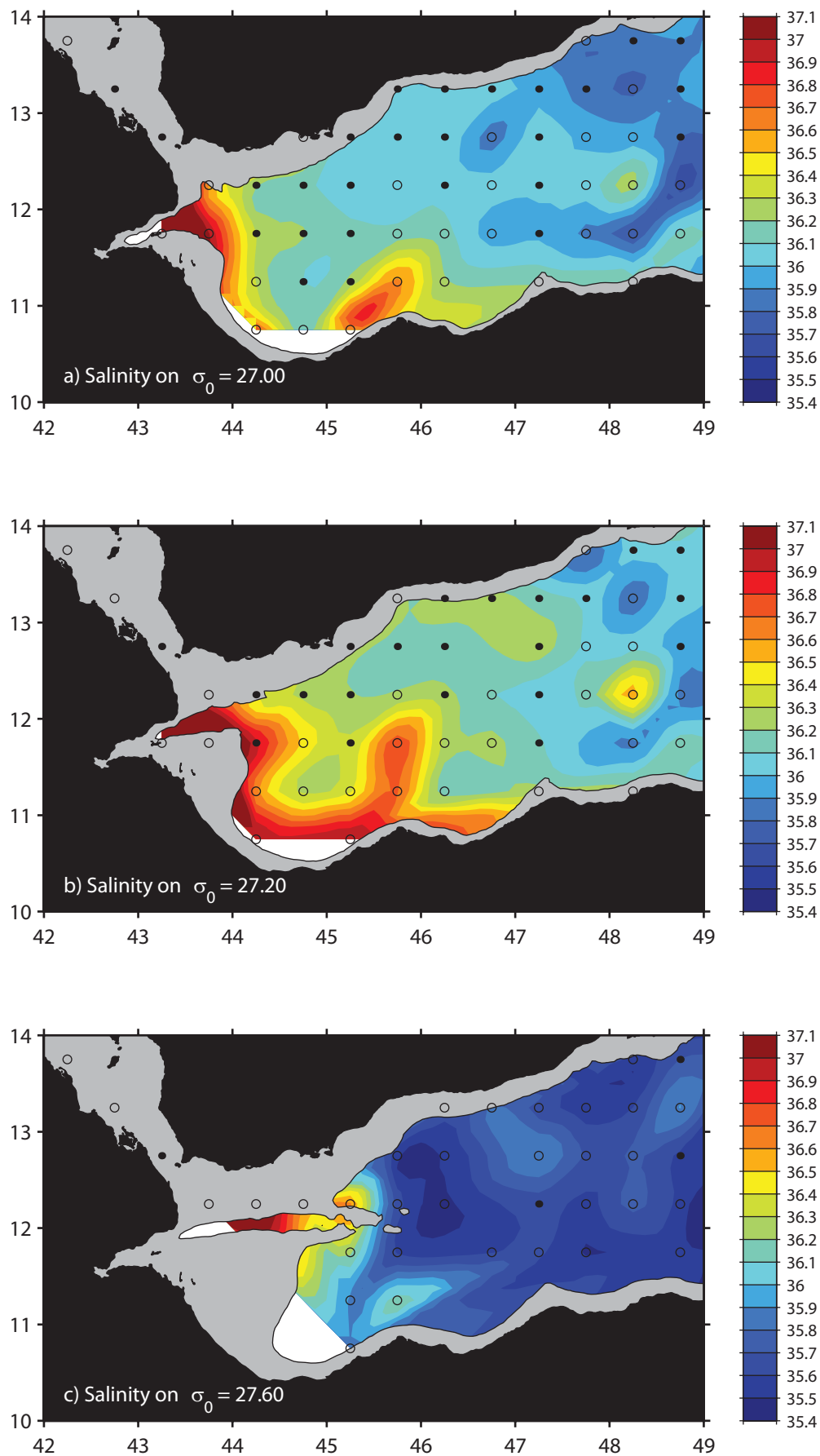
FIGURE 7 "Character and Dynamics of the Red Sea and Persian Gulf Outflow" JGR 2000 Bower et al.
