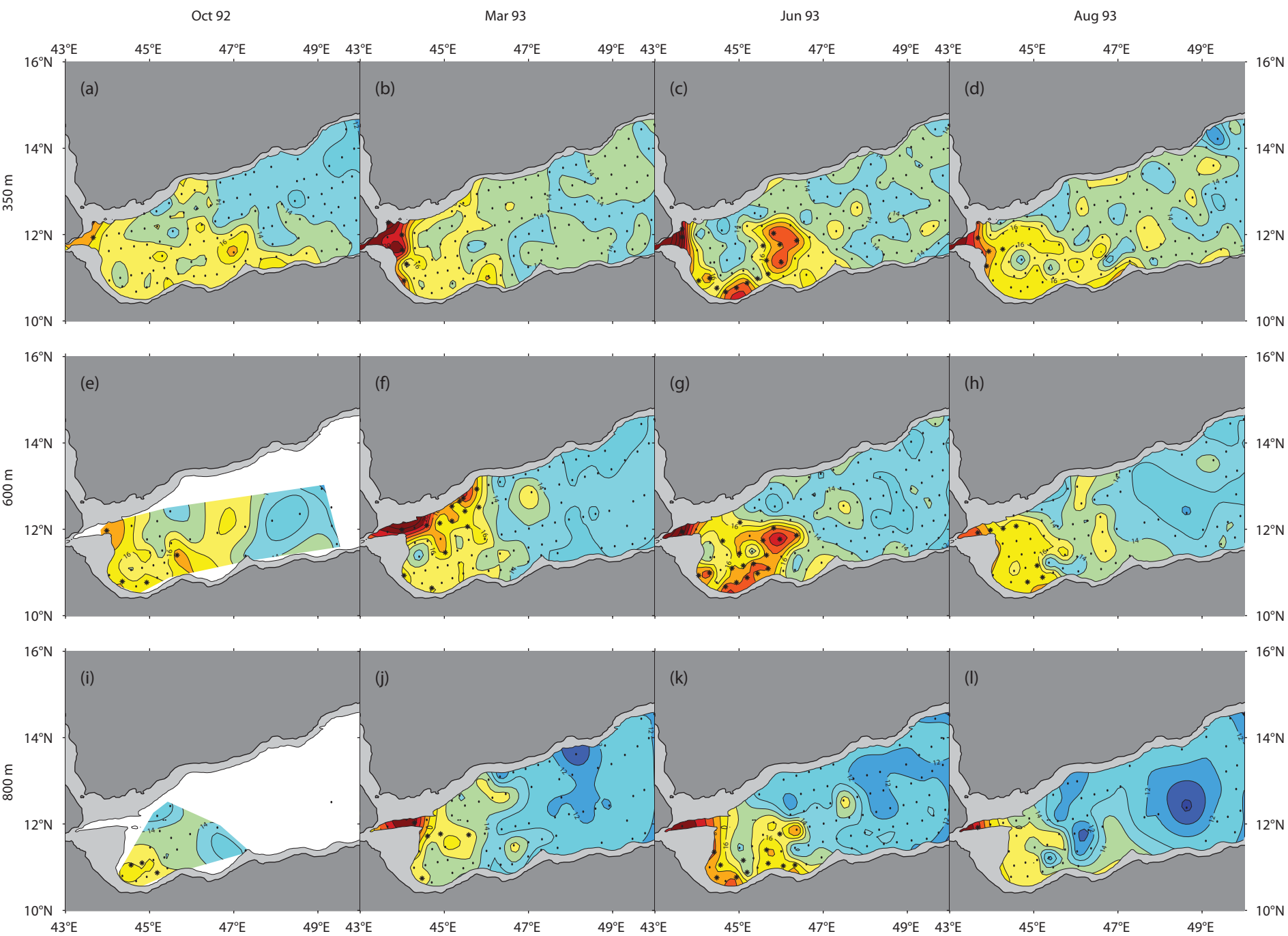
FIGURE 8 "Character and Dynamics of the Red Sea and Persian Gulf Outflow" JGR 2000 Bower et al.
