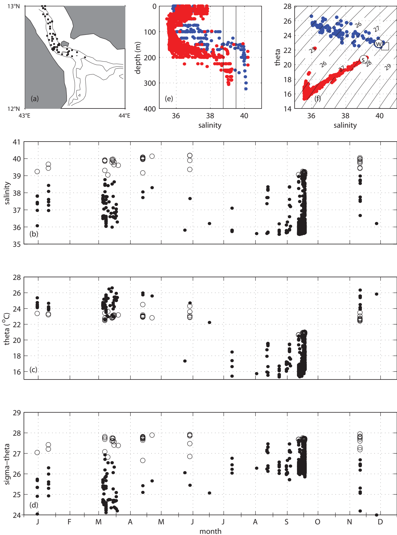
FIGURE 3 "Character and Dynamics of the Red Sea and Persian Gulf Outflow" JGR 2000 Bower et al.
