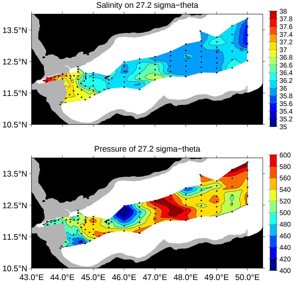
Figure 9: (Top) Horizontal distribution of salinity in the Gulf of Aden at the main spreading level of Red Sea Water (density layer 27.15 < \sigma_\theta < 27.25 ). (Bottom) Same as top, but showing the mean pressure in dbar of that layer.
