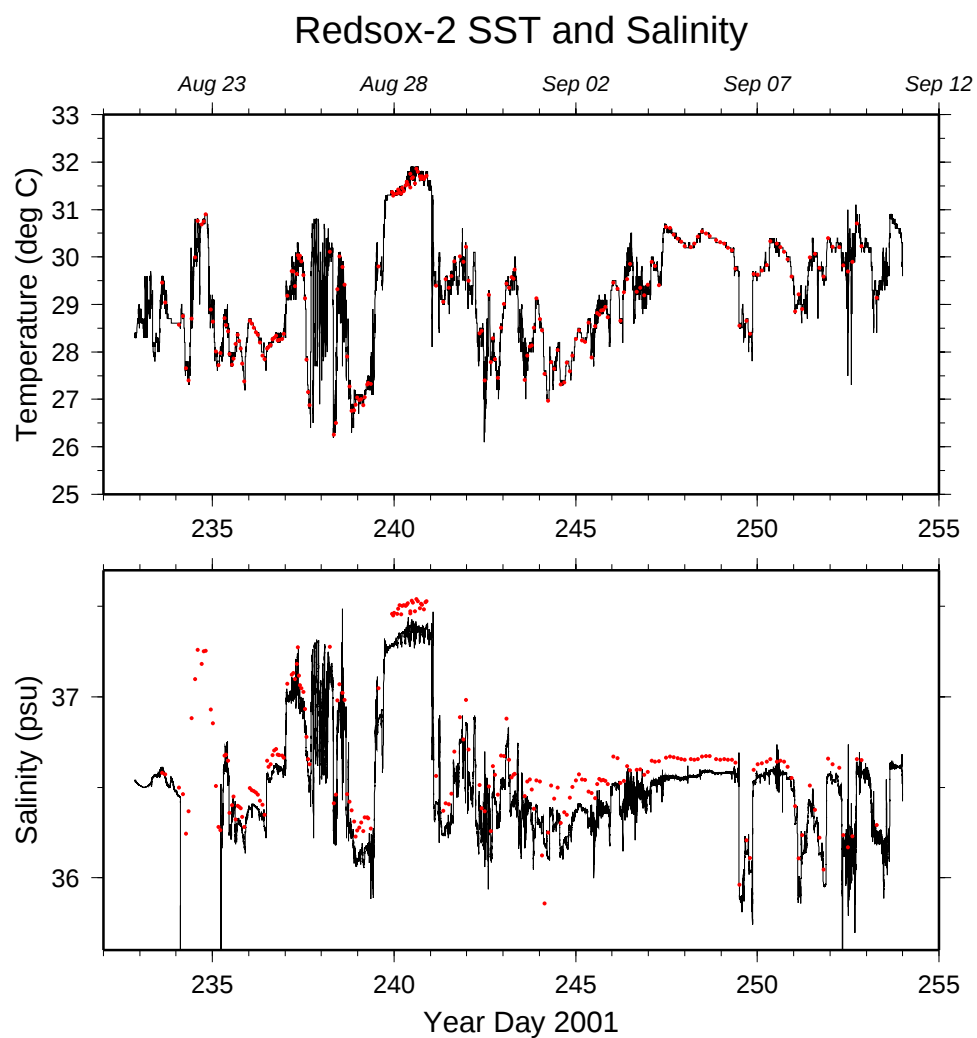
Figure 6: Sea surface temperature (top) and salinity (bottom) as recorded by the thermosalinograph on the R/V Maurice Ewing during REDSOX-2. Near-surface CTD data (dots) indicate a mean offset of the thermosalinograph salinity of -0.12 psu.
