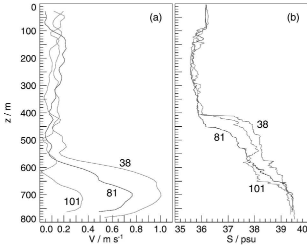
FIG. 9. Variations of (a) velocity magnitude and (b) salinity near the lower end of the Northern Channel, REDSOX-1. The locations of casts 38, 81, and 101 are depicted in Fig. 1a.
