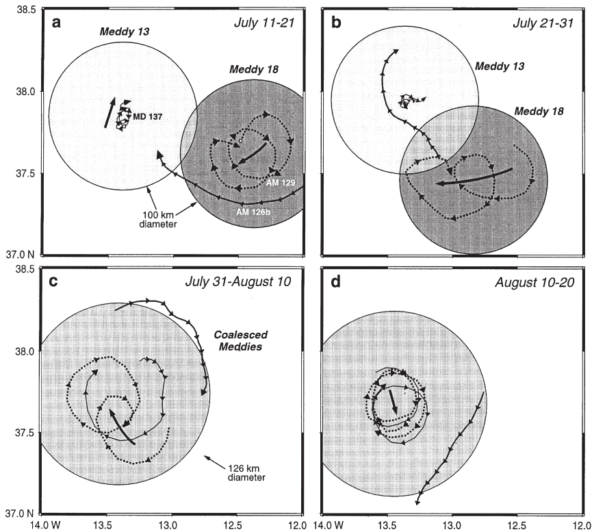
Fig. 7. Coalescence of Meddies 13 and 18 as shown by the trajectories of floats MD137 in Meddy 13 and, AM129, and AM126b in Meddy 18 (near depths of 930, 1170 and 1160 m respectively). Circles have been added to illustrate the approximate overall size of the Meddies. During July 11–21, 1994, the Meddies began to coalesce as Meddy 18 approached from the east toward a nearly stationary Meddy 13. During July 21–31 the central region of Meddy 18 (float AM129) began to turn northward. At this time the trajectory of float AM126b showed the connection between Meddies. During July 31–August 10 the Meddies completely coalesced as shown by all three floats which began looping around a common center. Further evidence is provided by another float, MD136, at 1120 m which was launched along with MD137 in Meddy 13 and remained in it and the merged Meddy until December 1994. The trajectory and temperature series of MD136 are not shown because they are very gappy and the loops were not resolved. The data are consistent with the coalescence of two Meddies.
