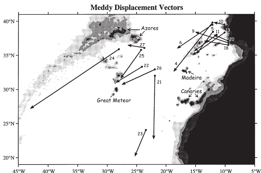
Fig. 13. Overall displacement vectors for 16 Meddies continuously tracked for at least 100 days. Depth contours (1000 and 2000 m) show the Horseshoe Seamounts, the Great Meteor Seamounts and the mid-Atlantic Ridge. The displacements of Canary Basin Meddies 22, 25, 26 all stop where their floats ceased to loop after the Meddies collided with seamounts. Meddy 24 collided with Plato Seamount but continued for at least another 1.2 yr despite significant changes of the Meddy's swirl velocity and temperature during the collision.
