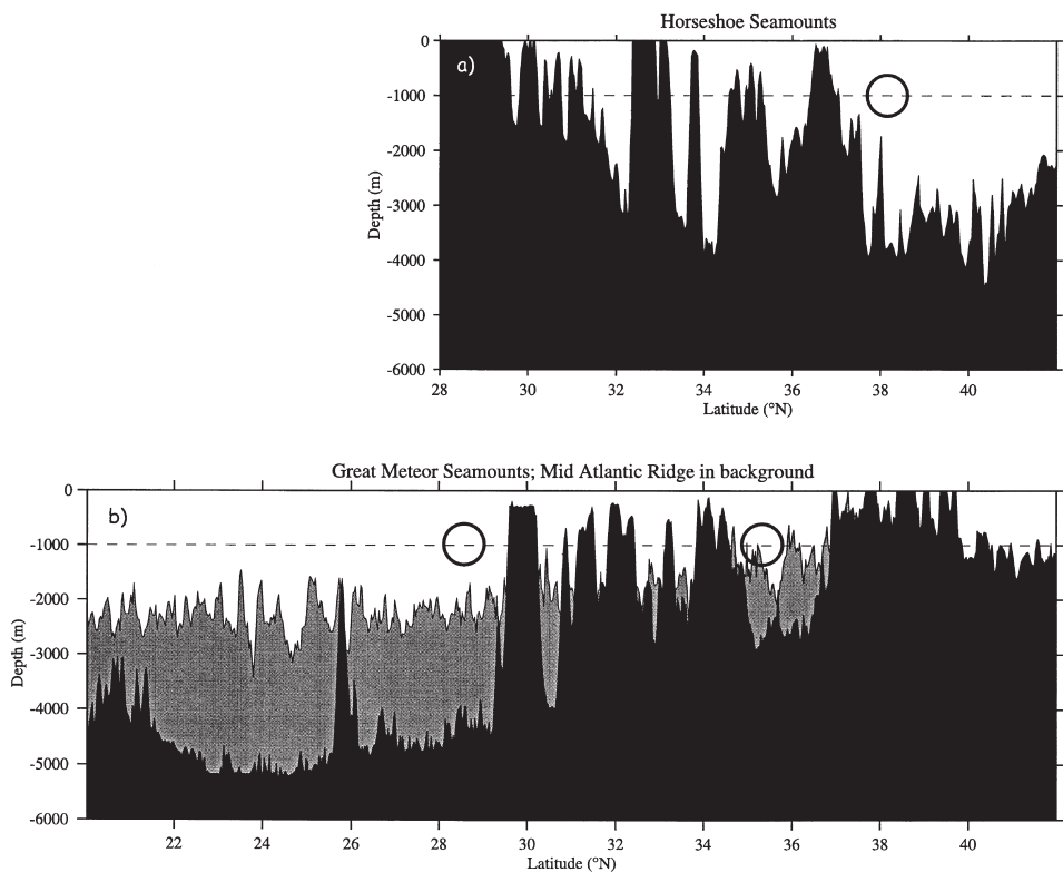
Fig. 9. North-south sea floor depth profiles showing (a) the Horseshoe Seamounts, and (b) the Great Meteor Seamounts and the Azores Plateau (black), and the mid-Atlantic Ridge (grey). The Great Meteor Seamounts are a line of seamounts extending north and a little west of Great Meteor Seamount as shown in detail in later figures. These are major obstacles faced by a Meddy translating westward in the Atlantic. Typical Meddies are shown schematically to be 800 m in vertical extent and 100 km in diameter. The Meddies are shown centered where they could possibly translate westward without colliding with seamounts. Depth profiles were created by plotting the shallowest depth at each latitude using ETOPO2 data (Smith & Sandwell, 1997) in meridional swaths in the Iberian Basin 11°W–17°W (Horseshoe Seamounts), in the Canary Basin 25°W–32°W (Great Meteor Seamounts), and along the mid-Atlantic Ridge 32°W–45°W.
