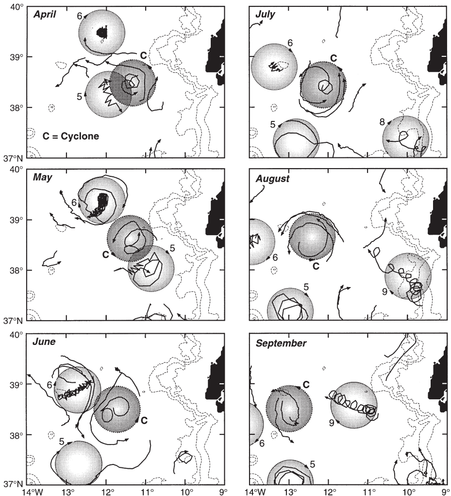
Fig. 11. Time sequence showing month-long segments of all floats in and around a coherent cyclone observed between April and September 1993 southwest of the Tejo Plateau. The Meddies and cyclone are indicated schematically here with circles 100 km in diameter which show the approximate overall size of the eddies. The circles overlap at times (April–June) which implies that the eddies were probably connected and interacting.
