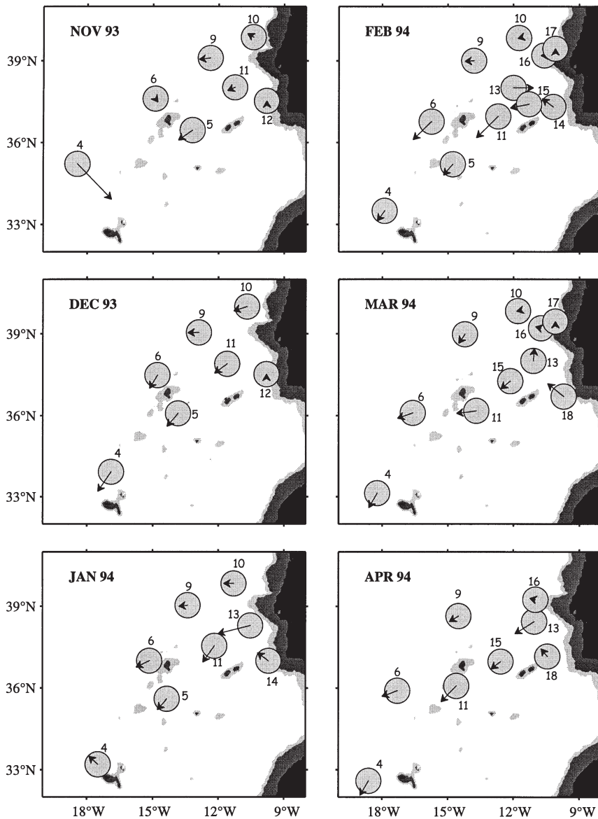
Fig. 18. Sequence of Meddies observed by looping floats in the Iberian Basin November 1993–April 1994. Meddies are indicated schematically by 100 km diameter circles. Some Meddies such as 12, 14, and 17 near the eastern boundary were probably smaller than 100 km as implied by the circles which overlap the 1000 m depth contour (see Appendix A for diameter). The velocity of each Meddy between positions one month apart is shown by vectors. Fig. 17 is an expanded area version of the February 1994 subplot.
