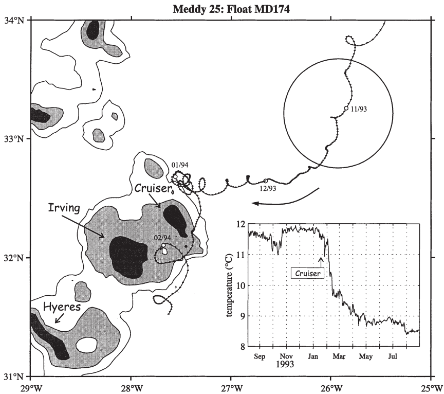
Fig. 15. Trajectory and temperature of float MD174 in Meddy 25 as it translated over Cruiser Seamount on January 26, 1994, and made a close pass to Irving Seamount. Float MD174 stopped looping on February 13, 1994. The trajectory is terminated in the figure where the loops stop. A second float (MD172) in Meddy 25 with a similar trajectory stopped looping on February 6. The main decrease in temperature of these two floats at depths of 1000–1050 m was over a three week period, January 26–February 15, although the temperature of float MD174 continued to decrease at least through March as the float remained in the same general area and depth but did not loop. The total decrease in temperature was around 3°C. The overall diameter of Meddy 25 measured hydrographically before the collision was around 100 km as shown by the circle.
