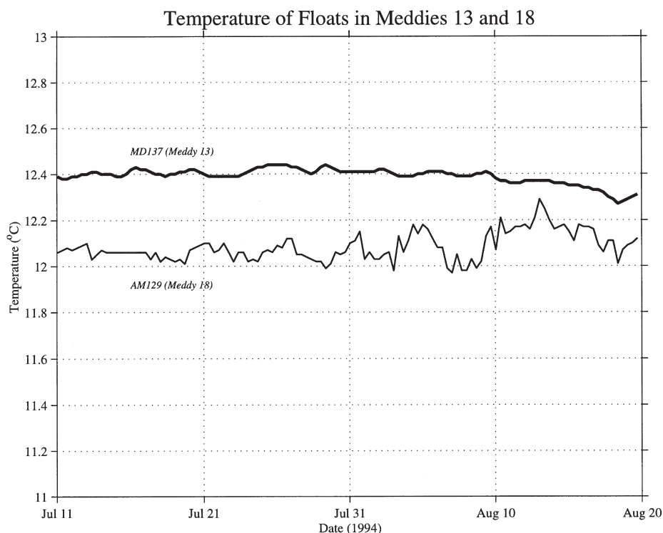
Fig. 8. Temperature measured by floats MD137 at a depth of 930 m and AM129 at 1170 m during the coalescence of Meddies 13 and 18. Temperature remained greater than 12°C throughout the coalescence, and in the case of MD137, did not drop significantly until the composite Meddy collided (possibly fatally) with Lion Seamount. Float MD137 was warmer and shallower than float AM129 and closer to the warmer, less saline upper core water originating in the Mediterranean Undercurrent. The temperature of float MD136 at a depth of 1120 m was around 12.2 during the coalescence but gappy and therefore not shown.
