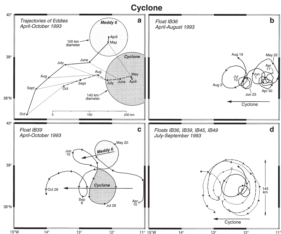
Fig. 12. Detailed observations of a large cyclonic eddy. (a) Monthly positions of Meddy 6 and the cyclone based on looping float trajectories. The circles added to the April positions indicate the eddies' overall size. Meddy 6 translated counterclockwise relative to the cyclone and was possibly advected by it. (b) Trajectory of float IB36 as it looped in the cyclone from April 11 to August 19, 1993. (c) Trajectory of IB39 from April 10 to October 31, 1993, as it looped alternately in the Meddy and cyclone. One loop in each eddy was shaded to differentiate them. (d) Four floats (IB36, IB39, IB45, IB49) looped in the cyclone during July to September 1993.
