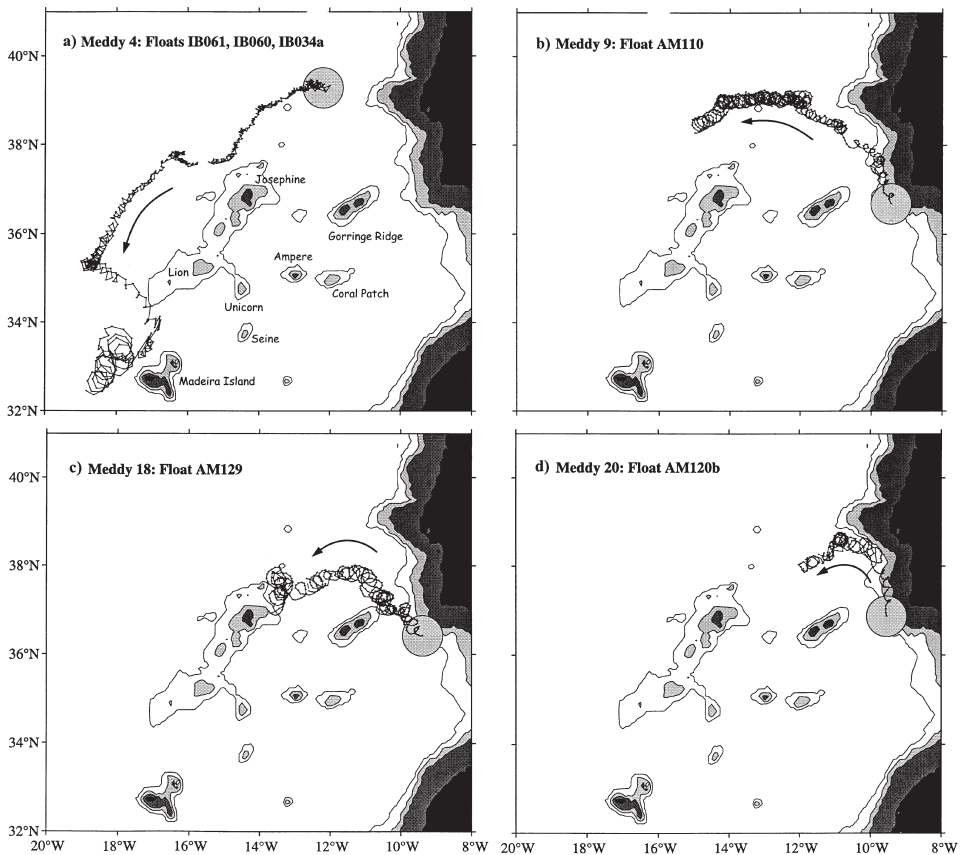
Fig. 4. Trajectories of four representative Meddies in the Iberian Basin. A circle of diameter 100 km was added to each Meddy to show its approximate overall size. Meddies formed near Cape St Vincent are probably smaller than this and do not overlap the topography as it appears in the figure. In all panels, the coastline and 1000, 2000 and 3000 m isobaths are indicated. (a) Three floats (IB61, IB60, IB34) pieced together to show the overall trajectory of Meddy 4 (see Appendix A) from September 23, 1992, to April 21, 1994. This is the longest tracked (1000 km, 1.6 yr) of the Iberian Basin Meddies. Meddy 4 was surveyed three times by ship in September 1992, March and July 1993 and seeded with floats each time. Many float loops were around 10 km in diameter, much smaller than the Meddy's overall diameter of around 80 km. Larger diameter loops up to 70 km appeared after Meddy 4 interacted with the Azores Current and brushed past (at a distance of ~40 km) Madeira Islands in mid January 1994. (b) Trajectory of float AM110 which looped in Meddy 9 for 328 days, starting at its formation near Cape St Vincent on July 20, 1993 and continuing until the float surfaced on June 13, 1994. Of the six Meddies observed to form at Cape St Vincent, this one drifted the farthest north before turning toward the southwest and drifting around the Horseshoe Seamounts. (c) Track of AM129, which looped in Meddy 18 from March 3, 1994 to September 16, 1994. The loops of float AM126b suggest that this Meddy's overall diameter was greater than 90 km. In July and early August Meddy 18 coalesced with Meddy 13, then collided with several seamounts in the Horseshoe chain. (d) Meddy 20, as revealed by float AM120b, translated rapidly (17 cm/s) northward along the eastern boundary before turning westward away from the slope and into deeper water. This Meddy was tracked from October 14, 1994 to January 31, 1995.
