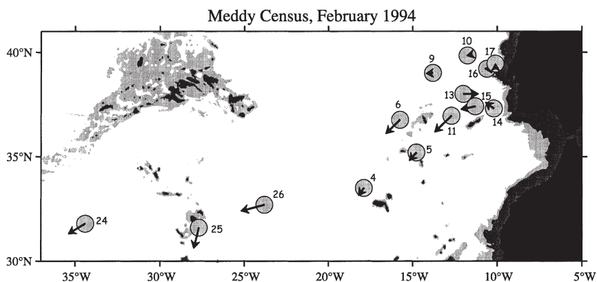
Fig. 17. A census of Meddies in February 1994, the month with the most observed Meddies. Fourteen Meddies were tracked, eleven east of 18°W and three in the Canary Basin, 23°W–35°W, with at least one float looping in each Meddy. Vectors show the translation of Meddies between February and March 1994. Circles with a diameter of 100 km show the location and typical overall size of the Meddies. Some Meddies could be smaller than 100 km and others larger. Our interpretation is that two different Meddies coexisted where 16 and 17 are shown, and that at least Meddy 17 was much smaller than the schematic 100 km diameter.
