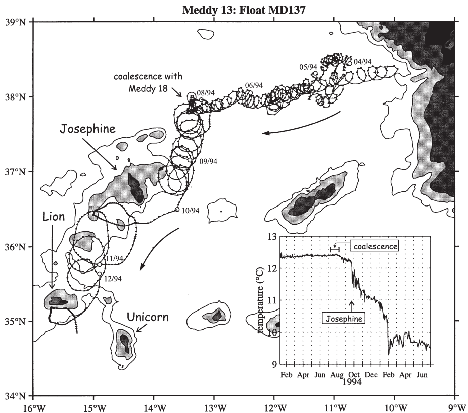
Fig. 10. Trajectory of float MD137 in Meddy 13 from January 1 to December 25, 1994. Meddy 13 was discovered by Pingree (1995) near 38.4°N 10.0°W adjacent to the continental slope near Lisbon Canyon and had presumably just formed. Pingree launched two surface drifters, two ALACE floats and two RAFOS floats into this Meddy. In July and early August Meddy 13 collided and coalesced with Meddy 18 (see Fig. 7). In September and October 1994 Meddy 13 skirted around the southeastern side of Josephine Seamount (<200 m depth) and then translated over or near two other seamounts southwest of Josephine (one <800 m depth and the other <1600 m depth). In December Meddy 13 passed over or around Lion Seamount (<600 m). The loops of float MD137 increased in diameter from 10 to 40 km during the coalescence with Meddy 18 and to 50 km after colliding with Josephine Seamount. Both floats MD136 and MD137 stopped looping in December 1994 after passing over or around Lion. The cessation of looping after the final collision implies that Meddy 13 was severely disrupted if not totally destroyed by its collisions with the Horseshoe Seamounts. The inset shows temperature time series measured by float MD137 near a depth of 930 m in Meddy 13. On September 20, 1994, as Meddy 13 collided with Josephine Seamount the temperature dropped from 12.1 to 11.6°C. From September 20 into January 1995 as Meddy 13 passed over several seamounts the temperature gradually decreased to 10.5°C accompanied by temperature fluctuations up to 0.5°C. During this time the float was looping at a diameter of 50–80 km. Float MD137 stopped looping on December 25, 1994, just after passing over Lion Seamount. Afterward (not shown) float MD137 slowly translated south to around 31°N. At the end of January the temperature dropped to 9.4°C and then stabilized near 9.7°C. The cooling after December 25 occurred after the float stopped looping, possibly indicating the mixing of a Meddy remnant with the background fluid.
