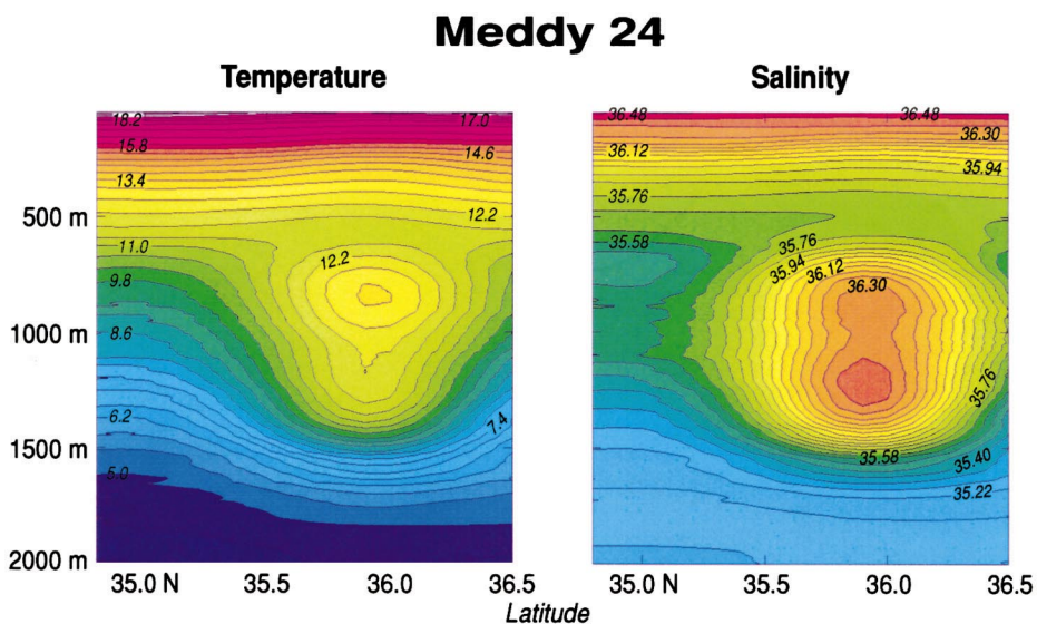
Fig. 1. Vertical sections of temperature and salinity through Meddy 24 in the Canary Basin near 36°N 28°W measured during July 1993 (Tychensky & Carton, 1998). Meddy 24 contained double maxima in the vertical of both temperature and salinity. Values reached 13.2°C and 36.4 psu at 850 m and 12.3°C and 36.5 psu at 1250 m. Maximum anomalies compared to background values were 4.1°C and 1.1 psu at 1250 m. The overall diameter of Meddy 24 was around 120 km. Repeated sections through a Meddy during two years have been shown by Armi et al. (1989) and Hebert et al. (1990), see also Schultz Tokos et al. (1994).
