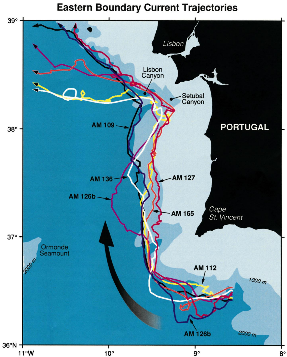
Fig. 5. Trajectories of seven floats deployed in the Mediterranean Undercurrent south of Portugal that followed the continental slope around Cape St Vincent and northward to the Tejo Plateau. These floats clearly indicate the presence of a well-defined boundary current that could advect newly formed Meddies northward. The mean depth of these seven floats is 1123 m.
