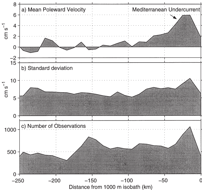
Fig. 6. (a) Mean poleward along-boundary velocity within 250 km of the 1000 m isobath based on all float data except those clearly in the cores of Meddies and those east of 9.25°W in the Gulf of Cadiz. Individual float velocities were grouped and averaged in 10 km wide bins parallel to the 1000 m depth contour which was obtained from ETOPO2 data. A poleward flowing eastern boundary current, the Mediterranean Undercurrent, has a peak mean speed of about 6 cm/s, and occupies the nearest 100 km to the slope. (b) Standard deviation in the 10 km wide bins, and (c) number of observations in each bin.
