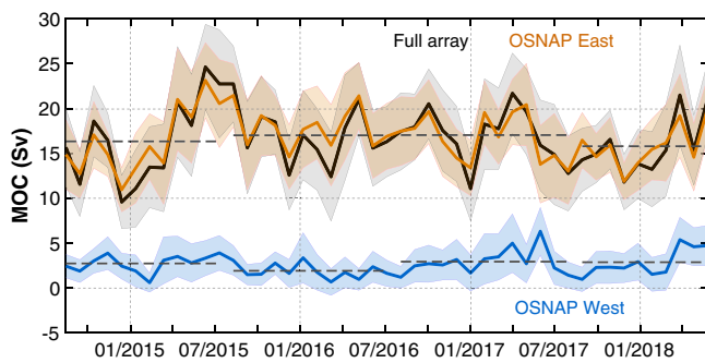
Fig. 2 Subpolar Meridional Overturning Circulation (MOC) time series. 30-day MOC estimates across the full array, OSNAP West and East, respectively. Shading indicates uncertainty in the 30-day estimate, obtained from a Monte Carlo method 10 . Horizontal dashed lines indicate the 12-month averages (10-month for 2017–2018). The total Ekman transport (not shown) is -0.7 \pm 0.01 \text{ Sv} during the whole time period.
