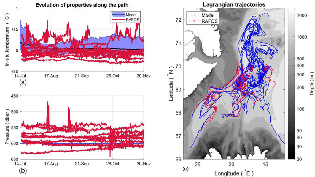
FIG. 4. Evolution of (a) in situ temperature and (b) pressure of model Lagrangian particles and RAFOS floats. The blue shade shows the 5th and 95th percentile ranges of the particle temperatures. The solid black line shows the mean particle temperature. The red lines show the RAFOS float time series. All the modeled particles are confined to 600 m depth [the blue line in (b)]. (c) Lagrangian trajectories of the model particles (blue) and the RAFOS floats (red). Only 50 model trajectories are shown.
