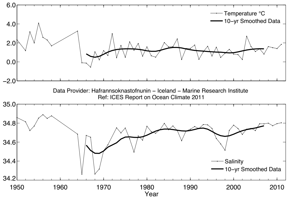
Figure 35. Area 3 – Icelandic waters. Temperature (upper panel) and salinity (lower panel) at 0–50 m in the East Icelandic Current (Langanes Stations 2–6).
