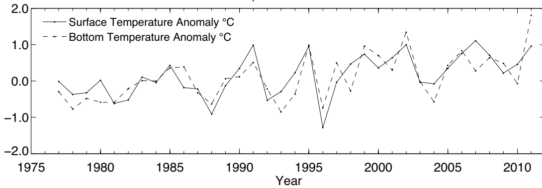
Figure 26. Area 2c – Mid-Atlantic Bight. Surface and bottom temperature anomalies in the central Mid-Atlantic Bight (relative to the base period of 1980–2010) from XBT measurements; the origin of the line is New York City. The data represent the average conditions at the surface and bottom inshore of the 100 m isobath.
