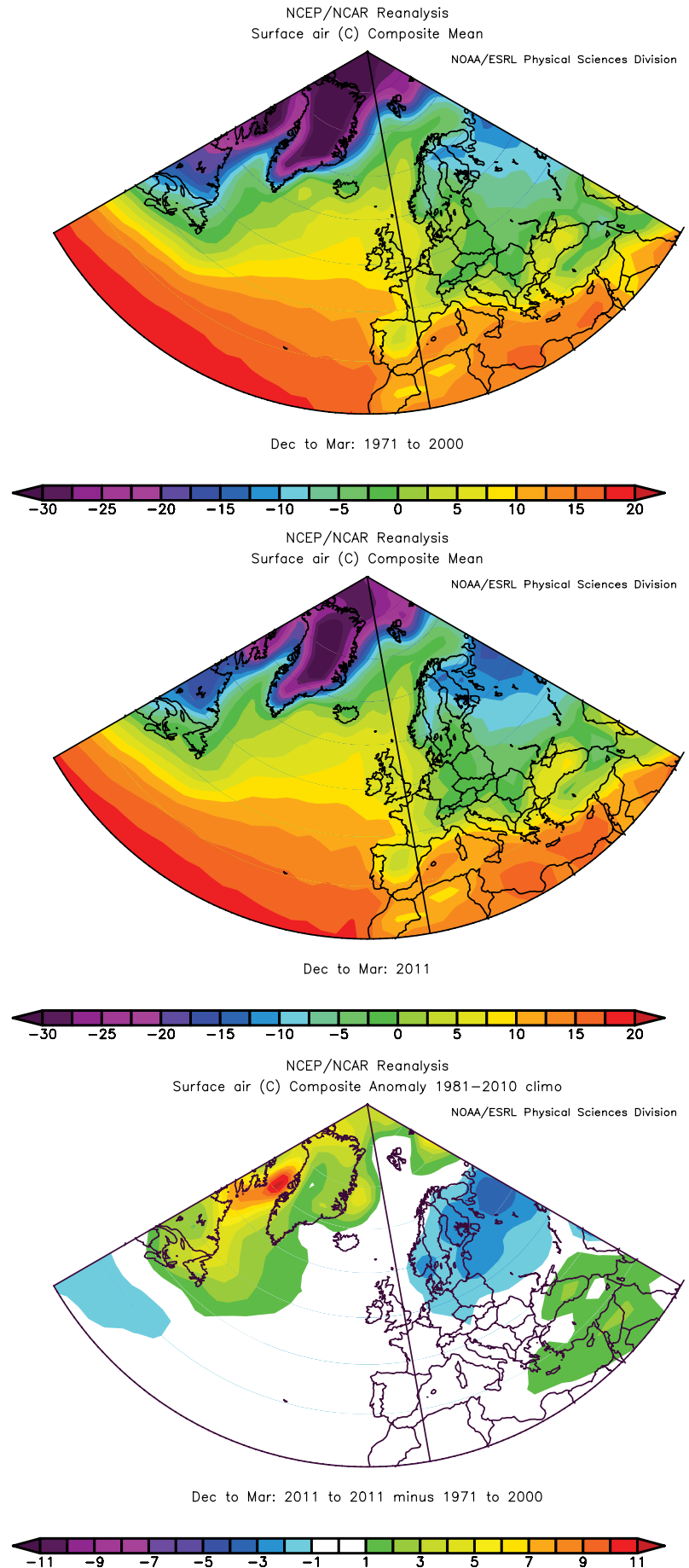
Figure 12. Winter (DJFM) surface air temperature fields. Top panel: surface air temperature averaged over 30 years (1971–2000). Middle panel: temperatures in winter 2011 (December 2010, January to March 2011). Bottom panel: winter 2011 surface air temperature anomaly – the difference between the top and middle panels. Images provided by the NOAA/ESRL Physical Sciences Division, Boulder, CO (available online at http://www.cdc.noaa.gov/ ).
