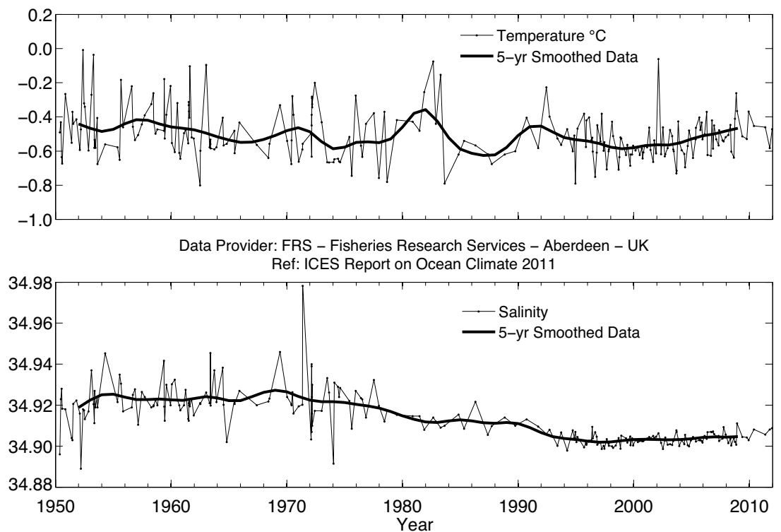
Figure 78. Area 7 – Faroe–Shetland Channel. Temperature (upper panel) and salinity (lower panel) at 800 m.
