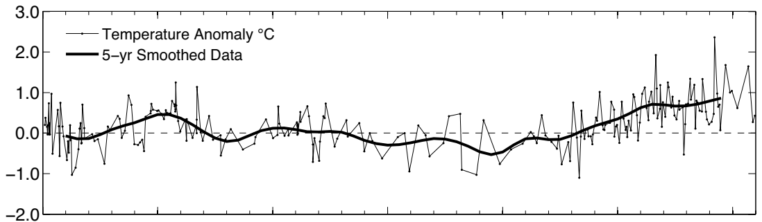
Figure 51. Areas 6 and 7 – Faroe-Shetland Channel. Temperature anomaly (upper panel) and salinity anomaly (lower panel) in the Modified Atlantic Water entering the Faroe-Shetland Channel from the north after circulating around the Faroes.
