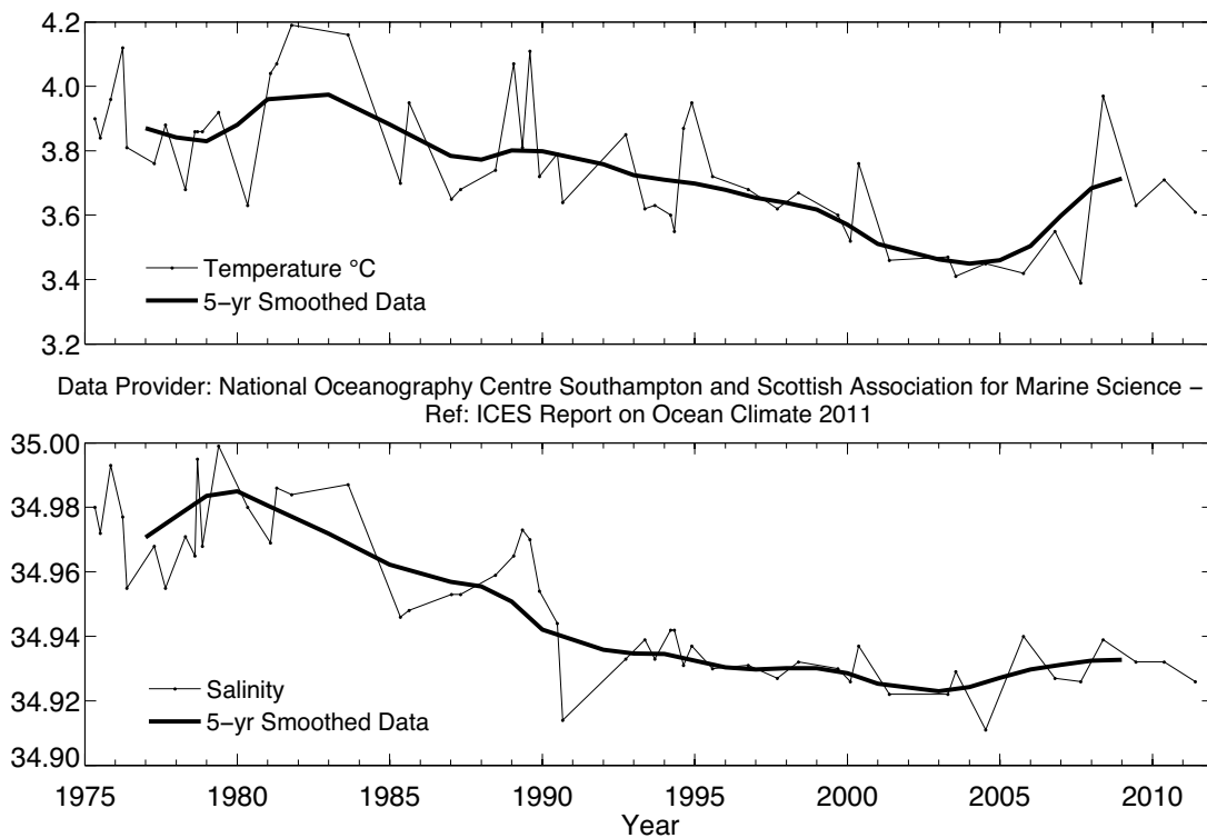
Figure 83. Area 5 – Rockall Trough. Temperature (upper panel) and salinity (lower panel) of Labrador Sea Water (averaged over 1800–2000 m).
