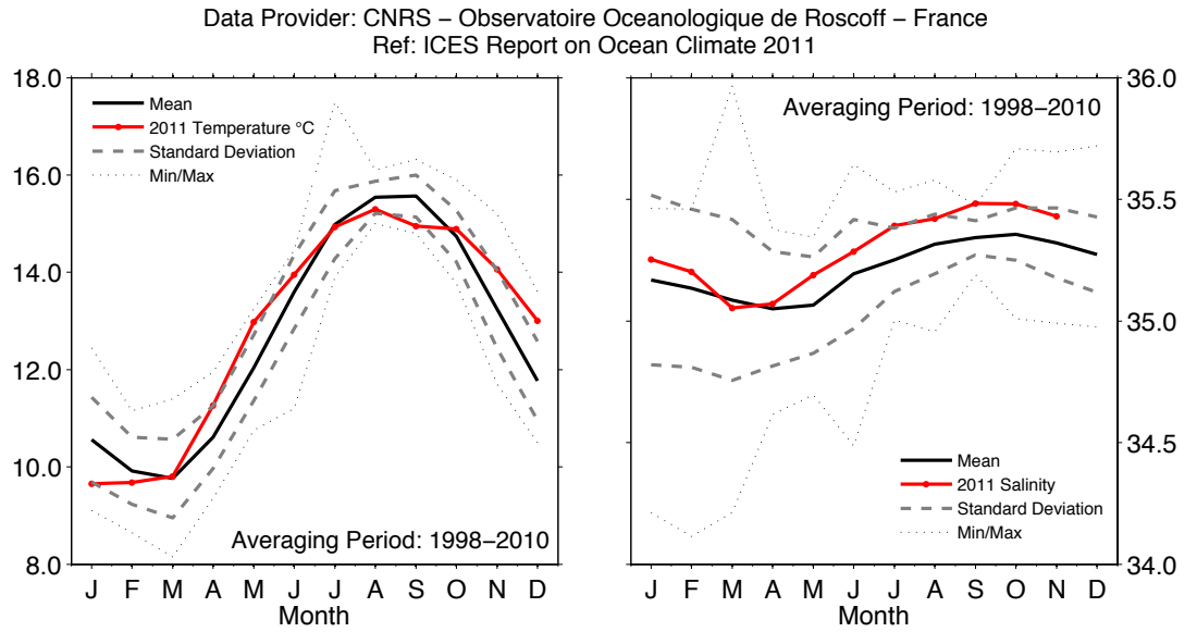
Figure 40. Area 4b – Northwest European continental shelf. 2011 monthly temperature (left panel) and salinity (right panel) of surface water at the Astan station (48.77°N 3.94°W).
