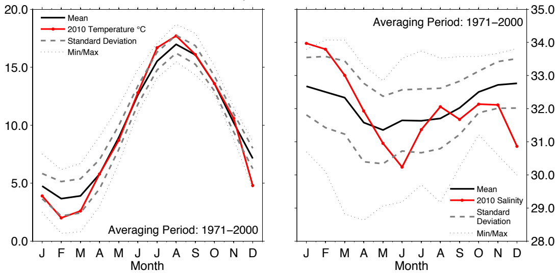
Figure 56. Area 9 – Southern North Sea. 2010 monthly surface temperature (left panel) and salinity (right panel) at Station Helgoland Roads.
