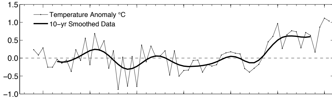
Figure 66. Area 10 – Norwegian Sea. Temperature anomaly (upper panel) and salinity anomaly (lower panel) at 50 m at Ocean Weather Station "M" (66°N 2°E).
