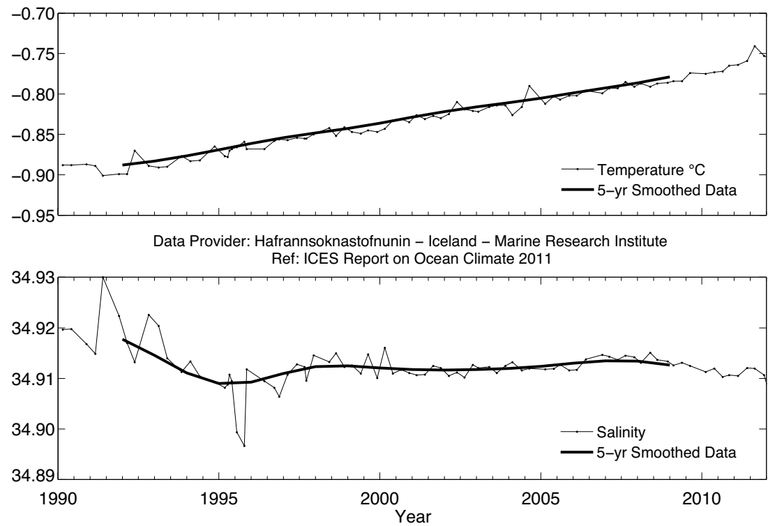
Figure 75. Area 3 – Icelandic waters. Temperature at 1500–1800m in the Iceland Sea (68°N 12.67°W).
