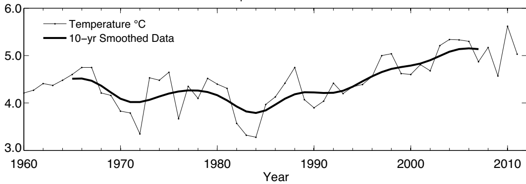
Figure 23. Area 2b – Labrador Sea. Annual mean sea surface temperature data from the west-central Labrador Sea (56.5°N 52.5°W). Data obtained from the HadISST1.1 sea ice and sea surface temperature dataset, UK Meteorological Office, Hadley Centre.
