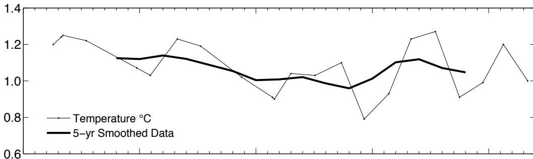
Figure 79. Area 5b – Irminger Sea. Temperature (upper panel) and salinity (lower panel) in Denmark Strait Overflow Water on the East Greenland Slope.
