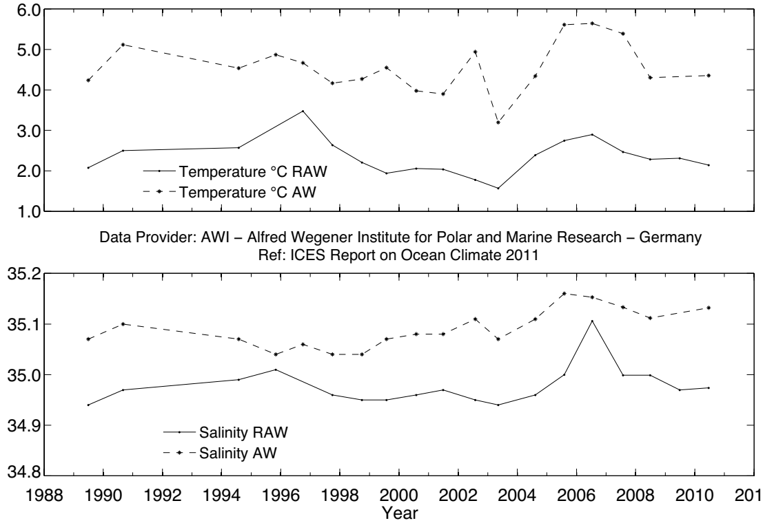
Figure 71. Area 12 – Greenland Sea and Fram Strait. Temperature (upper panel) and salinity (lower panel) of Atlantic Water (AW) and Return Atlantic Water (RAW) in the Greenland Sea Section at 75°N (data to 2010). AW properties are 50–150 m averages at 10–13°E. The RAW is characterized by temperature and salinity maxima below 50 m, averaged over three stations west of 11.5°W.
