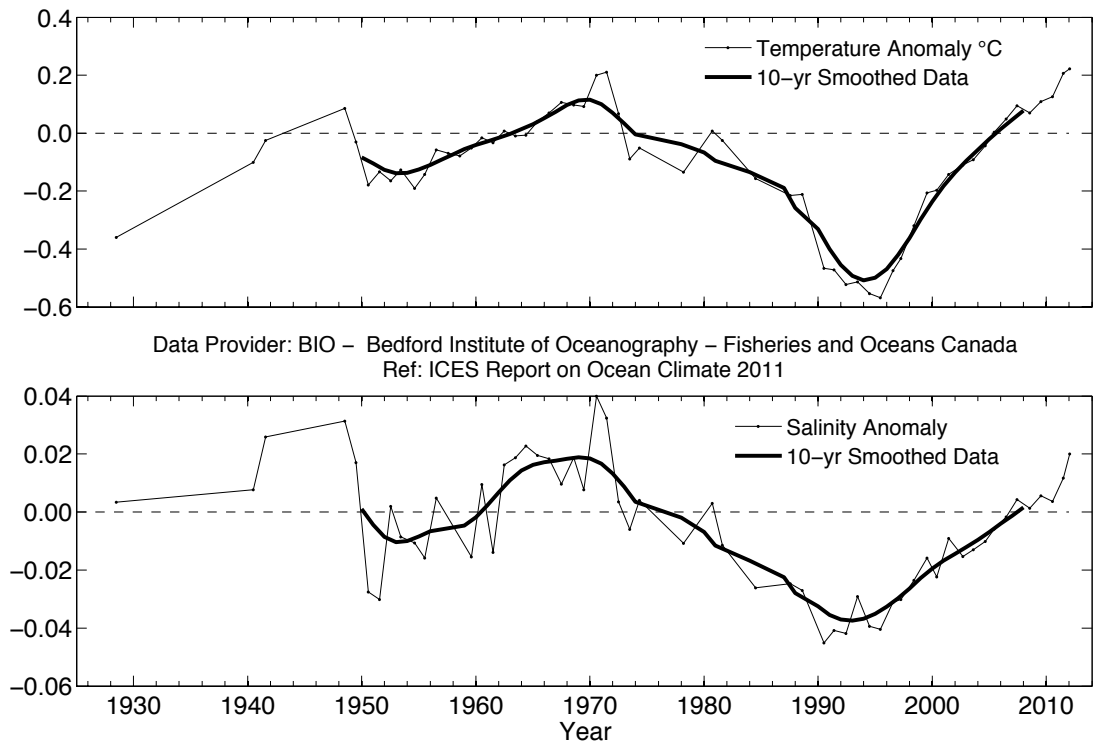
Figure 81. Area 2b – Labrador Sea. Temperature anomaly (upper panel) and salinity anomaly (lower panel) of Labrador Sea Water (averaged over 1000–1800 m).
