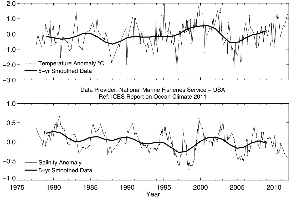
Figure 28. Area 2c – Mid-Atlantic Bight. Time-series plots of 0–30 m averaged temperature anomaly (upper panel) and salinity anomaly (lower panel) on northwest Georges Bank. Anomalies are calculated relative to the period 1980–2010 using hydrographic data from shelf-wide surveys.
