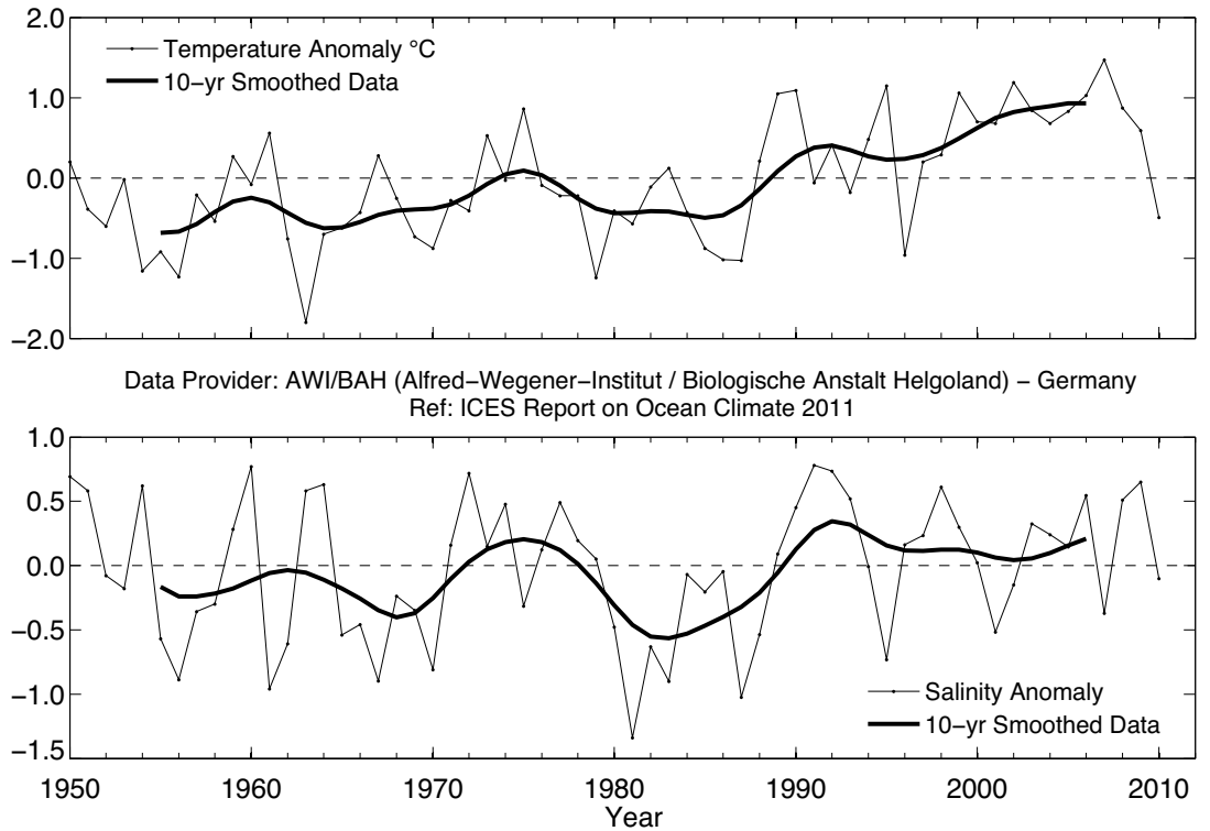
Figure 55. Area 9 – Southern North Sea. Annual mean surface temperature anomaly (upper panel) and salinity anomaly (lower panel) at Station Helgoland Roads.
