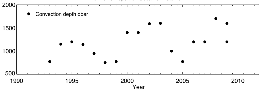
Figure 77. Area 12 – Greenland Sea and Fram Strait. Winter convection depths in the Greenland Sea Section at 75°N (data to 2009; note that due to the unambiguous convection depth in winter 2009/2010 two values are provided for this period).
