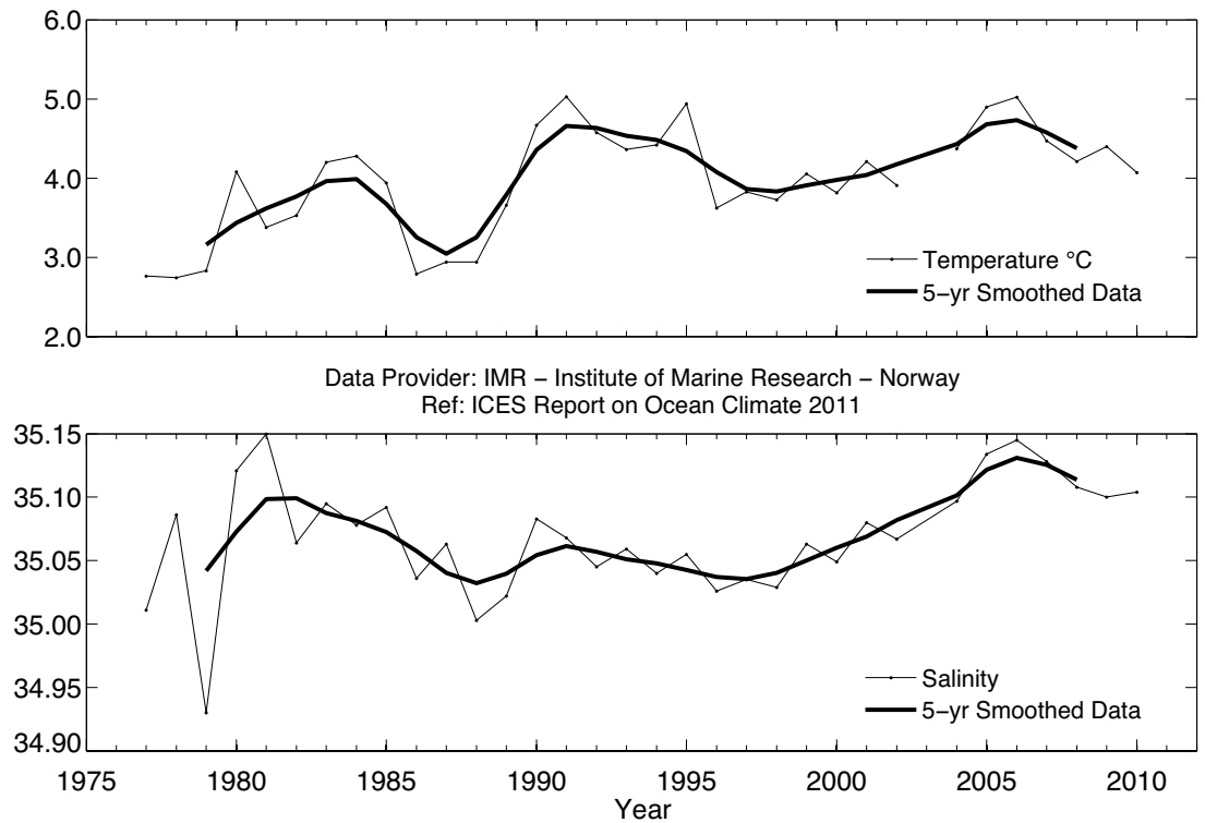
Figure 65. Area 10 – Norwegian Sea. Average temperature (upper panel) and salinity (lower panel) above the slope at Sørkapp Section (76°N, not updated for 2011).
