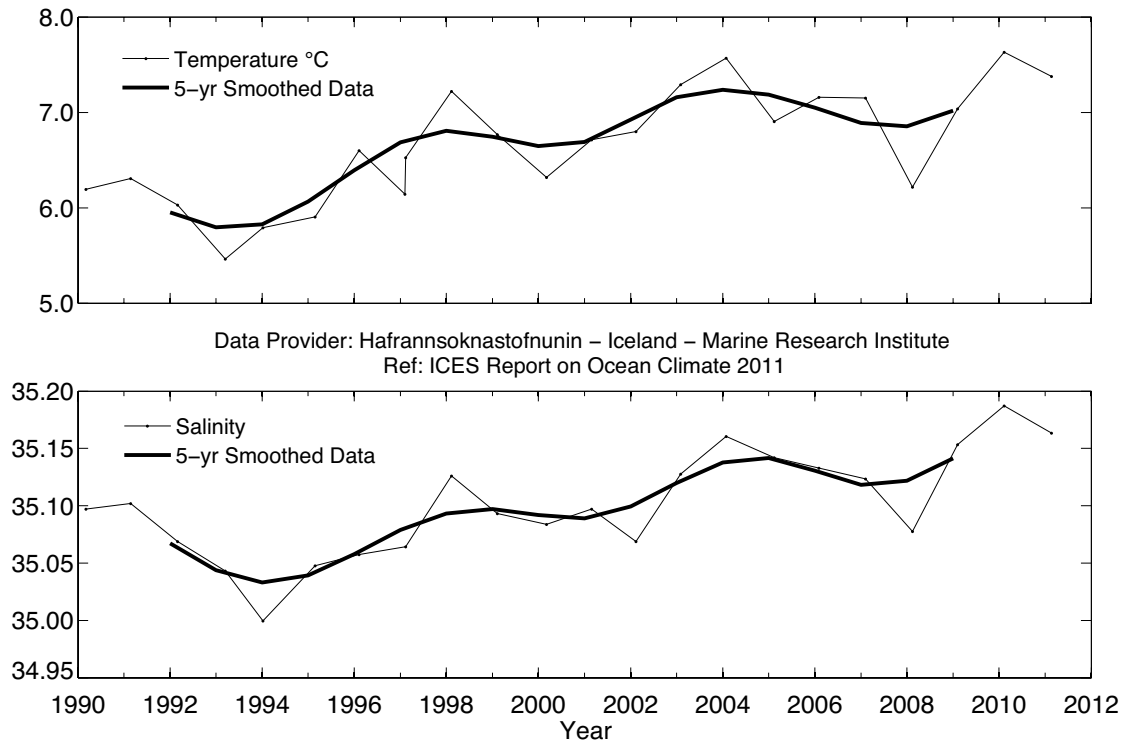
Figure 47. Area 5b – Irminger Sea. Temperature (upper panel) and salinity (lower panel) of Subpolar Mode Water in the northern Irminger Sea (Station FX9, 64.33°N 28°W), averaged over 200–500 m).
