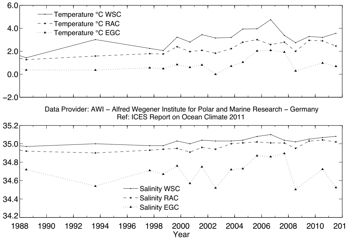
Figure 72. Area 12 – Greenland Sea and Fram Strait. Temperature (upper panel) and salinity (lower panel) in Fram Strait (78.83°N) at 50–500 m: in the West Spitsbergen Current (WSC; between the shelf edge and 5°E), in the Return Atlantic Current (RAC; between 3°W and 5°E), and in the Polar Water in the East Greenland Current (EGC; between 3°W and the Greenland Shelf).
