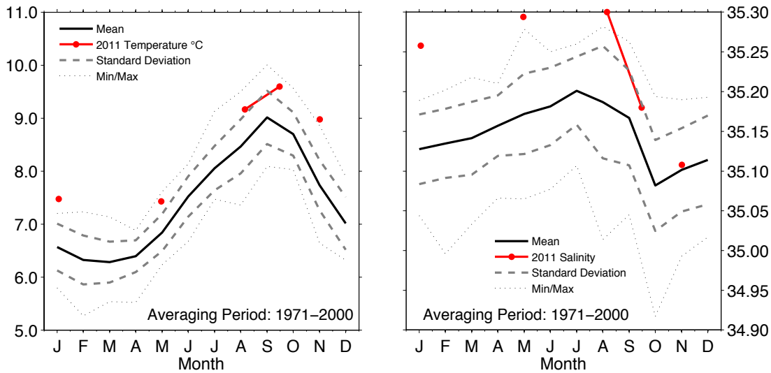
Figure 67. Area 10 – Norwegian Sea. 2011 monthly temperature (left panel) and salinity (right panel) at 50 m at Ocean Weather Station "M" (66°N 2°E).
