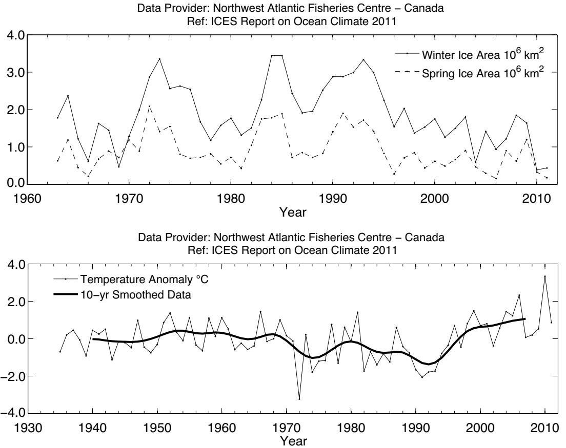
Figure 20. Area 2 – Northwest Atlantic: Newfoundland–Labrador Shelf. Winter and spring sea ice area off Newfoundland–Labrador between 45° and 55°N (upper panel). Annual air temperature anomalies at Cartwright on the Labrador Coast (lower panel).
