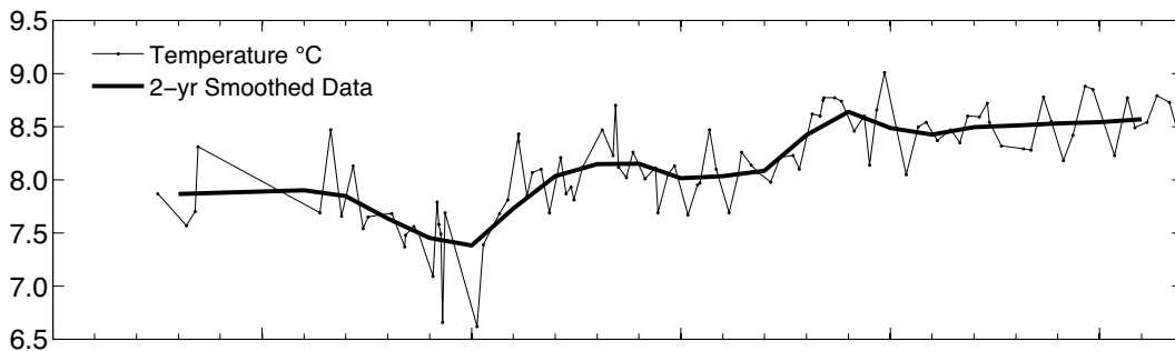
Figure 49. Areas 6 and 7 – Faroe Current. Temperature (upper panel) and salinity (lower panel) in the high salinity core of the Faroe Current north of the Faroes (maximum salinity averaged over a 50 m deep layer).
