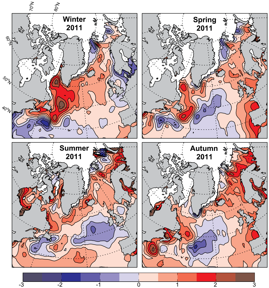
Figure 3. Maps of seasonal sea surface temperature anomalies (°C) over the North Atlantic for 2011 from the NOAA Optimum Interpolation SSTv2 dataset provided by the NOAA–CIRES Climate Diagnostics Center, USA. The colour-coded temperature scale is the same in all panels. The anomaly is calculated with respect to normal conditions for 1971–2000. The data are produced on a 1° grid from a combination of satellite and in situ temperature data. Regions with ice cover >50% of the averaging period are left blank.
