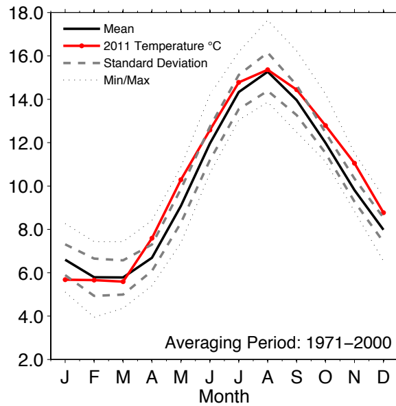
Figure 58. Areas 8 and 9 – Northern and southern North Sea. North Sea area-averaged sea surface temperature (SST) annual cycle; 2011 monthly means based on operational weekly North Sea SST maps.
