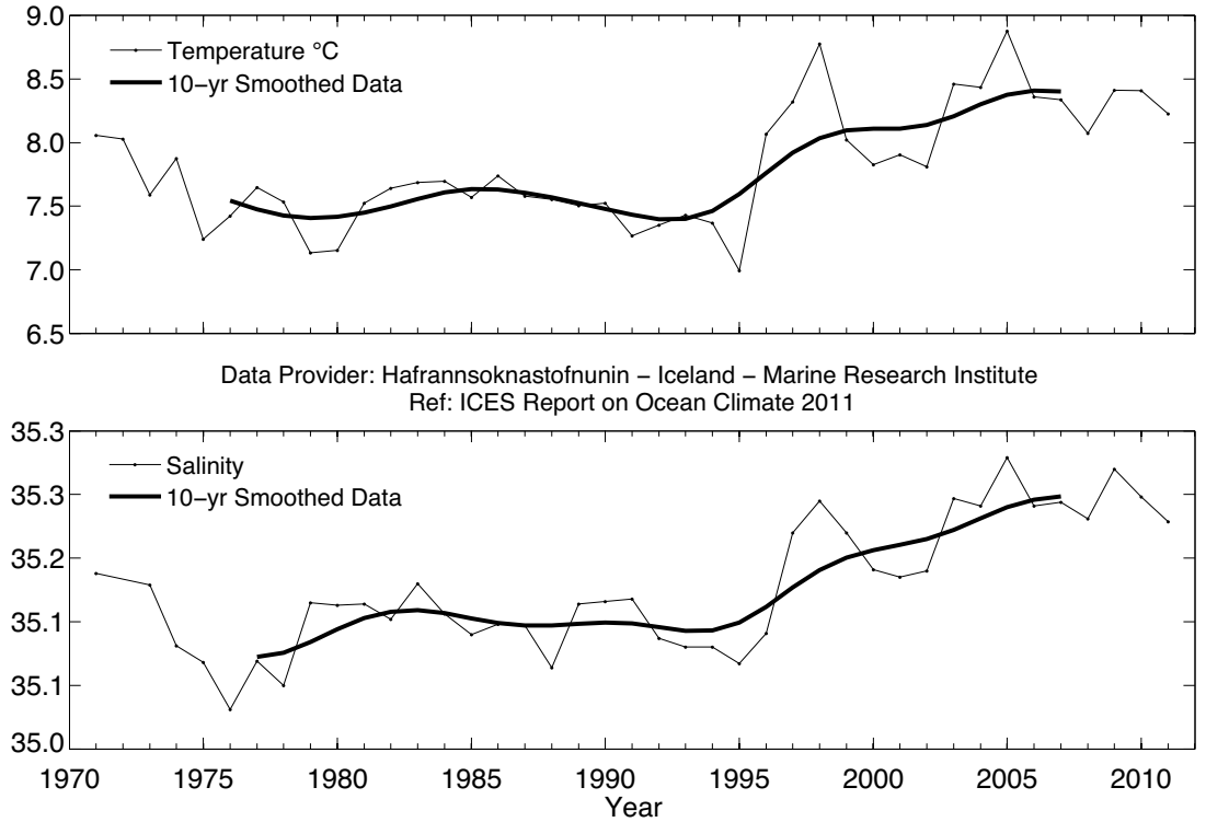
Figure 34. Area 3 – Icelandic waters. Temperature (upper panel) and salinity (lower panel) at 0–200 m at Selvoogsbanki Station 5 in South Icelandic waters.
