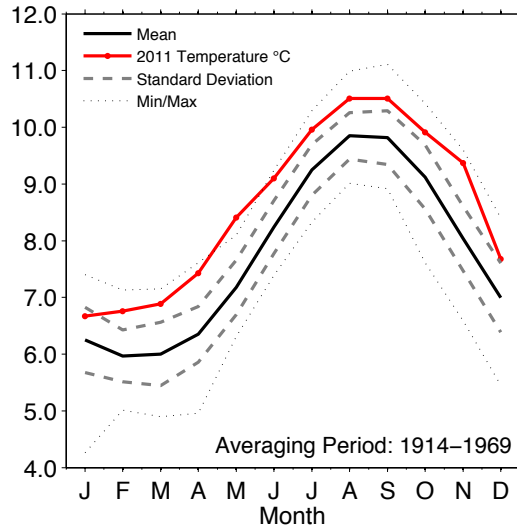
Figure 50. Areas 6 and 7 – Faroe Shelf. 2011 monthly temperature data from the Faroe coastal station at Oyrargjogv (62.12°N 7.17°W). Note the average values were calculated from the nearby station at Mykines (69.10°N 7.66°W).
