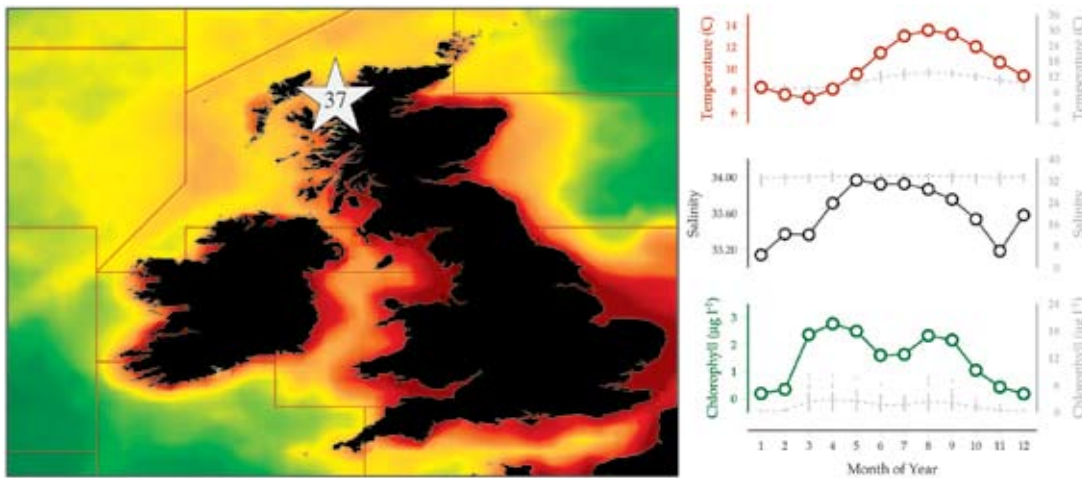
Figure 7.1.1 Location of the Loch Ewe plankton monitoring area (Site 37), plotted on a map of average chlorophyll concentration, and its corresponding environmental summary plot (see Section 2.2.1).
