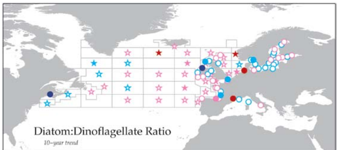
Figure 11.7 Spatio-temporal map of 10-year trends in the diatoms: dinoflagellates ratio present within the CPR standard areas (star symbols) and other monitoring sites (circle symbols). Symbol colors indicate slope (blue/cyan = negative, red/pink = positive) and statistical significance (dark red/blue = p < 0.01 , pink/cyan = p < 0.05 ). Symbols with a white, unfilled, centre indicate slope with a non-significant ( p > 0.05 ) trend.
