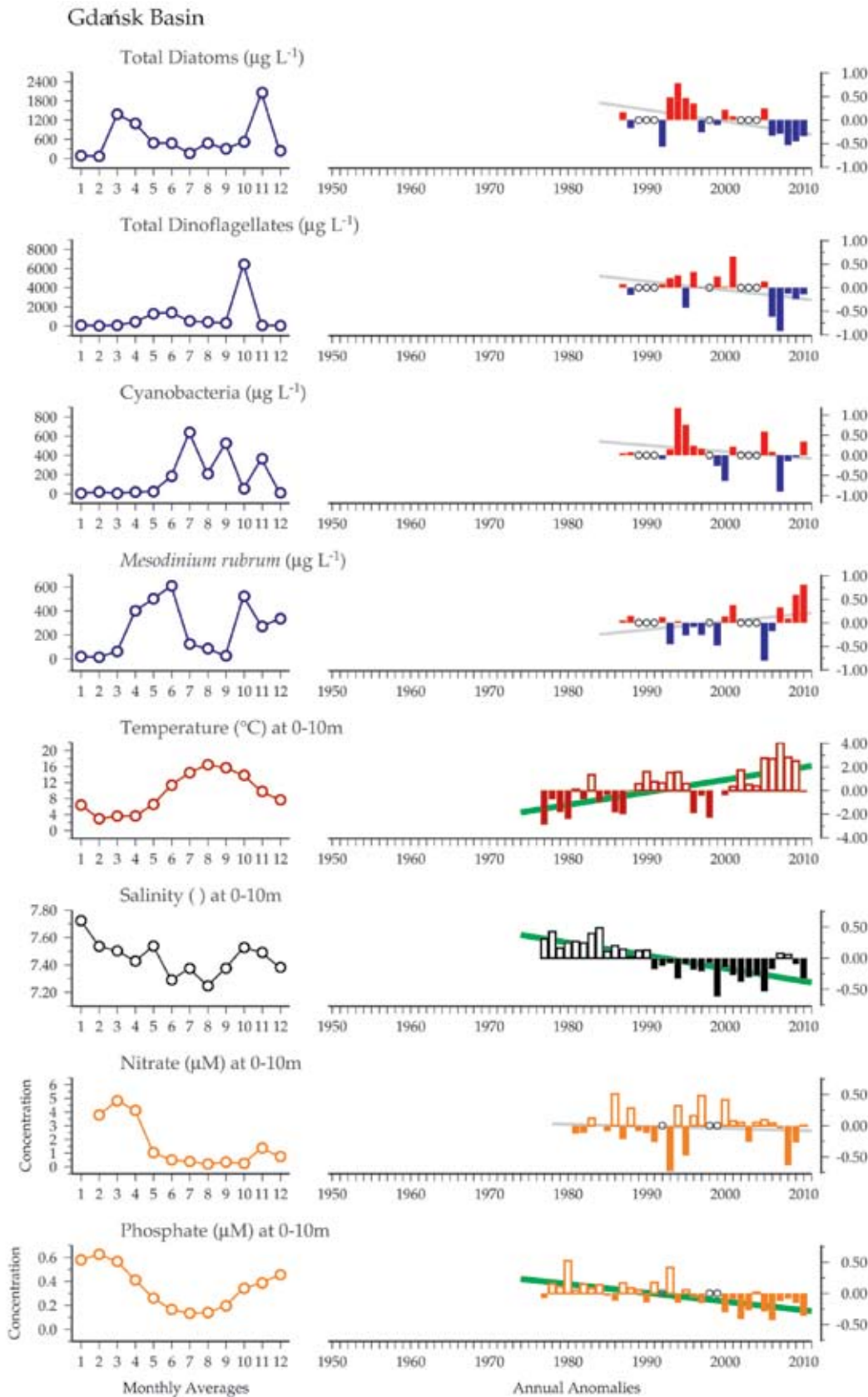
Figure 5.2.2 Multiple-variable comparison plot (see Section 2.2.2) showing the seasonal and interannual properties of select cosampled variables at the Gdańsk Basin plankton monitoring site. Additional variables from this site are available online at http://vgme.net/time-series .
