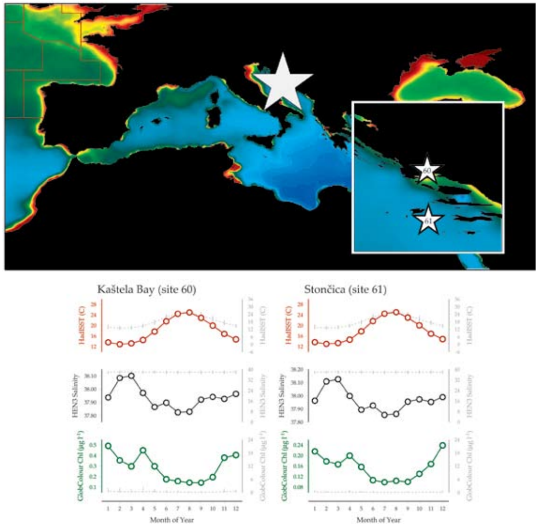
Figure 9.5.1 Locations of the Kaštela Bay and Stončica plankton monitoring areas (Sites 60–61), plotted on a map of average chlorophyll concentration, and their corresponding environmental summary plots (see Section 2.2.1).
