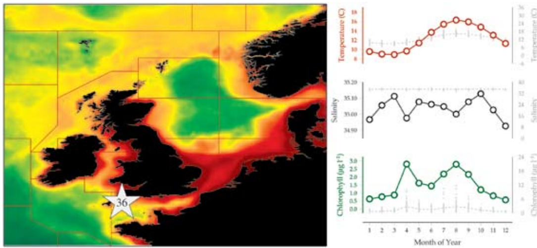
Figure 6.6.1 Location of the Plymouth L4 plankton monitoring area (Site 36), plotted on a map of average chlorophyll concentration, and its corresponding environmental summary plot (see Section 2.2.1).
