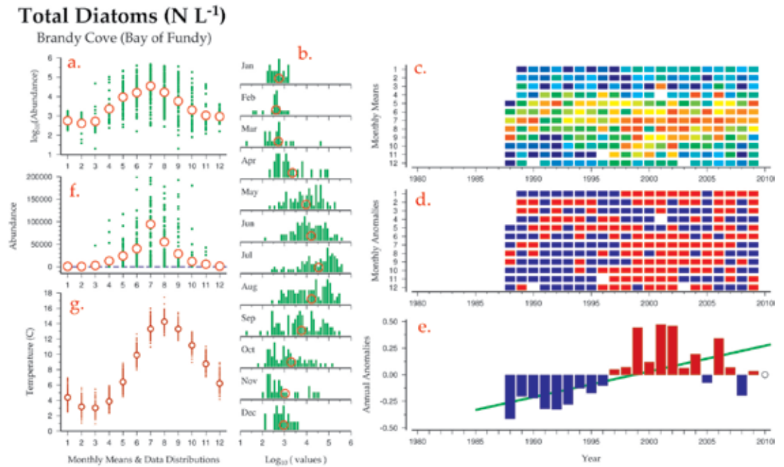
Figure 2.2 A collection of standard WGPME time-series visualization figures illustrating the steps and components used in the WGPME analysis for creating annual anomalies of total diatom abundance from the Brandy Cove time series (Bay of Fundy, Site #2, see Section 3.2 for more information on this site).
