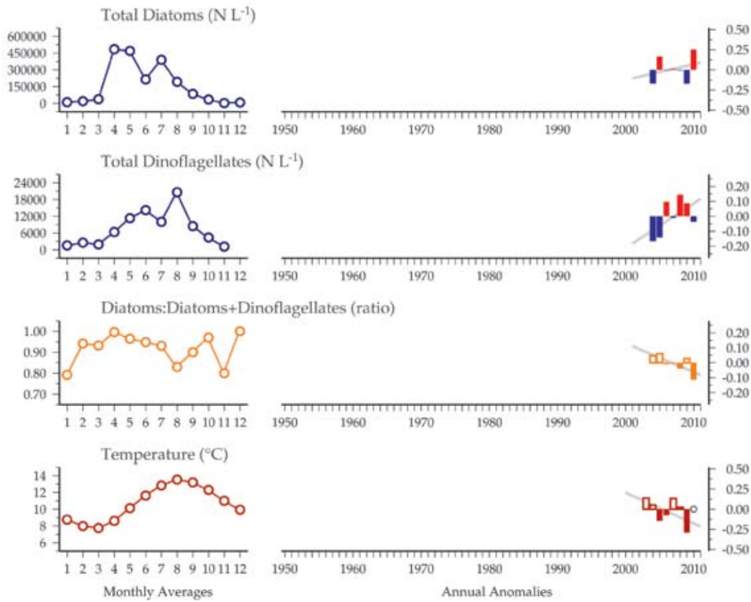
Figure 7.2.2 Multiple-variable comparison plot (see Section 2.2.2) showing the seasonal and interannual properties of select cosampled variables at the Loch Maddy plankton monitoring site. Additional variables from this site are available online at http://wgpme.net/time-series .
