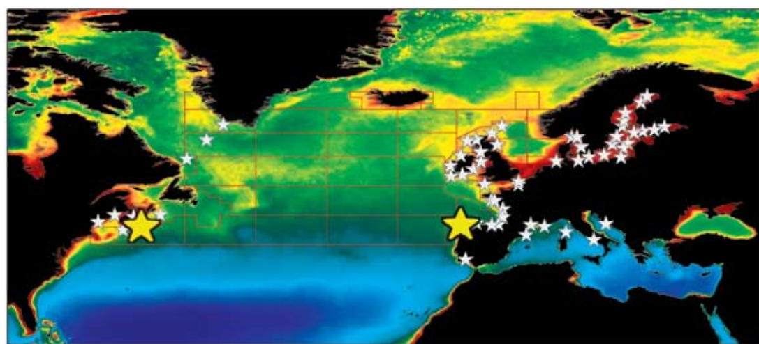
Figure 2.7 Map of GlobColour sea surface chlorophyll concentrations (see Section 2.3.2) overlaid with phytoplankton time-series site locations (white and yellow stars) and CPR standard areas (red boxes). The lower subpanel shows examples of seasonal and interannual properties (see Section 2.2.2) of sea surface chlorophyll concentrations from the Central Scotian Shelf (left yellow star, Site #5, Section 3.4) and RADIALES A Coruña station 2 (right yellow star, Site #53, Section 8.5).
