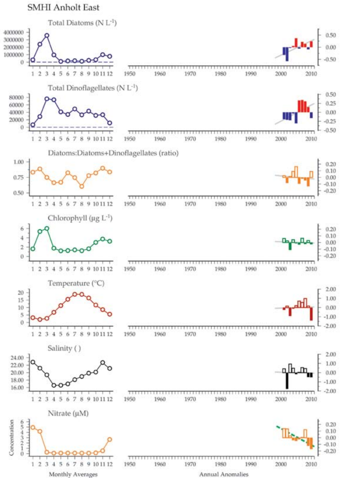
Figure 5.7.2 Multiple-variable comparison plot (see Section 2.2.2) showing the seasonal and interannual properties of select cosampled variables at the Anholt East plankton monitoring site. Additional variables from this site are available online at http://wgpme.net/time-series .
