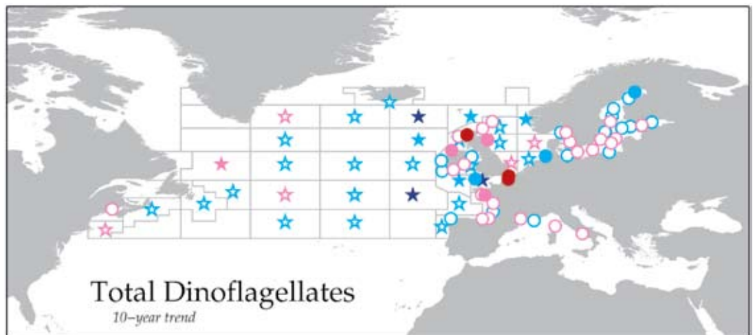
Figure 11.6 Spatio-temporal map of 10-year trends in total dinoflagellate abundance present within the CPR standard areas (star symbols) and other monitoring sites (circle symbols). Symbol colors indicate slope (blue/cyan = negative, red/pink = positive) and statistical significance (dark red/blue = p < 0.01 , pink/cyan = p < 0.05 ). Symbols with a white, unfilled, centre indicate slope with a non-significant ( p > 0.05 ) trend.
