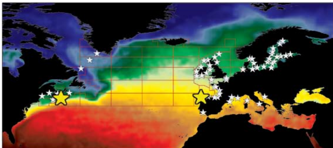
Figure 2.6 Map of HadISST sea surface temperature (see Section 2.3.1) overlaid with phytoplankton time-series site locations (white and yellow stars) and CPR standard areas (red boxes). The lower sub-panel shows examples of seasonal and interannual properties (see Section 2.2.2) of HadISST sea surface temperatures from the Central Scotian Shelf (left yellow star, Site #5, Section 3.4) and RADIALES A Coruña station 2 (right yellow star, Site #53, Section 8.5).
