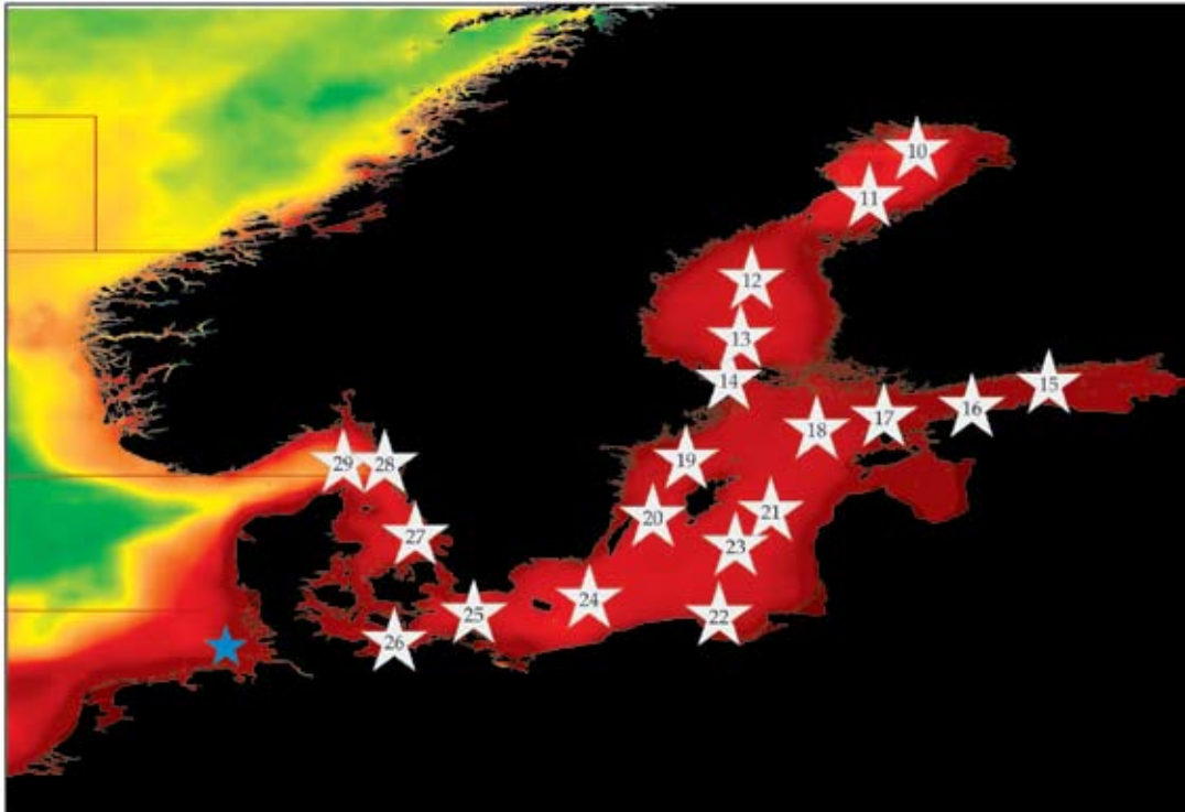
Figure 5.1 Locations of the Baltic Sea plankton monitoring areas (Sites 10–29) plotted on a map of average chlorophyll concentration. Blue stars indicate locations of sites described in the adjacent North Sea and English Channel region (see Section 6).
