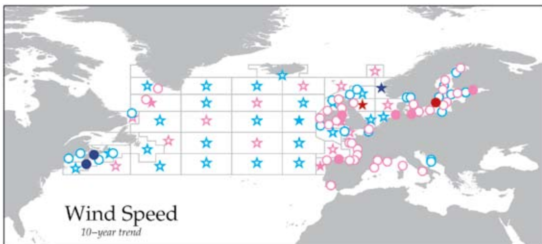
Figure 11.3 Spatio-temporal map of 10-year trends in wind speed present within the CPR standard areas (star symbols) and other monitoring sites (circle symbols). Symbol colors indicate slope (blue/cyan = negative, red/pink = positive) and statistical significance (dark red/blue = p < 0.01 , pink/cyan = p < 0.05 ). Symbols with a white, unfilled, centre indicate slope with a non-significant ( p > 0.05 ) trend.
