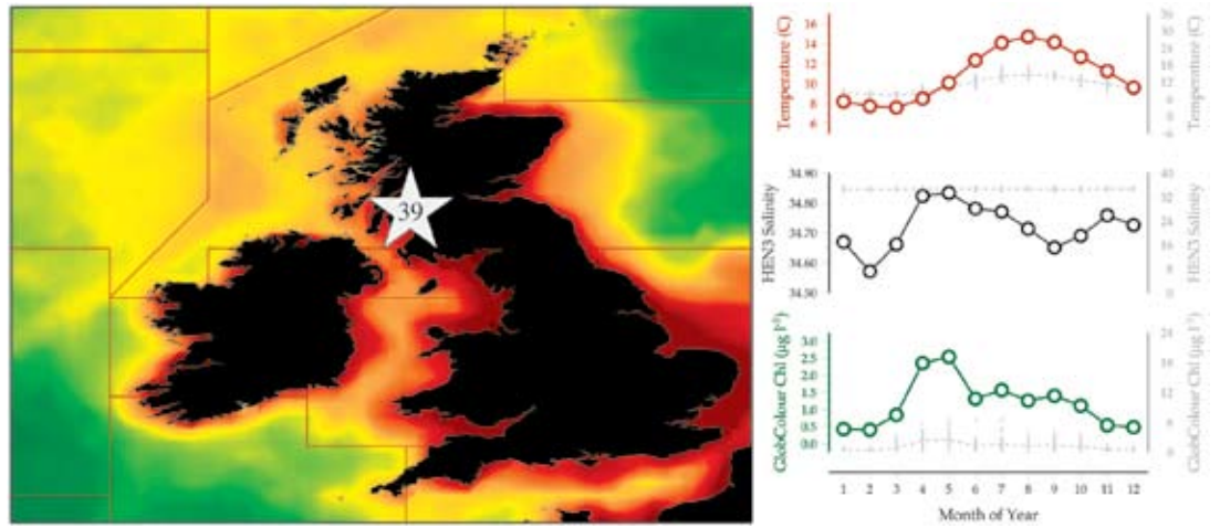
Figure 7.3.1 Location of the Millport plankton monitoring area (Site 39), plotted on a map of average chlorophyll concentration, and its corresponding environmental summary plot (see Section 2.2.1).
