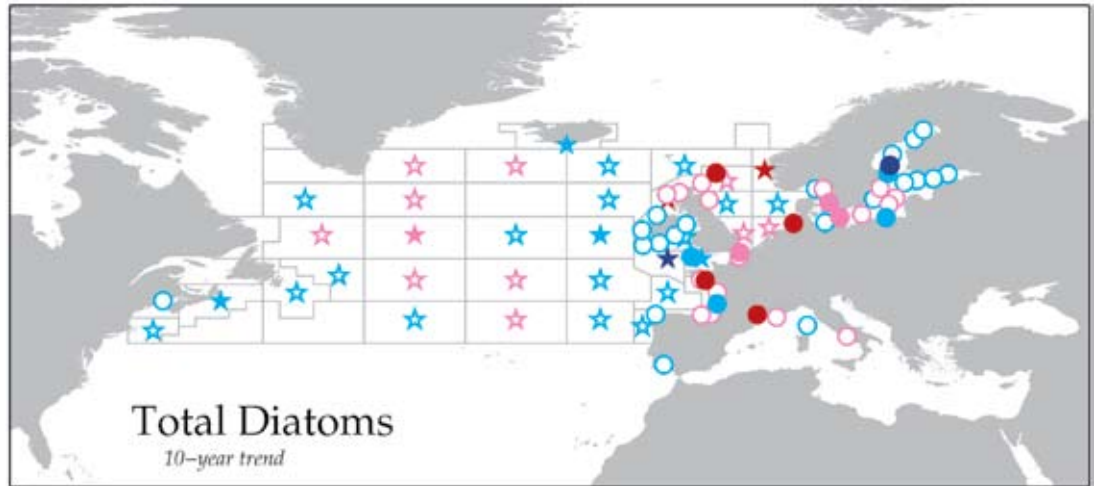
Figure 11.5 Spatio-temporal map of 10-year trends in total diatom abundance present within the CPR standard areas (star symbols) and other monitoring sites (circle symbols). Symbol colors indicate slope (blue/cyan = negative, red/pink = positive) and statistical significance (dark red/blue = p < 0.01 , pink/cyan = p < 0.05 ). Symbols with a white, unfilled, centre indicate slope with a non-significant ( p > 0.05 ) trend.
