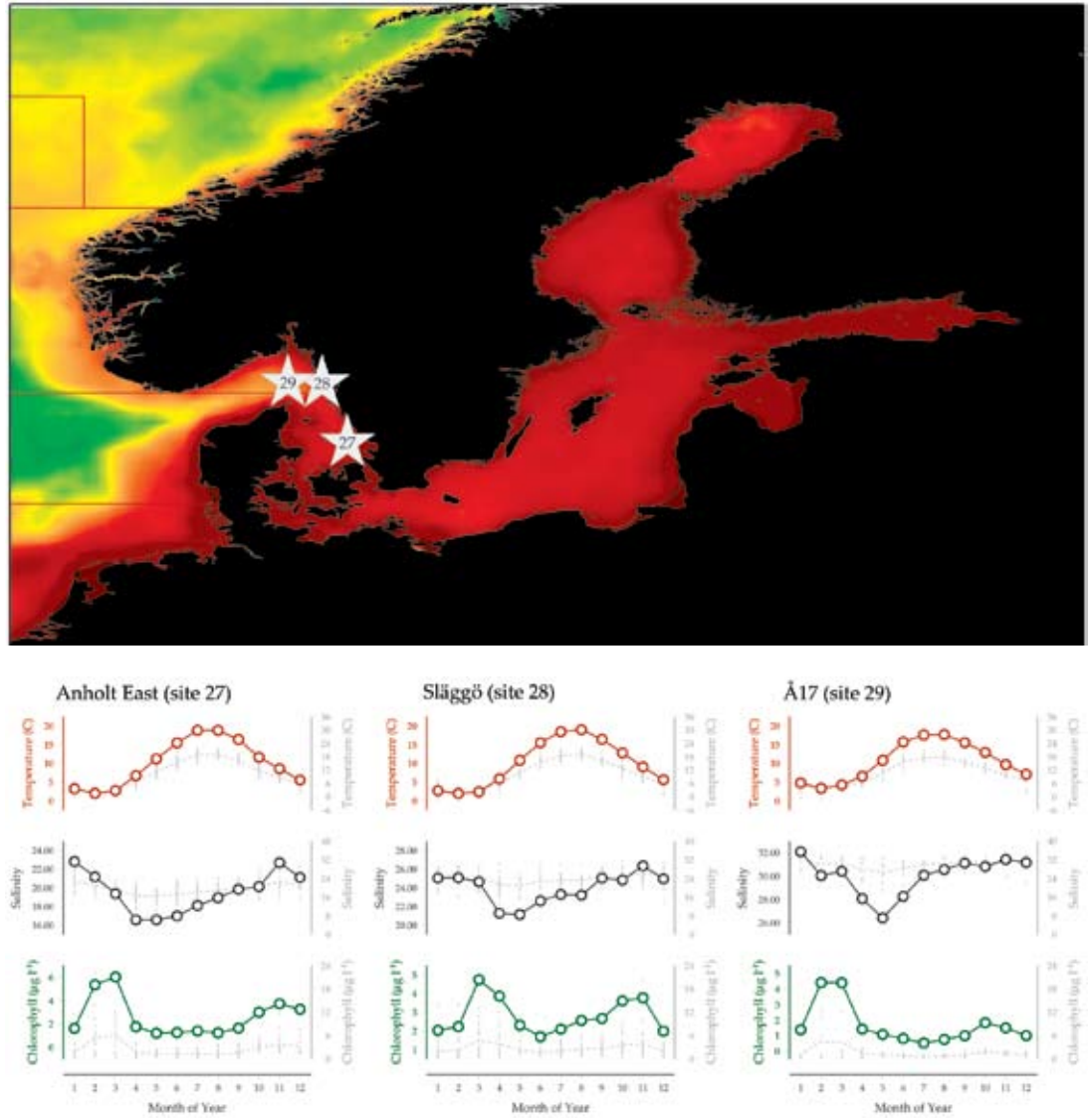
Figure 5.7.1 Locations of the Kattegat and Skagerrak plankton monitoring areas (Sites 27–29), plotted on a map of average chlorophyll concentration, and their corresponding environmental summary plots (see Section 2.2.1).
