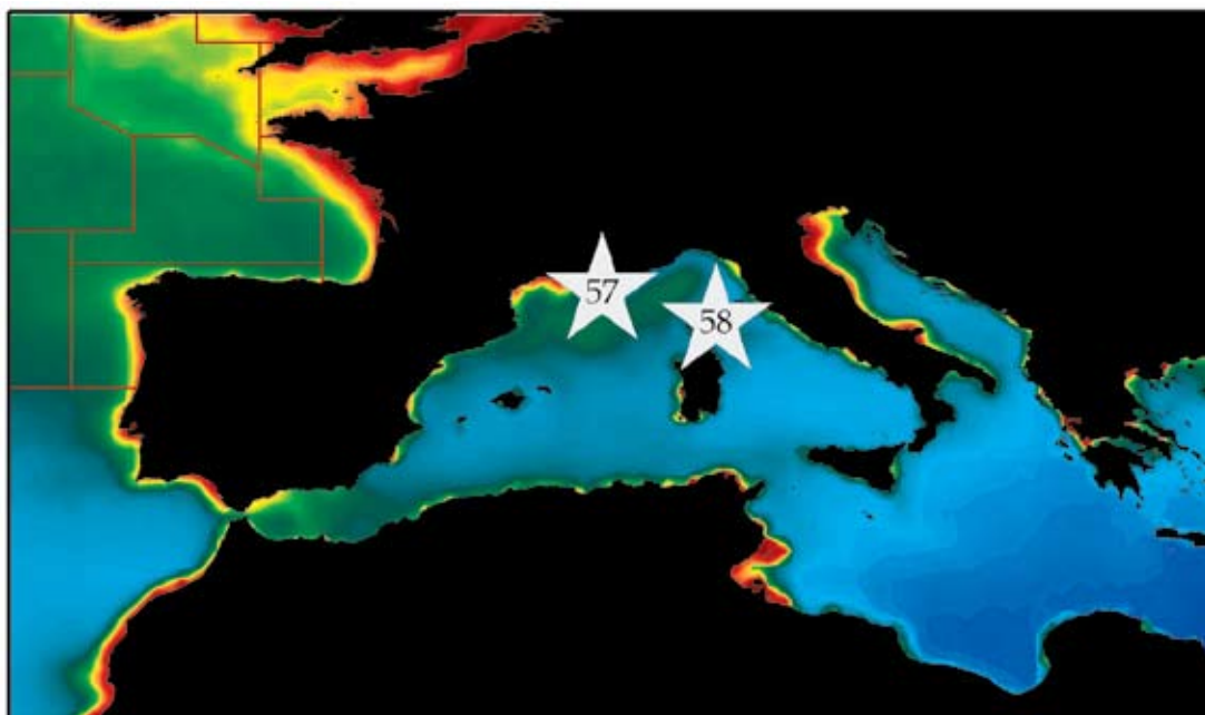
Figure 9.3.1 Locations of the REPHY Mediterranean Sea plankton monitoring areas (Sites 57–58), plotted on a map of average chlorophyll concentration, and their corresponding environmental summary plots (see Section 2.2.1).
