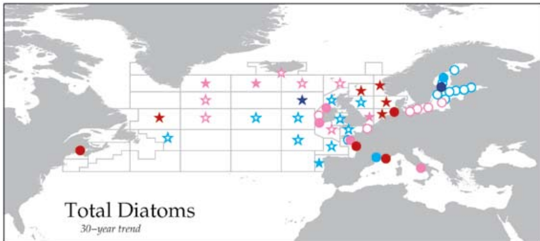
Figure 11.14 Spatio-temporal map of 30-year trends in total diatom abundance present within the CPR standard areas (star symbols) and other monitoring sites (circle symbols). Symbol colors indicate slope (blue/cyan = negative, red/pink = positive) and statistical significance (dark red/blue = p < 0.01 , pink/cyan = p < 0.05 ). Symbols with a white, unfilled, centre indicate slope with a non-significant ( p > 0.05 ) trend.
