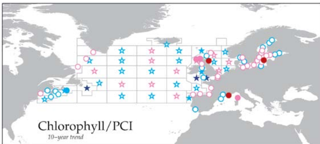
Figure 11.4 Spatio-temporal map of 10-year trends in the Phytoplankton Colour Index present within the CPR standard areas (star symbols) and chlorophyll a present within the other monitoring sites (circle symbols). Symbol colors indicate slope (blue/cyan = negative, red/pink = positive) and statistical significance (dark red/blue = p < 0.01 , pink/cyan = p < 0.05 ). Symbols with a white, unfilled, centre indicate slope with a non-significant ( p > 0.05 ) trend.
