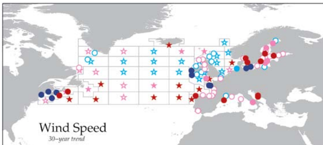
Figure 11.12 Spatio-temporal map of 30-year trends in wind speed present within the CPR standard areas (star symbols) and other monitoring sites (circle symbols). Symbol colors indicate slope (blue/cyan = negative, red/pink = positive) and statistical significance (dark red/blue = p < 0.01 , pink/cyan = p < 0.05 ). Symbols with a white, unfilled, centre indicate slope with a non-significant ( p > 0.05 ) trend.
