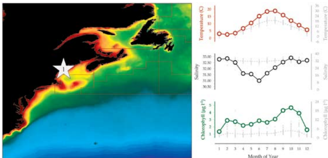
Figure 3.1.1 Location of the Booth Bay, Maine plankton monitoring area (Site 1), plotted on a map of average chlorophyll concentration, and its corresponding environmental summary plot (see Section 2.2.1).
