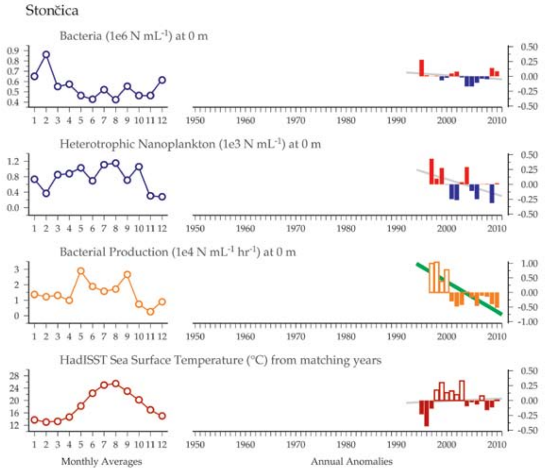
Figure 9.5.3 Multiple-variable comparison plot (see Section 2.2.2) showing the seasonal and interannual properties of select cosampled variables at the Stončica plankton monitoring site. Additional variables from this site are available online at http://wgpme.net/time-series .
