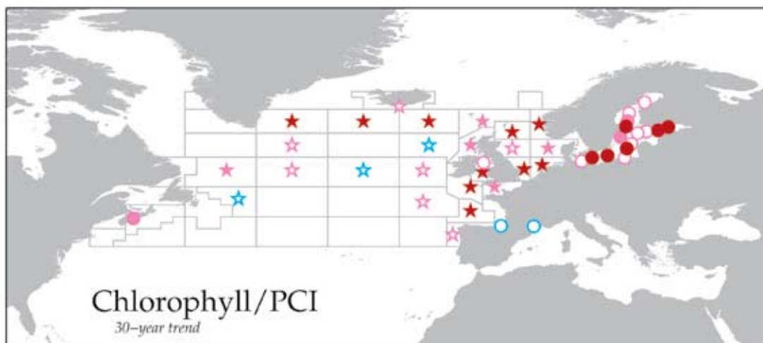
Figure 11.13 Spatio-temporal map of 30-year trends in the Phytoplankton Colour Index present within the CPR standard areas (star symbols) and chlorophyll a present within the other monitoring sites (circle symbols). Symbol colors indicate slope (blue/cyan = negative, red/pink = positive) and statistical significance (dark red/blue = p < 0.01 , pink/cyan = p < 0.05 ). Symbols with a white, unfilled, centre indicate slope with a non-significant ( p > 0.05 ) trend.
