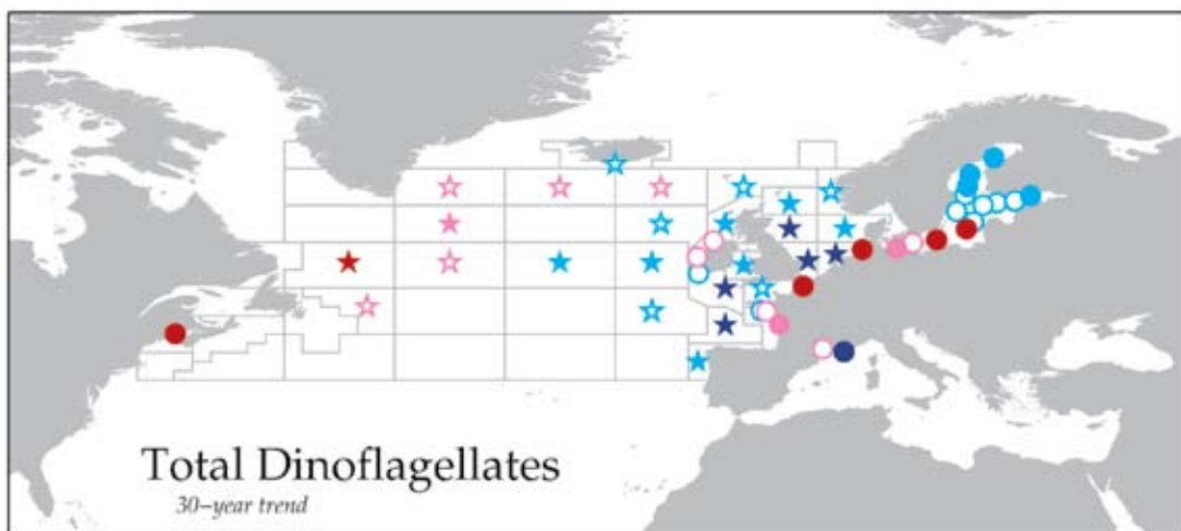
Figure 11.15 Spatio-temporal map of 30-year trends in total dinoflagellate abundance present within the CPR standard areas (star symbols) and other monitoring sites (circle symbols). Symbol colors indicate slope (blue/cyan = negative, red/pink = positive) and statistical significance (dark red/blue = p < 0.01 , pink/cyan = p < 0.05 ). Symbols with a white, unfilled, centre indicate slope with a non-significant ( p > 0.05 ) trend.
