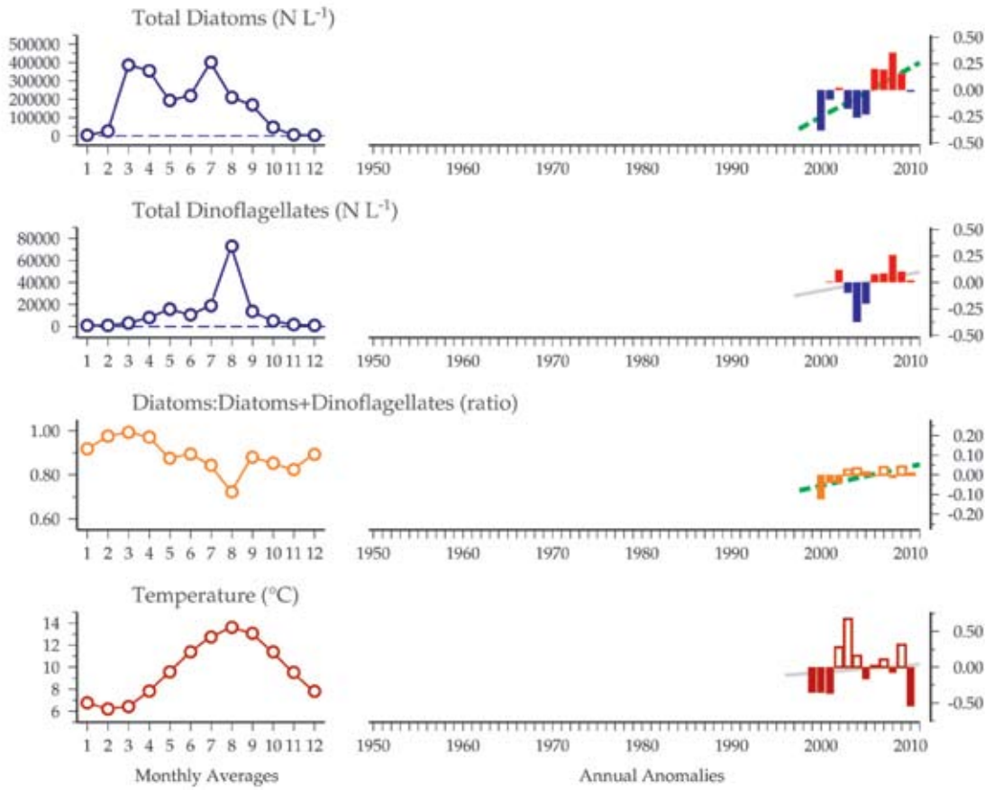
Figure 6.3.2 Multiple-variable comparison plot (see Section 2.2.2) showing the seasonal and interannual properties of select cosampled variables at the Scapa Bay, Orkney plankton monitoring site. Additional variables from this site are available online at http://wgpmc.net/time-series .
