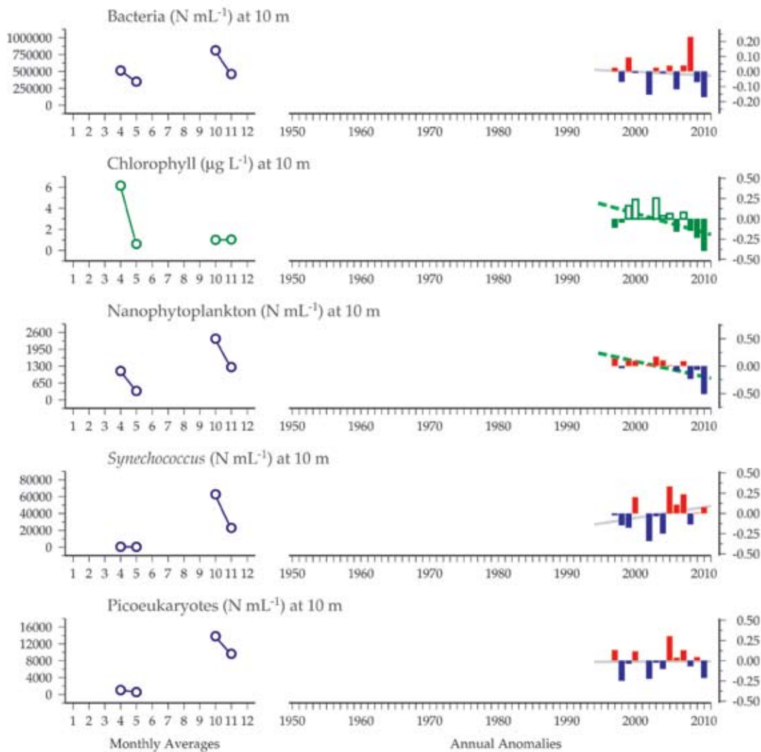
Figure 3.4.4 Multiple-variable comparison plot (see Section 2.2.2) showing the seasonal and interannual properties of select cosampled variables at the Eastern Scotian Shelf plankton monitoring site. Additional variables from this site are available online at http://wgpme.net/time-series .
