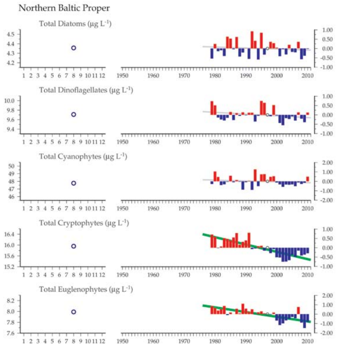
Figure 5.1.5 (continued on facing page) Multiple-variable comparison plot (see Section 2.2.2) showing the seasonal and interannual properties of select cosampled variables at the northern Baltic Proper plankton monitoring site. Additional variables from this site are available online at http://wgpme.net/time-series .
