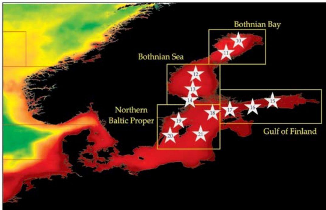
Figure 5.1.1 Location of Finnish Environmental Institute (SYKE) phytoplankton monitoring stations in the northern Baltic Sea (Sites 10–21), and their corresponding environmental summary plots (see Section 2.2.1). The yellow boxes and labels indicate the four subareas described in the report text.
