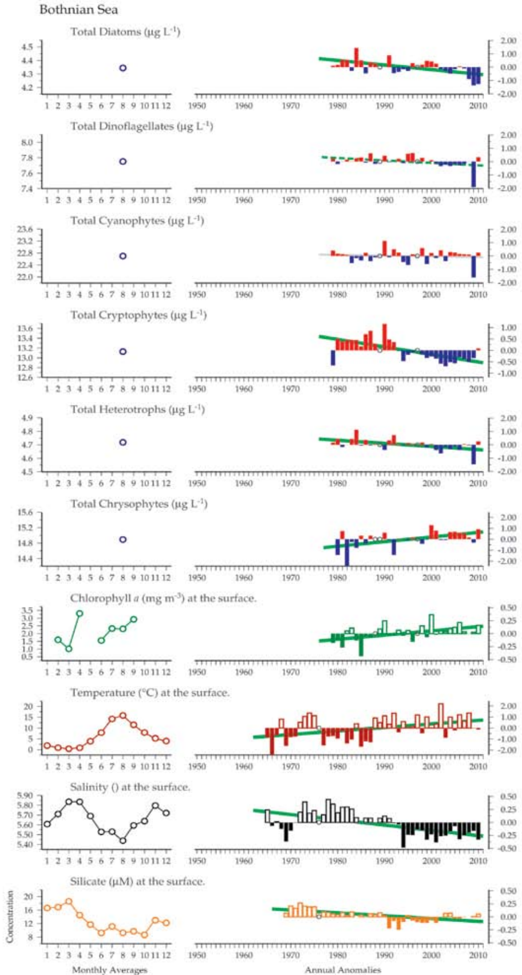
Figure 5.1.3 Multiple-variable comparison plot (see Section 2.2.2) showing the seasonal and interannual properties of select cosampled variables at the Bothnian Sea plankton monitoring site. Additional variables from this site are available online at http://wgpme.net/time-series .
