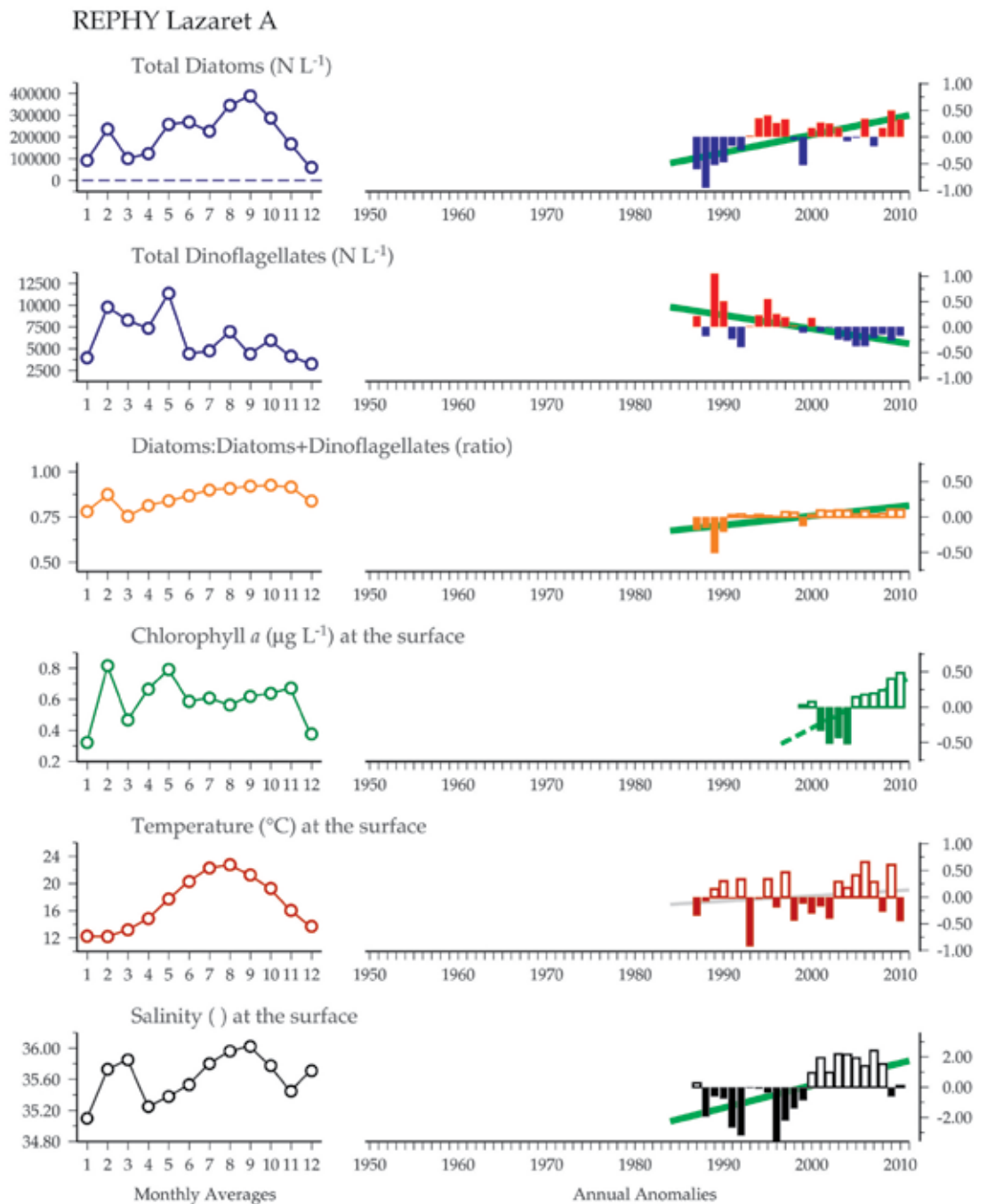
Figure 2.5 Example of a multiple-variable comparison plot (see Section 2.2.2) showing the seasonal and interannual properties of select cosampled variables at the REPHY Lazaret A monitoring site (Site #57, Section 9.3). The green lines drawn in the right figures represent the linear regression of the annual anomalies vs. year. The color and form of these lines indicate the statistical significance of the trend (e.g. solid green is p < 0.01 , dashed green is p < 0.05 ). The grey line (temperature) indicates a non-significant trend.
