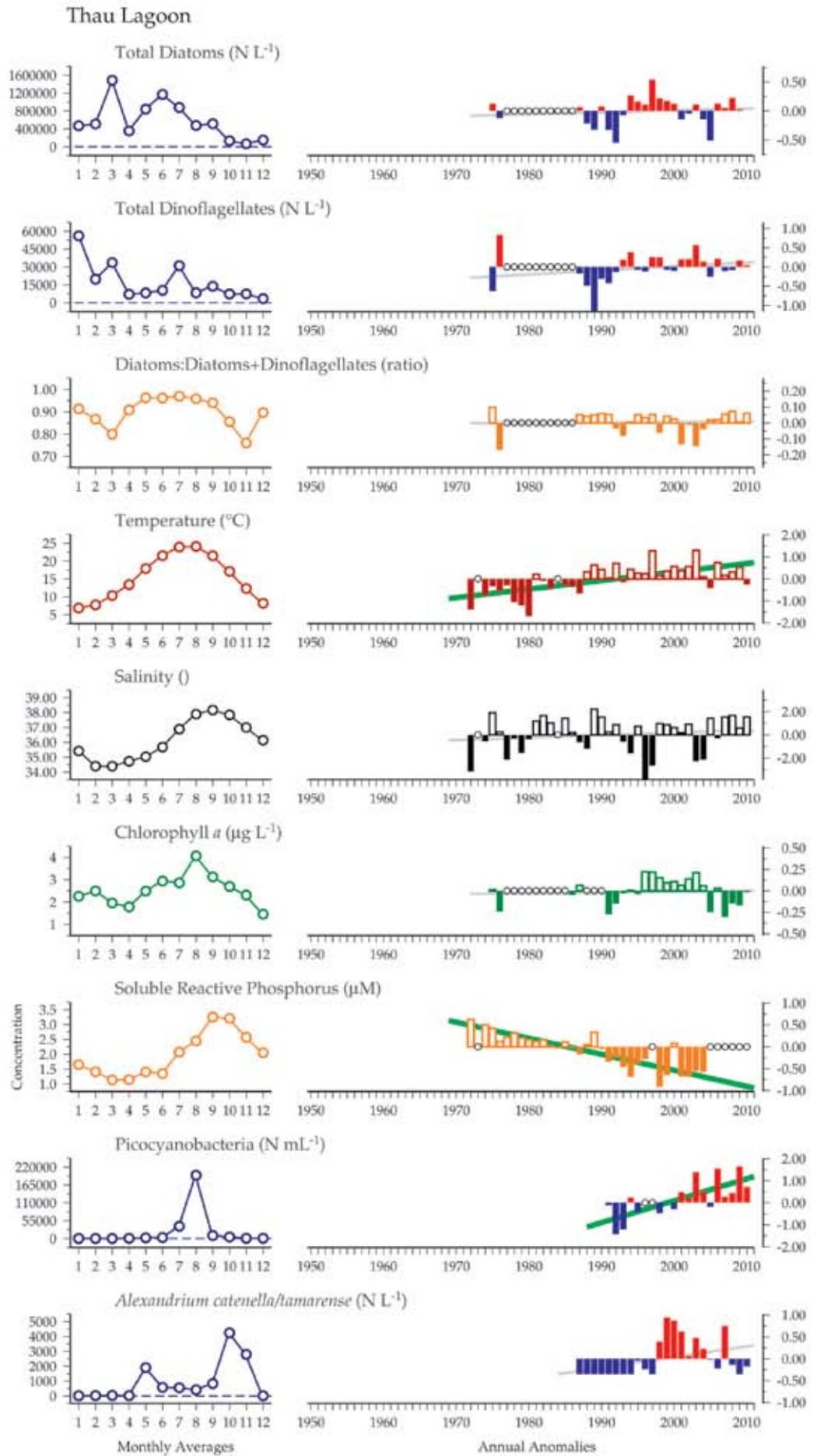
Figure 9.2.2 Multiple-variable comparison plot (see Section 2.2.2) showing the seasonal and interannual properties of select cosampled variables at the Thau Lagoon plankton monitoring site. Additional variables from this site are available online at http://wgpmc.net/time-series .
