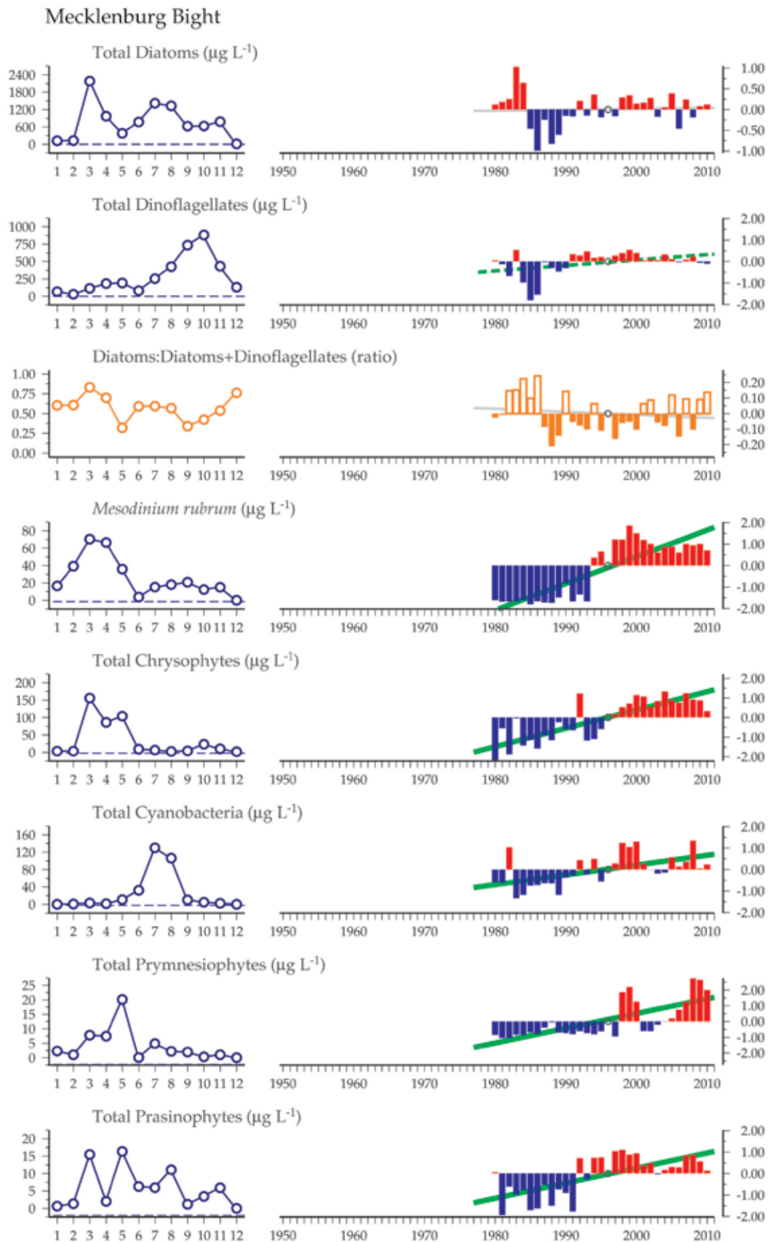
Figure 5.6.2 (continued on facing page) Multiple-variable comparison plot (see Section 2.2.2) showing the seasonal and interannual properties of select cosampled variables at the Mecklenburg Bight plankton monitoring site. Additional variables from this site are available online at http://wgpme.net/time-series .
