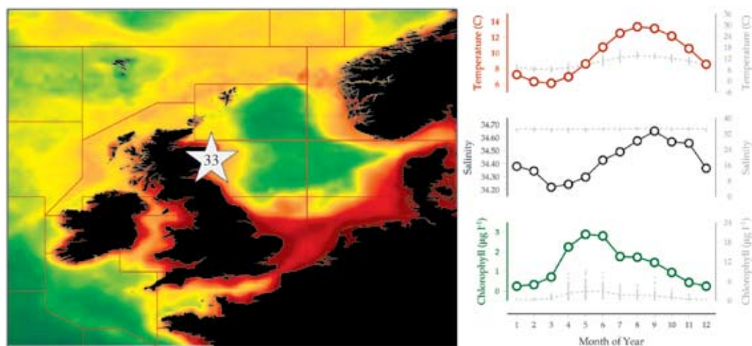
Figure 6.4.1 Location of the Stonehaven plankton monitoring area (Site 33), plotted on a map of average chlorophyll concentration, and its corresponding environmental summary plot (see Section 2.2.1).
