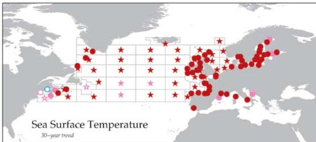
Figure 11.11 Spatio-temporal map of 30-year trends in sea surface temperature present within the CPR standard areas (star symbols) and other monitoring sites (circle symbols). Symbol colors indicate slope (blue/cyan = negative, red/pink = positive) and statistical significance (dark red/blue = p < 0.01 , pink/cyan = p < 0.05 ). Symbols with a white, unfilled, centre indicate slope with a non-significant ( p > 0.05 ) trend.
