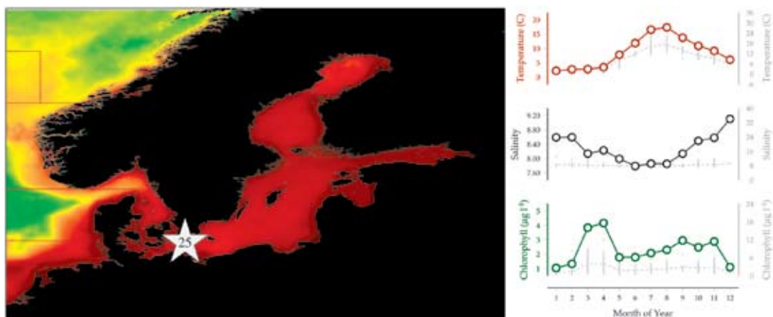
Figure 5.5.1 Location of the Arkona Sea plankton monitoring area (Site 25), plotted on a map of average chlorophyll concentration, and its corresponding environmental summary plot (see Section 2.2.1).
