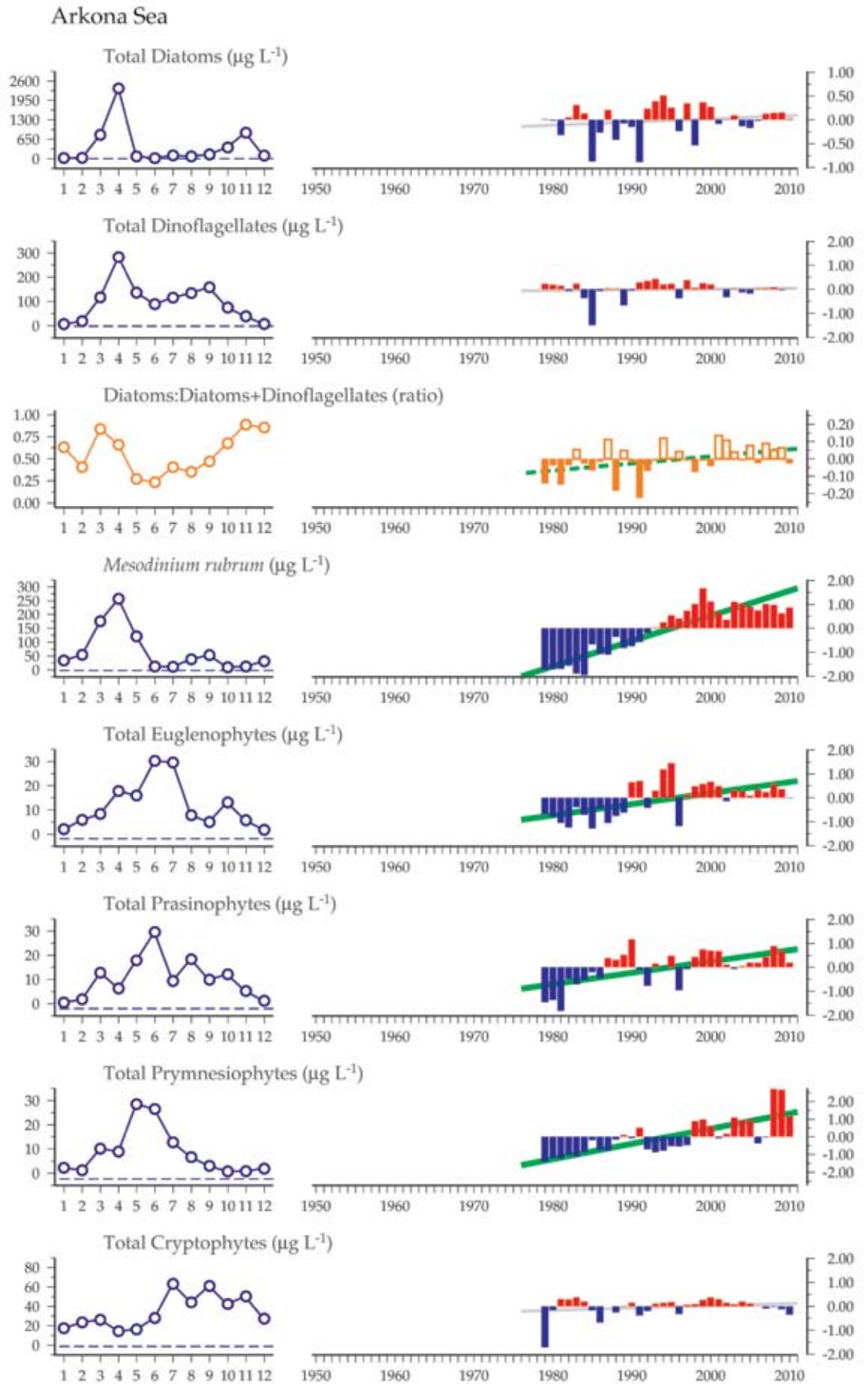
Figure 5.5.2 (continued on facing page) Multiple-variable comparison plot (see Section 2.2.2) showing the seasonal and interannual properties of select cosampled variables at the Arkona Sea plankton monitoring site. Additional variables from this site are available online at http://wgpme.net/time-series .
