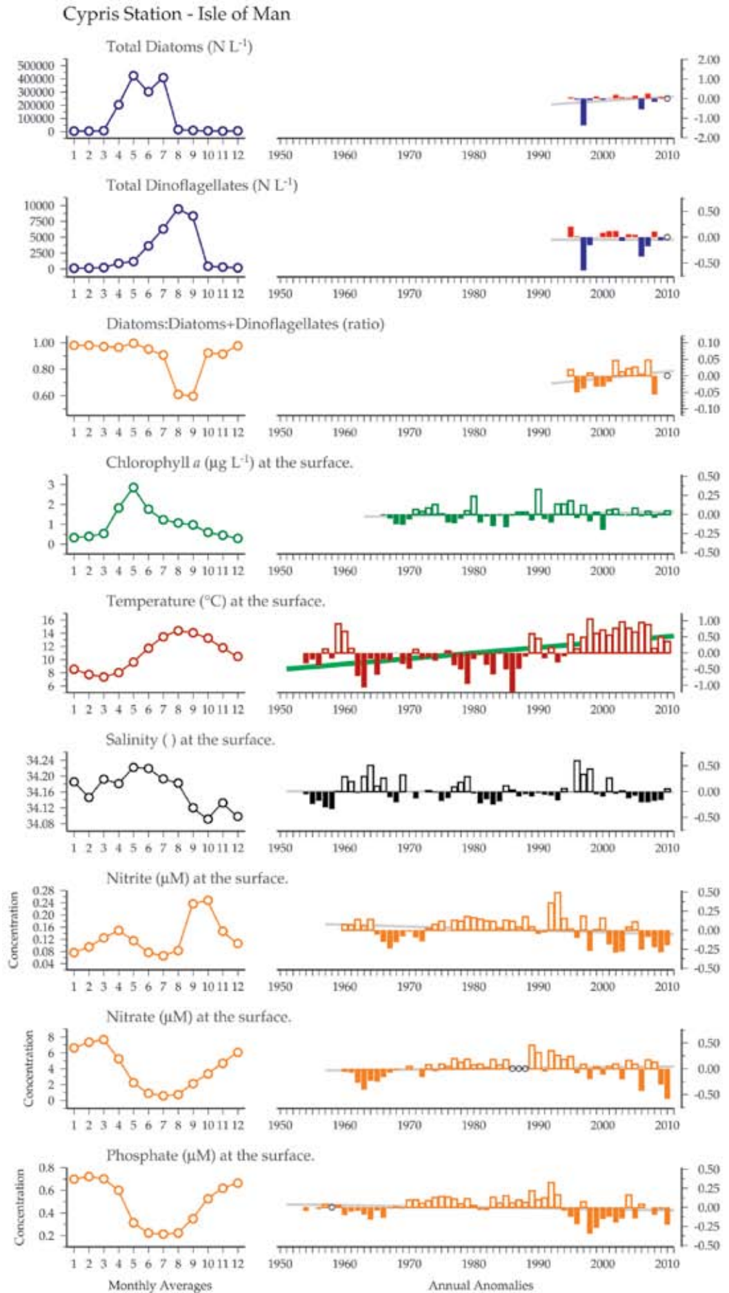
Figure 7.4.2 Multiple-variable comparison plot (see Section 2.2.2) showing the seasonal and interannual properties of select cosampled variables at the Cypris Station, Isle of Man plankton monitoring site. Additional variables from this site are available online at http://wgpmc.net/time-series .
