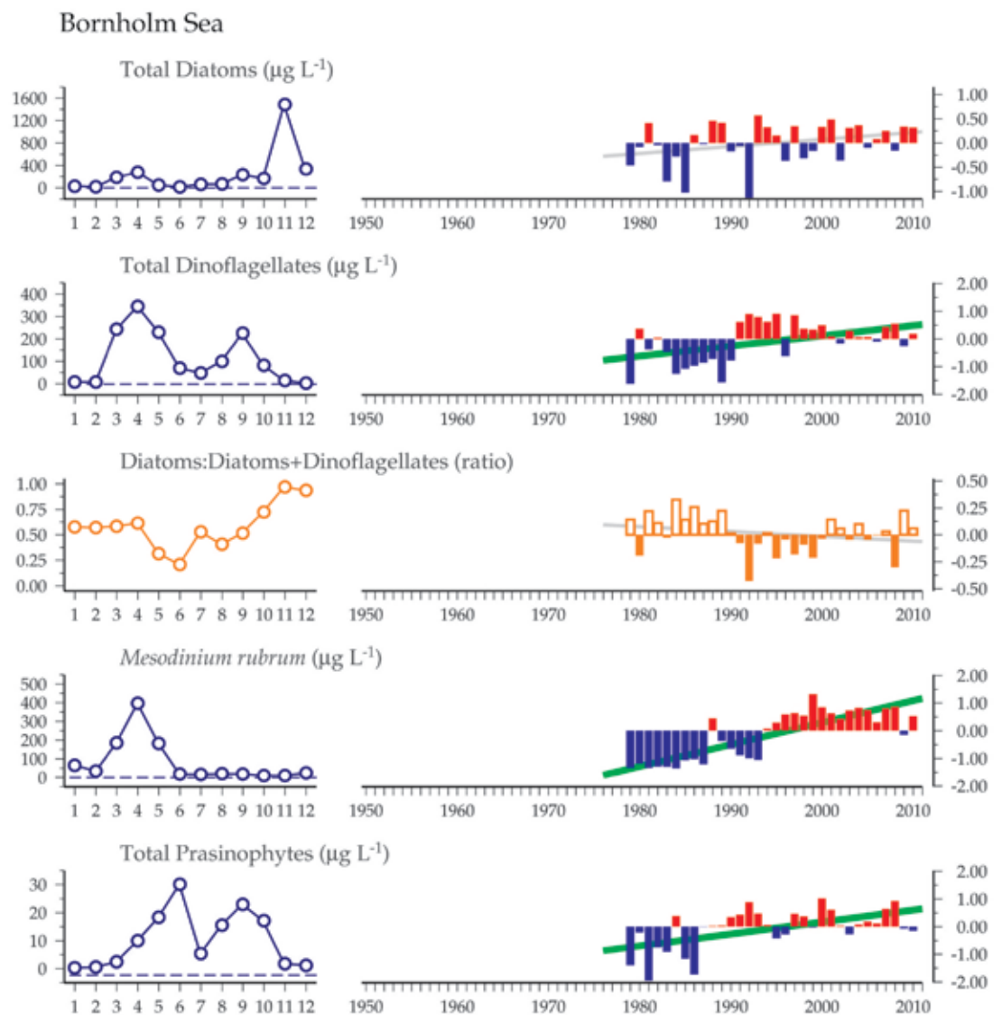
Figure 5.4.2 (continued on facing page) Multiple-variable comparison plot (see Section 2.2.2) showing the seasonal and interannual properties of select cosampled variables at the Bornholm Sea plankton monitoring site. Additional variables from this site are available online at http://wgpme.net/time-series .
