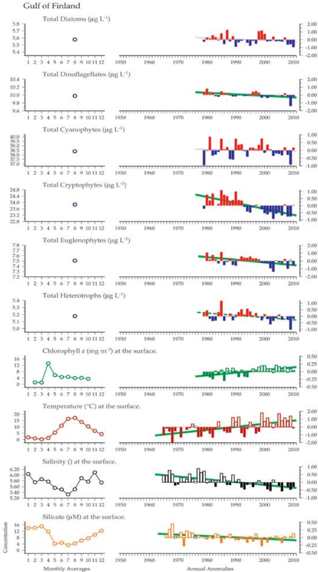
Figure 5.1.4 Multiple-variable comparison plot (see Section 2.2.2) showing the seasonal and interannual variability of select cosampled variables at the Gulf of Finland plankton monitoring site. Additional variables from this site are available online at http://wgpmc.net/time-series .
