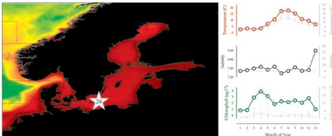
Figure 5.4.1 Location of the Bornholm Sea plankton monitoring area (Site 24), plotted on a map of average chlorophyll concentration, and its corresponding environmental summary plot (see Section 2.2.1).
