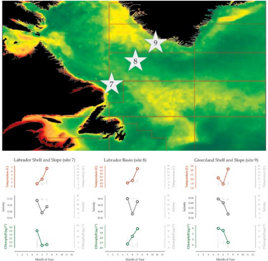
Figure 4.1.1 Locations of the Labrador Sea plankton monitoring areas (Sites 7–9), plotted on a map of average chlorophyll concentration, and their corresponding environmental summary plots (see Section 2.2.1).
