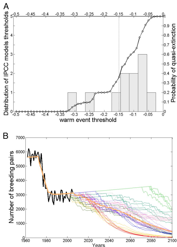
Fig. 3. Quasi-extinction and population projection. (A) Probability of quasi-extinction (a decline of 95% or more) of the emperor penguin population in Terre Adélie by 2100, as a function of the warm event thresholds. The distribution of warm event thresholds calculated for the 10 IPCC models is represented by the gray bars, and warm event threshold calculated from Fig. 2B for the satellite observation by the vertical dotted line. The probability of quasi-extinction varied from 0.36 to 0.84 over the range of likely thresholds [-0.15; 0.07] . (B) Observations and projections of the emperor penguin population. The thick dark line is the observed number of breeding pairs. The thick orange line from 1962 to 2000 is the projected number of breeding pairs based on the observed sequence of warm events. The thick red line from 2005 to 2100 is the median of 10,000 stochastic projections based on the forecasts of SIEa produced by the 10 IPCC models. To give a sense of the variability in these projections, 30 projections from 2005 to 2100 (three for each climate model) are shown; line colors as in Fig. 2.
