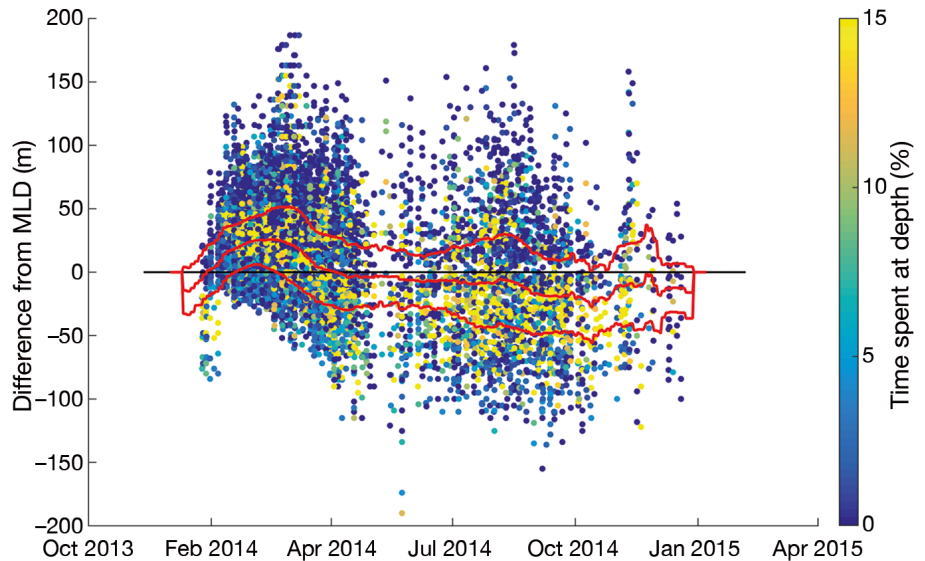
Fig. 5. Times series of depth-difference between 15 juvenile emperor penguins' depth and the mixed layer depth (MLD). Positive values: deeper than MLD. The color scale represents the time spent at depth. The middle red line corresponds to the average distance from the MLD (using a moving window of 30 d) weighted by the time spent at depth (i.e. where the penguins spent most of their time relative to the MLD). The bottom and top red lines correspond to the standard deviation of this moving weighted average
