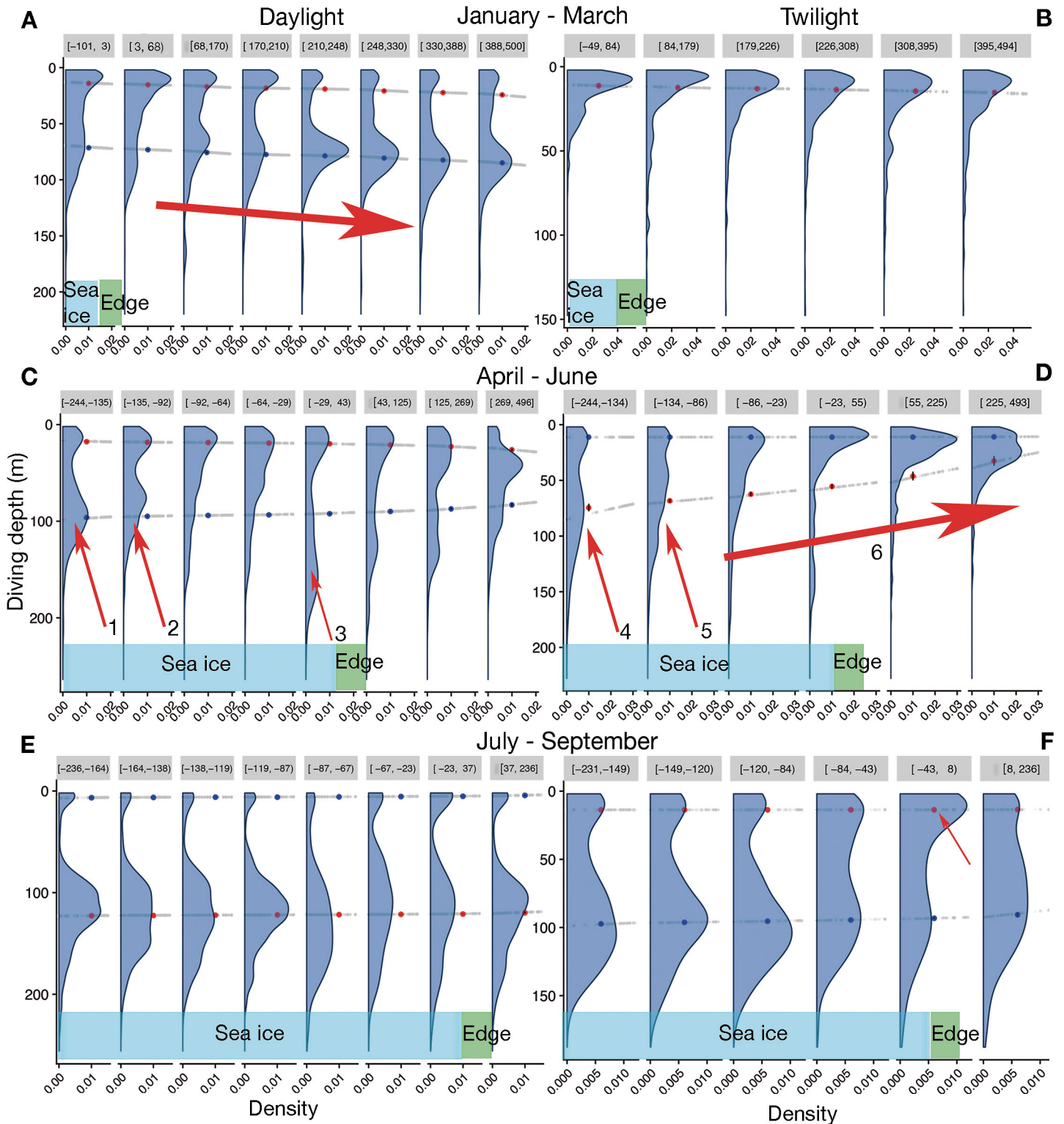
Fig. 3. Density plots of the diving depth of juvenile emperor penguins relative to their distance from the sea ice edge (grey boxes: distance bins, km) for daytime and twilight respectively across (A,B) summer, (C,D) autumn and (E,F) winter. For illustration purposes, the distance from the sea ice edge was binned in 8 classes for daylight (A,C,E) and 6 classes for twilight (B,D,F) of equal numbers of observations. Fitted values from mixture model 'a' are represented by grey dots, and the mean fitted value per bin of distance from the sea ice edge is represented in red or blue for each component. Red arrows correspond to comments in the main text of Section 3.2
