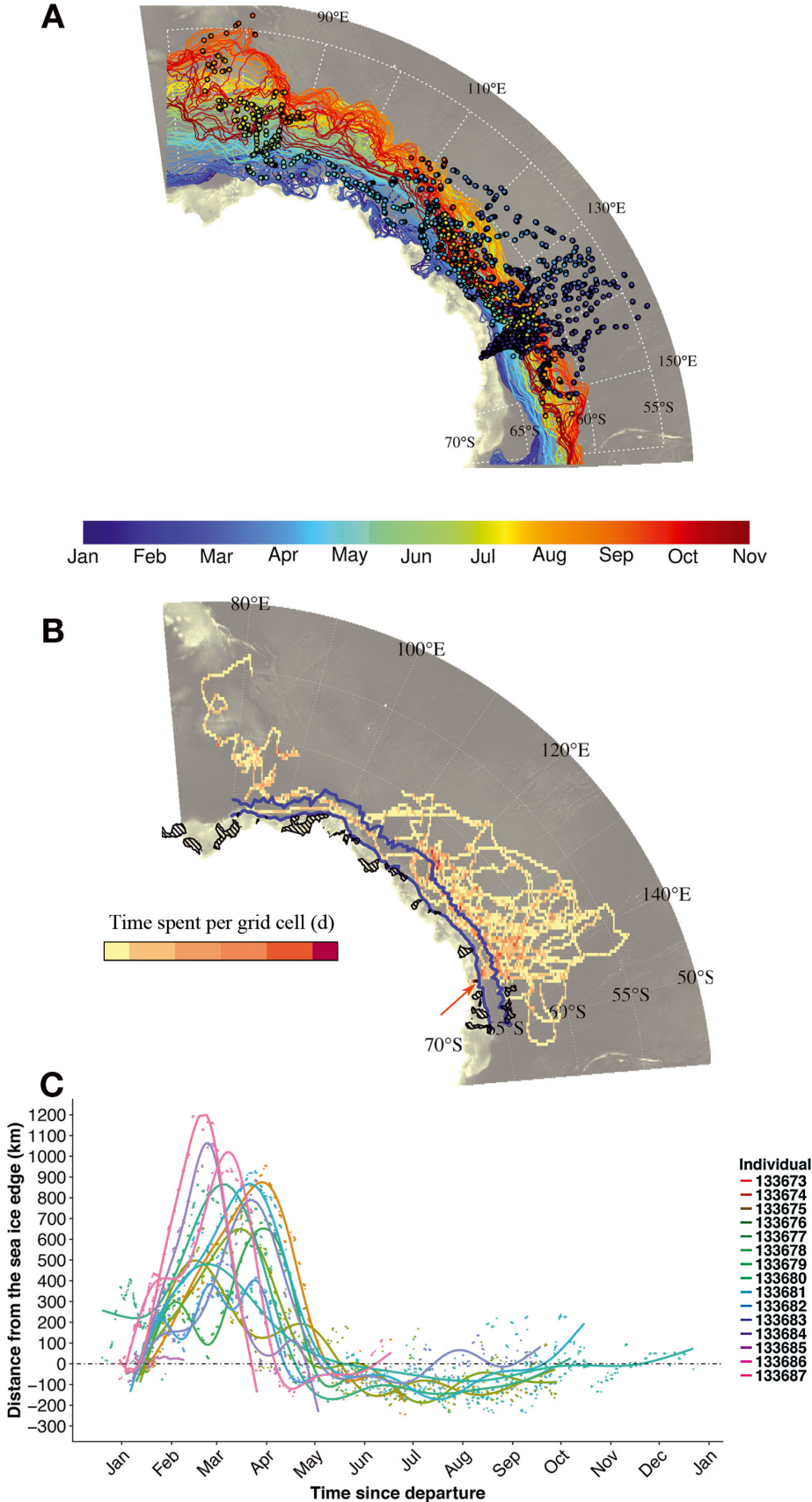
Fig. 1. At-sea distribution of 15 juvenile emperor penguins equipped with SPLASH tags in 2013–2014 (dots). (A) Tracks of the 15 juveniles linked with the seasonality of the sea ice in the East Antarctic region. The color scale represents time; the sea ice extent of a given day and associated penguin positions are colored in the same way. For simplicity, sea ice extent is only shown for every third day. Sea ice extent was obtained from SSM/IS daily sea ice concentration (resolution 25 km). (B) Sum of the time spent across all individual penguins per grid cell ( 148.2 \times 296 km). The 2 blue lines delineate the continental slope area. The black-hatched polygons represent the polynya areas computed using annual sea ice production from March to October 2014 as developed by Labrousse et al. (2018). The red arrow shows the small polynya close to the colony used by the penguins. (C) Time-series of the distance from the sea ice edge for each of the 15 individuals. Color scale corresponds to each individual. Smoothing lines were fitted for each individual observation
