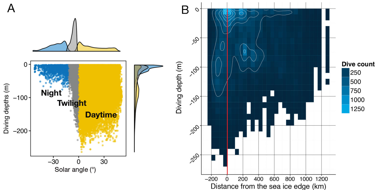
Fig. 2. Diving depth distribution across time of day and distance from the sea ice edge for 15 juvenile emperor penguins. (A) Diving depth versus the solar angle. Day dives are in yellow, twilight dives in grey and night dives in blue. The density distributions of the solar angle and the diving depths for each group are represented at the top and right side, respectively. (B) Diving depth relative to the bird's distance from the sea ice edge using a 2D kernel density estimation with a bandwidth of 50 m for the diving depth and 10 km for the distance from the sea ice edge (kde2D function from package MASS, R Development Core Team; Venables & Ripley 2002). One contour is drawn every 250 dives. The red line represents the sea ice edge
