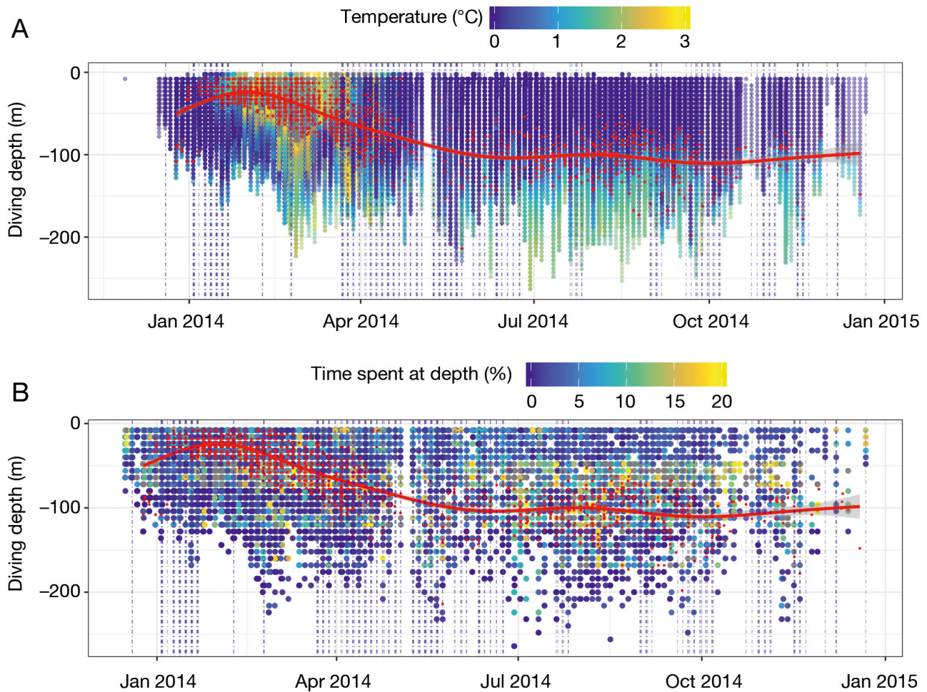
Fig. 4. Times series of depth-temperature profiles and depth-time indexes for 15 juvenile emperor penguins. (A) Minimum temperature profiles ( n = 3538 ) collected during the birds' trips at sea and recorded as profiles of depth and temperature (PDTs). (B) Time spent at depth along each PDT. For illustration purposes only, we linked the 4 h summary PDTs with the 4 h summary time-at-depth histograms. For each PDT, we looked at the corresponding time-at-depth histogram based on the date, time and depth; we then attributed the time spent at depth to each depth of the PDT. Red dots represent the mixed layer depth for each profile. Red curve: predicted values of a smooth fitted line of the mixed layer depths (generalized additive model); grey shaded envelope: 95 %CI of the predicted values. The dashed vertical blue lines correspond to profiles located on the slope region
