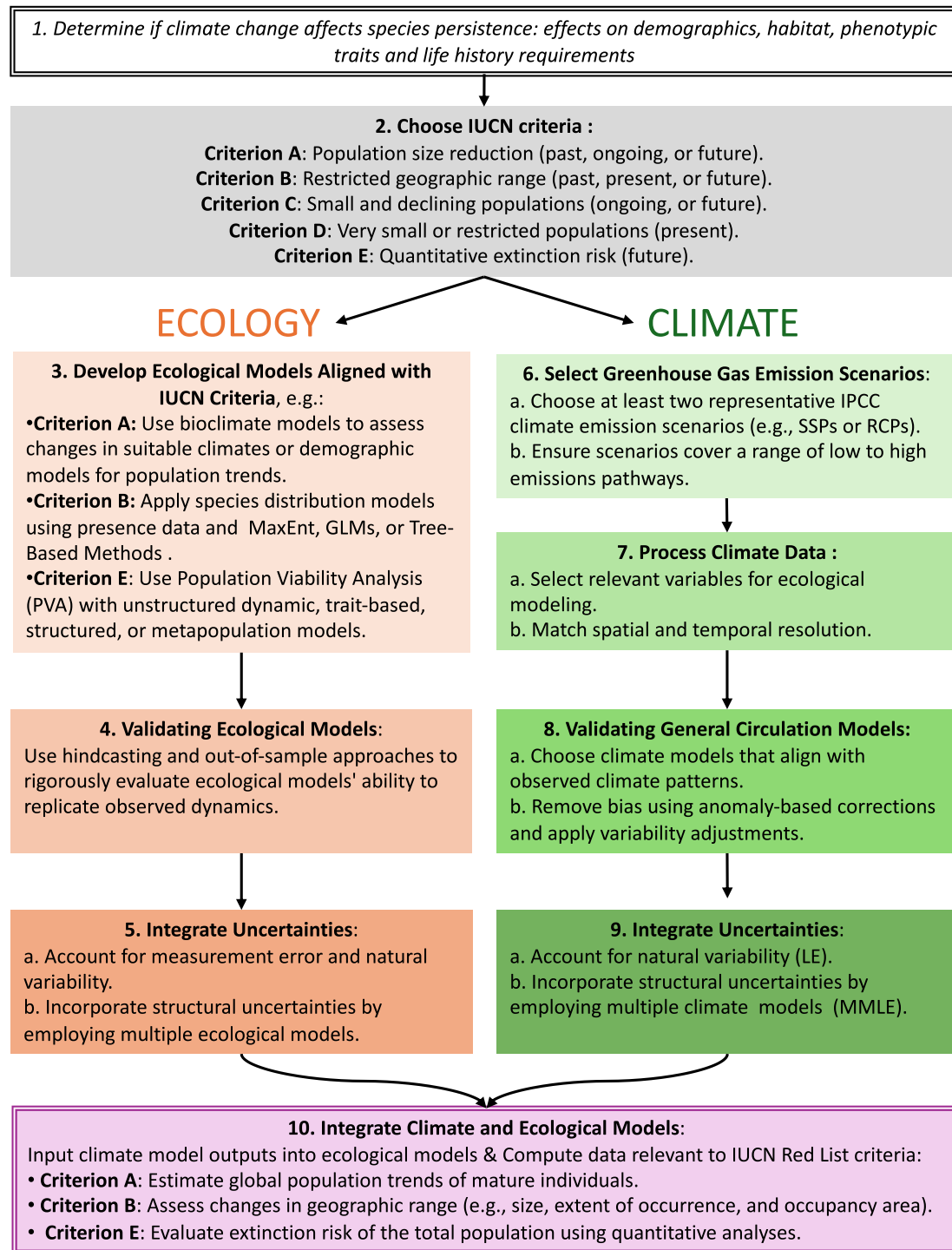
Fig. 1. Framework for assessing climate change impacts on species for the International Union for Conservation of Nature (IUCN) Red List. The process starts by identifying the impacts of climate change on species persistence, considering demographics, habitat suitability, phenotypic traits, and life history requirements (Box 1), which informs the selection of appropriate IUCN criteria (Gray Box 2). Ecological models tailored to these criteria are developed (Light Orange Box 3) and validated (Orange Box 4). Climate projections are built using at least two greenhouse gas emissions scenarios, such as Shared Socioeconomic Pathways (SSPs) or Representative Concentration Pathways (RCPs), to represent a range of emissions pathways (Light Green Box 6). These data are processed by selecting relevant variables, aligning resolutions (Green Box 7), choosing climate models that agree well with observed climate patterns, and applying corrections for biases and variability (Dark Orange Box 5 and Dark Green Box 8). Uncertainties are integrated through ecological and climate model ensembles, addressing natural variability and structural differences (Green Box 9). The final step combines processed climate outputs with ecological models to compute metrics relevant to the selected criteria, enabling a robust and uncertainty-informed evaluation of extinction risks (Purple Box 10). (Interpretation of the references to color in this figure legend is available in the web version of this article. The boxes are also numbered, ensuring clarity even in grayscale print.)
