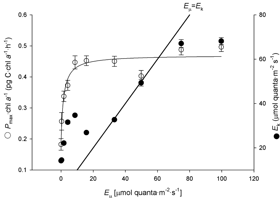
FIG. 3. Maximum photosynthetic rates at a range of acclimation irradiances and the saturation point of photosynthesis are plotted against growth irradiance. The line E_\mu = E_k is also shown. Data points represent experimental averages \pm standard deviation ( n = 2 ). When photosynthetic rate is normalized to chl, the high chl a content of low-irradiance-acclimated cells reduces efficiency of each chl a molecule due to self-shading. Cultures incubated at light intensities below E_0 retained low amounts of photosynthetic capacity in spite of their poor health but were less photosynthetically active overall compared with higher-light acclimations.
