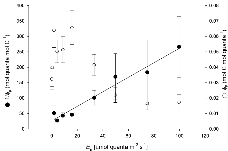
FIG. 4. The inverse of the quantum yield for growth ( \phi_\mu ) calculated according to Falkowski et al. (1985). \phi_\mu was calculated only for cultures with positive growth rates. The maximum quantum yield for photosynthesis ( \phi_P ) is also shown. Data points indicate mean \pm standard deviation ( n = 2 ). The quantum requirement for carbon assimilation increases linearly ( r^2 = 0.96 ) with increasing irradiance, indicating that Mesodinium rubrum is a less efficient phototroph under high-light conditions. \phi_P declined with increasing growth irradiance, so that light-limited cultures ( E_\mu < E_{\text{sat}} ) were more photosynthetically efficient than their light-saturated counterparts.
