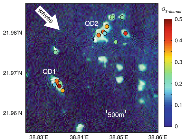
Fig. 6 USGS LandsAT image of Qita Dukais reef system. Circles show the location of Onset Temp Pros on the reef knolls and the color represents diurnal temperature variability at each location, estimated as, \sigma_{T\text{-diurnal}} = \sigma(T_{33\text{hr-hpf}}) , the standard deviation of the 33-h high-pass-filtered temperature
