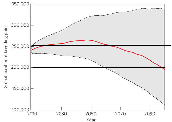
Figure 4 | Global number of breeding pairs of emperor penguins from 2009 to 2100. This global population size is calculated using SICa projections from AOGCMs selected with the local selection approach (see Supplementary Section 7 for results of alternative AOGCM selections). The red line is the median and the grey area is the 90% envelope from stochastic simulations of population trajectories.
