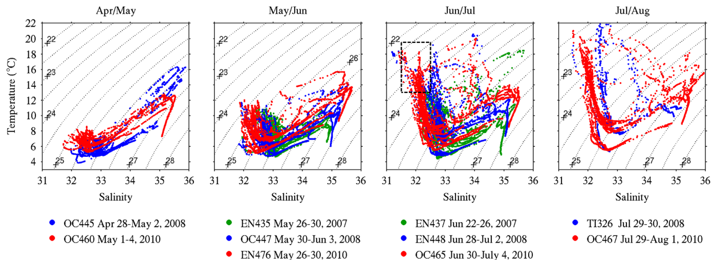
Fig. 6. Temperature/salinity characteristics of hydrographic profiles on Georges Bank: 2007, 2008, 2010. Cruise numbers refer to Table 1. The dashed box in the June/July panel indicates the criteria ( 31.5 < S < 32.5 , 13.0\text{ }^{\circ}\text{C} < T < 19.0\text{ }^{\circ}\text{C} ) used to infer the origin of the water mass anomaly associated with bloom decline in 2008 (see text).
