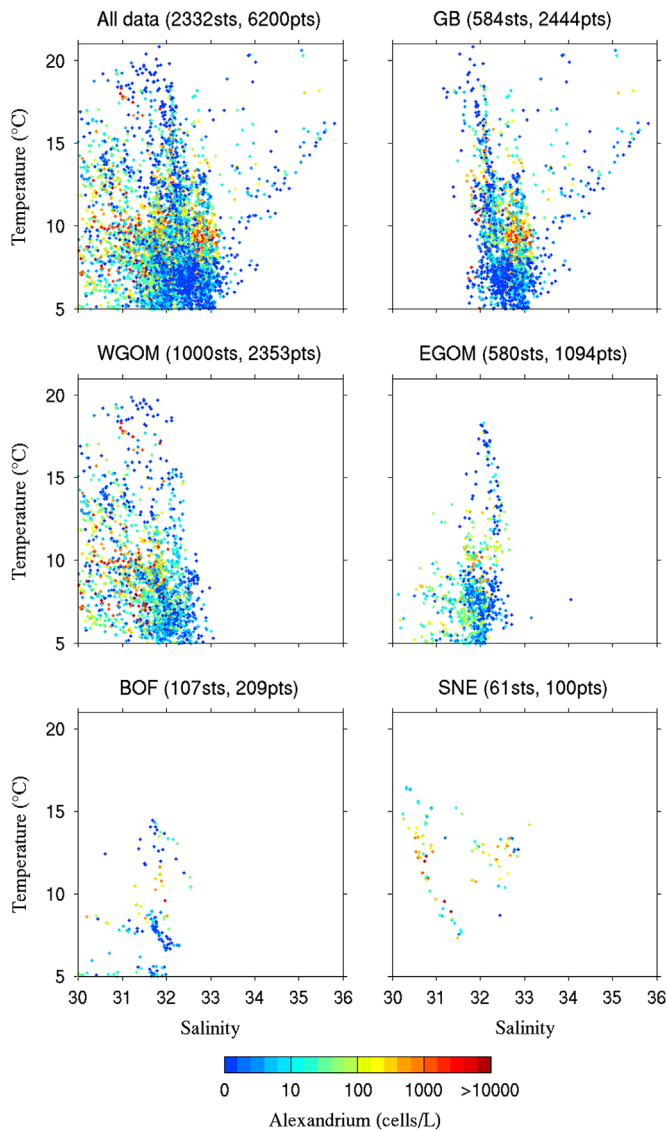
Fig. 10. A. fundyense concentration plotted as a function of temperature and salinity for the entire Gulf of Maine/Georges Bank region (upper left) and various subdomains: Georges Bank (GB), the western Gulf of Maine (WGOM), the eastern Gulf of Maine (EGOM), the Bay of Fundy (BOF), and the southern New England shelf (SNE). Note that these plots include not only data from the present study, but also prior data in the region starting in 1998 (Anderson et al., 2005b; Keafer et al., 2005; McGillicuddy et al., 2005b; Townsend et al., 2001); live counts from OC440 (October 8–18, 2007, Fig. 2) are not included.
