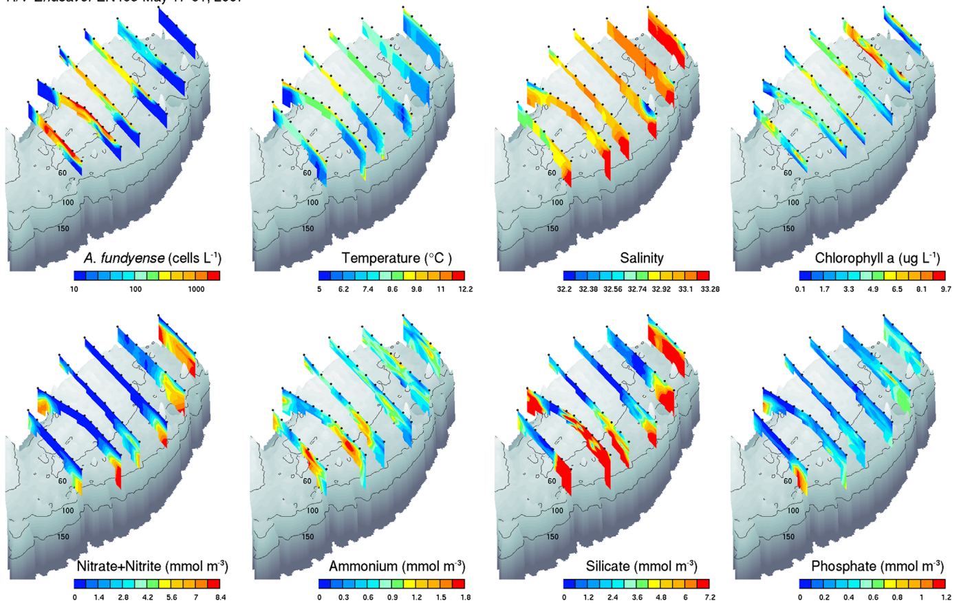
Fig. 3. Vertical sections of A. fundyense , temperature, salinity, chlorophyll a, nitrate+nitrite, ammonium, silicate, and phosphate from R/V Endeavor cruise EN435, May 17–31 2007. Black dots along the top of each section indicate the station locations. Standard sampling depths were 1, 10, 20, 30, 40, 50, 100, 150, 200, 250 m/near bottom. Gray shading shows bathymetry; 60 m, 100 m, and 150 m isobaths are indicated.
