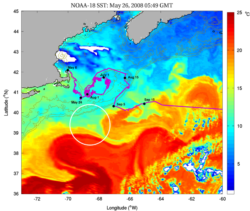
Fig. 8. Sea surface temperature image for May 26, 2008. The white circle indicates the meander-driven shelf water export described in the text. Trajectory of a surface drifter released northeast of Cape Cod on May 6 is plotted in magenta (drifter ID #85291 obtained from http://www.nefsc.noaa.gov/drifter/ ).
