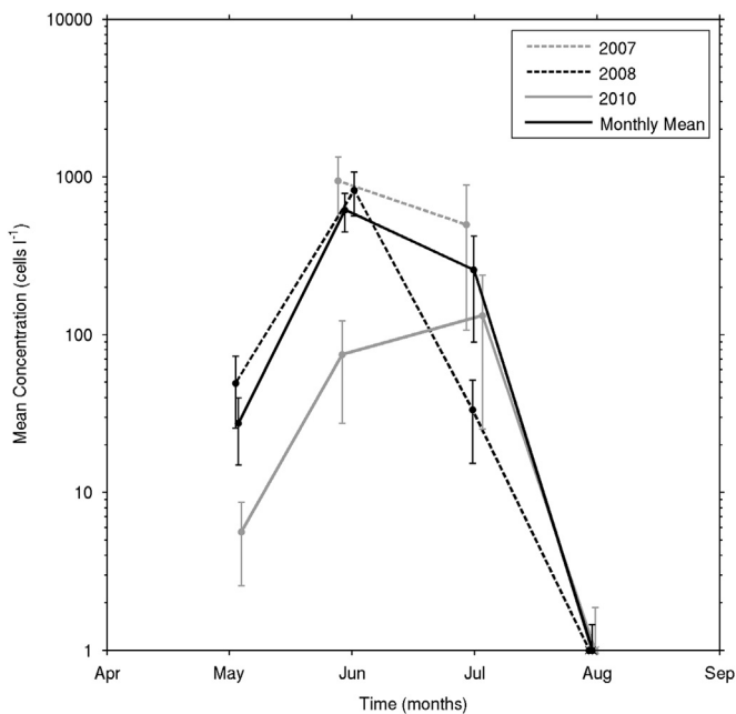
Fig. 5. Seasonal to interannual variability in surface A. fundyense concentrations on Georges Bank.
