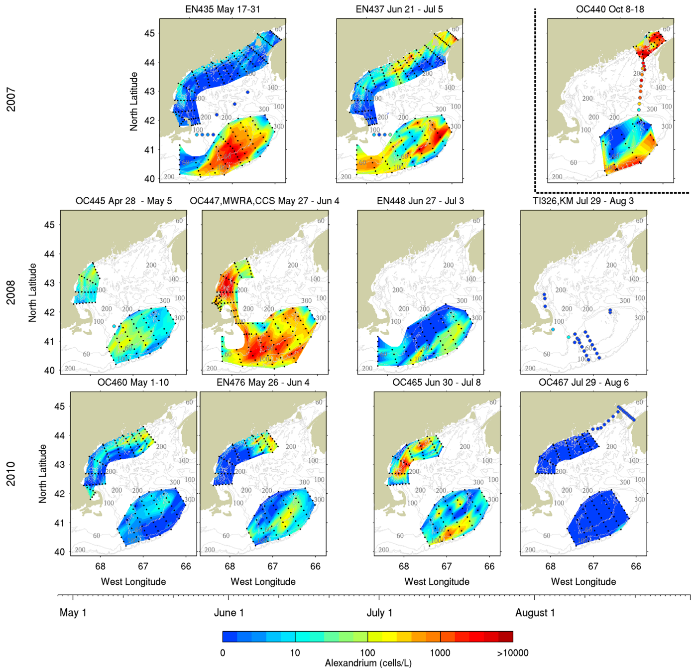
Fig. 2. A. fundyense surface concentrations observed on survey cruises in 2007, 2008, and 2010. Black dots denote the locations of samples used to construct the maps; colored dots indicate A. fundyense surface concentrations in areas for which there are not sufficient data to map the distribution. The horizontal position of each map reflects the timing of each survey (time axis located above the color bar), with the exception of the upper right panel which reports “live” microscope counts from underway samples collected during the fall 2007 cyst survey (October 8–18, 2007). The live counts from fall 2007 are presented for informational purposes only and not included in further analysis.
