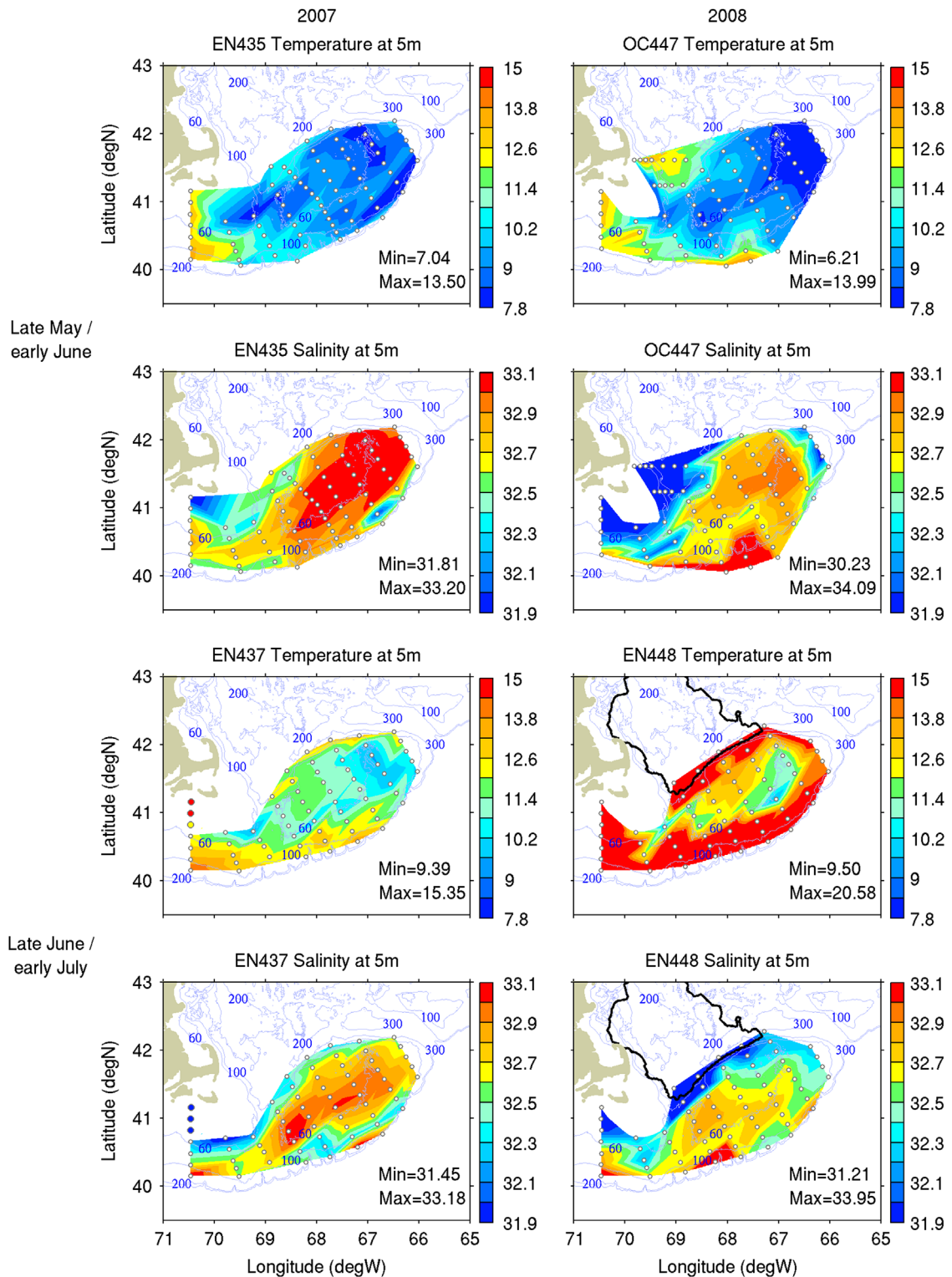
Fig. 7. Temperature and salinity at 5 m in late May/early June and late June/early July 2007 and 2008. Solid black contour in the lower right panels indicates the origin of the water mass bounded by 31.5 < S < 32.5 and 13.0 < T < 19.0 °C (dashed box in Fig. 6) based on the climatology of Lynch et al. (1996).
