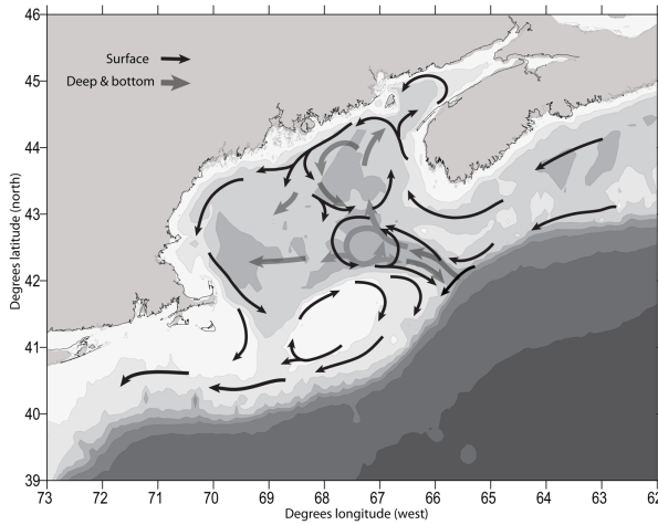
Figure 2. Schematic representation of the main features of surface currents in the upper 75 m and deep and bottom currents below 75 m in the Gulf of Maine region (after Brooks 1985; Pettigrew and Hetland 1995; and Beardsley et al. 1997).
