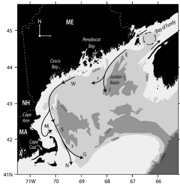
Fig. 1. Schematic of the Maine Coastal Current. Branch points are located at (1) Penobscot Bay, (2) Cape Ann, and (3) Great South Channel. Seven segments of the current are indicated: (E)astern, (J)ordan, (W)estern, (M)assachusetts, (S)tellwagen, (N)antucket, and (G)eorges Bank. Figure redrafted from Lynch et al. (1997) with the addition of the Bay of Fundy gyre system as drawn in Godin (1968). Dashed white lines denote state boundaries of Maine (ME), New Hampshire (NH), and Massachusetts (MA).
