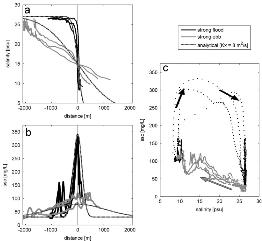
Fig. 5. Salinity and suspended sediment front during calm conditions. (a) Spatial distribution of salinity during strong floods and strong ebbs; (b) spatial distribution of suspended sediment during strong floods and strong ebbs. The salinity and sediment distributions were calculated from time series at Frame A assuming advection by the local velocity; each day's observation was plotted relative to the location of the 15 psu isohaline, and dashed lines represent analytical dispersion with K_x = 8 \text{ m}^2/\text{s} ; (c) Suspended sediment as a function of salinity; arrows indicate progression of time/distance.
