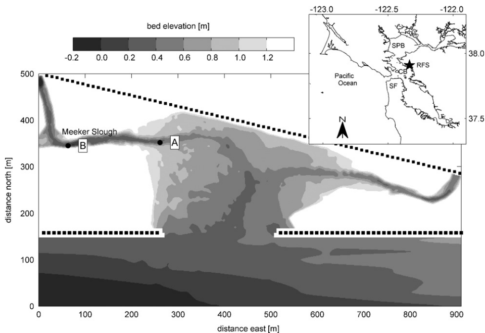
Fig. 1. Intertidal mudflat bathymetry at Richmond Field Station (RFS, ★) on the eastern shore of Central San Francisco Bay (CB) and south of San Pablo Bay (SPB). Instrument frames (A and B) and breakwaters (■) are marked; salt marsh area is white.
