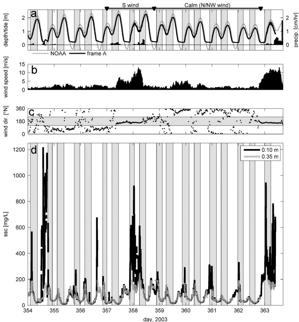
Fig. 2. Suspended sediment observations in the mudflat channel. (a) Water surface in the channel, tidal stage at NOAA station, and precipitation; (b) wind speed; (c) wind direction; and (d) suspended sediment concentration 0.10 and 0.35 m above the bed at Frame A. Forcing periods shown in greater detail are noted above (a): calm conditions (Fig. 4), wind from the south (Fig. 7).
