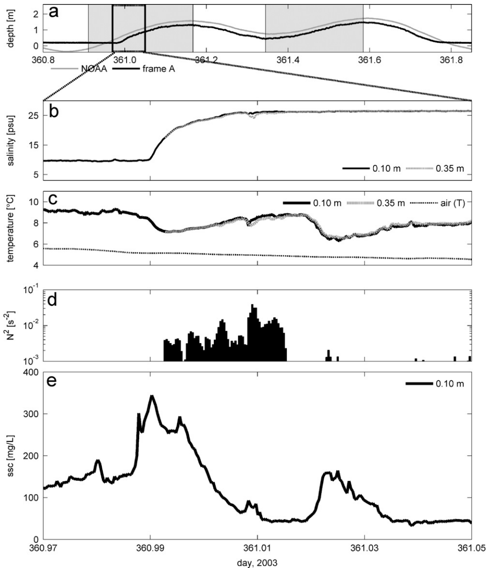
Fig. 6. Detail of secondary peak in suspended sediment during strong floods. (a) Depth and tidal stage for the entire inundation, with the period in the lower panels highlighted. (b) Salinity 0.10 and 0.35 m above the bed; (c) temperature 0.10 and 0.35 m above the bed along with air temperature; (d) stratification; (e) suspended sediment 0.10 m above the bed.
