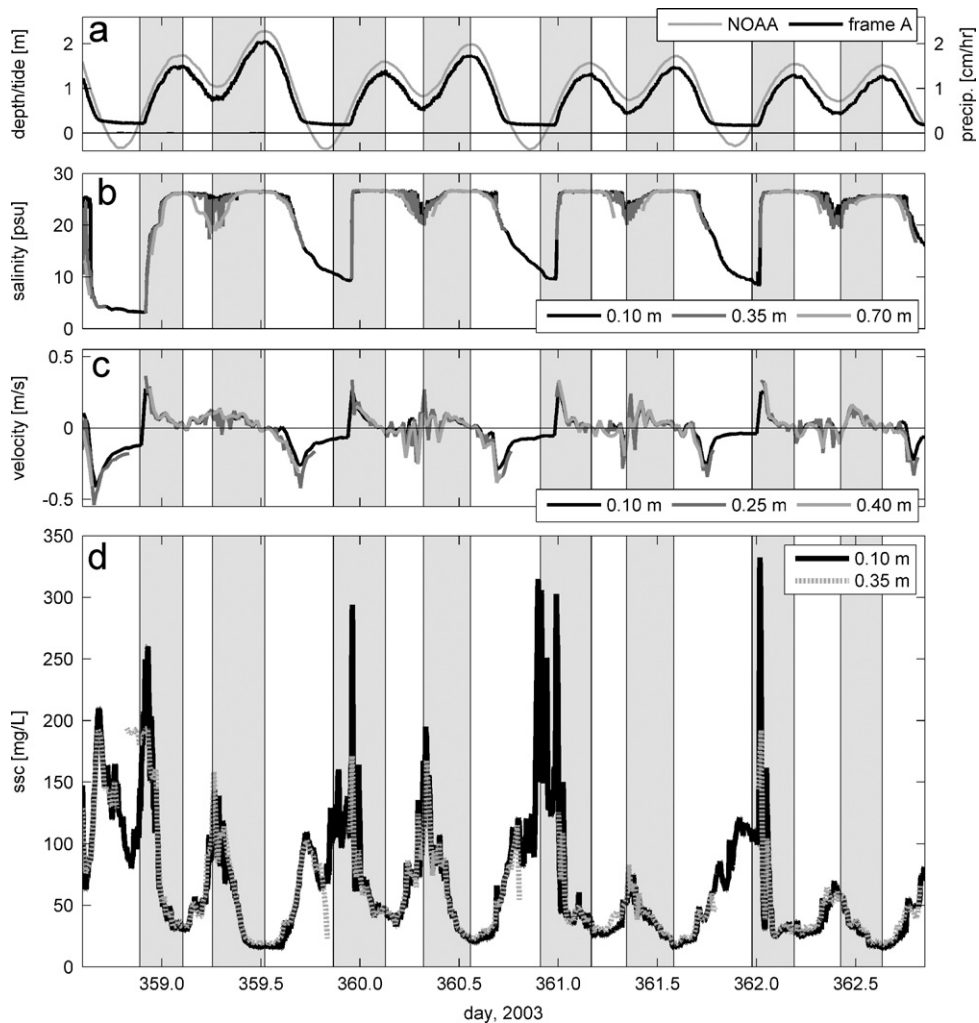
Fig. 4. Conditions in mudflat channel during calm weather conditions. (a) Water surface in the channel, tidal stage, and precipitation; (b) salinity 0.10, 0.35, and 0.70 m above the bed on Frame A; (c) along-channel velocity 0.10, 0.25, and 0.40 m above the bed; (d) suspended sediment concentration 0.10 and 0.35 m above the bed.
