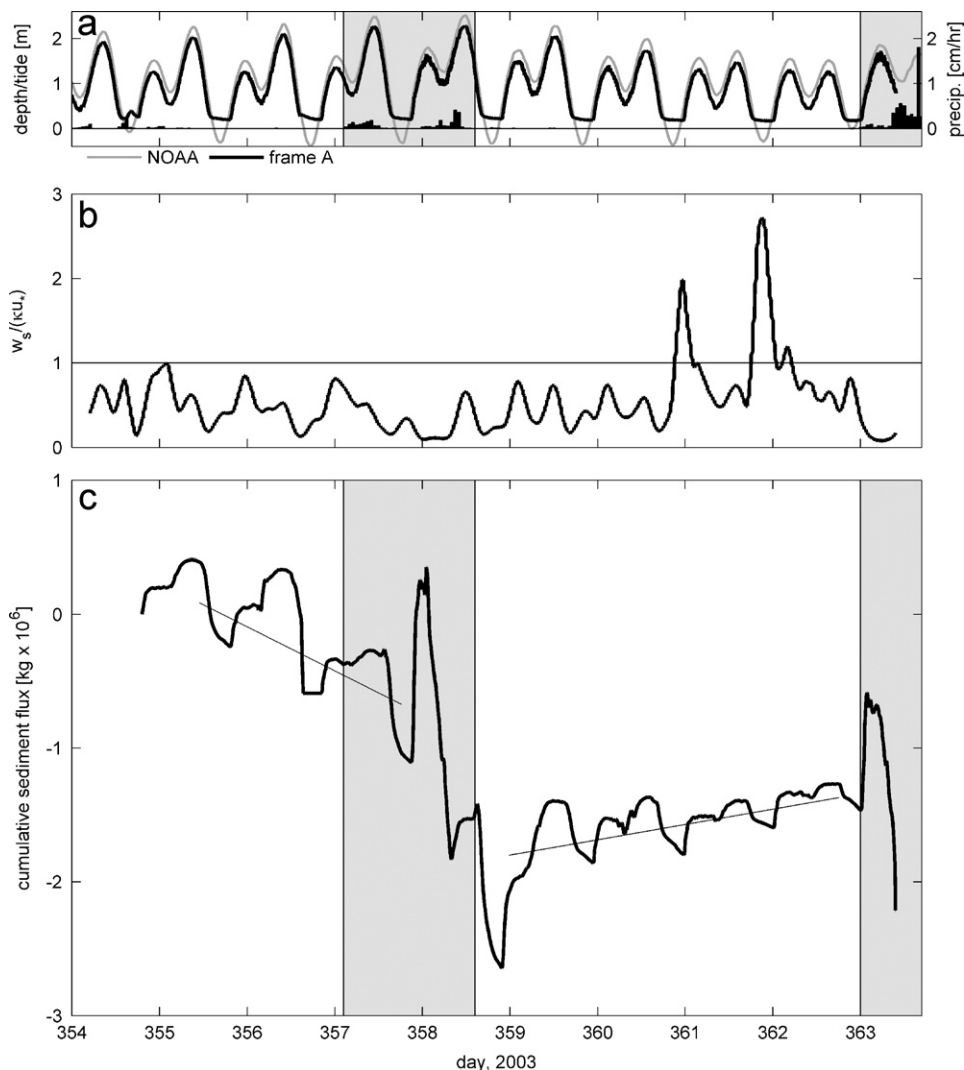
Fig. 9. Rouse number and cumulative sediment flux. (a) Water surface, tidal stage, and precipitation, with periods of precipitation highlighted gray; (b) Rouse number, P = w_s / (\kappa u_*) ; (c) cumulative sediment flux in the channel from the beginning of the deployment, with positive slope for onshore transport and negative slope for offshore transport.
