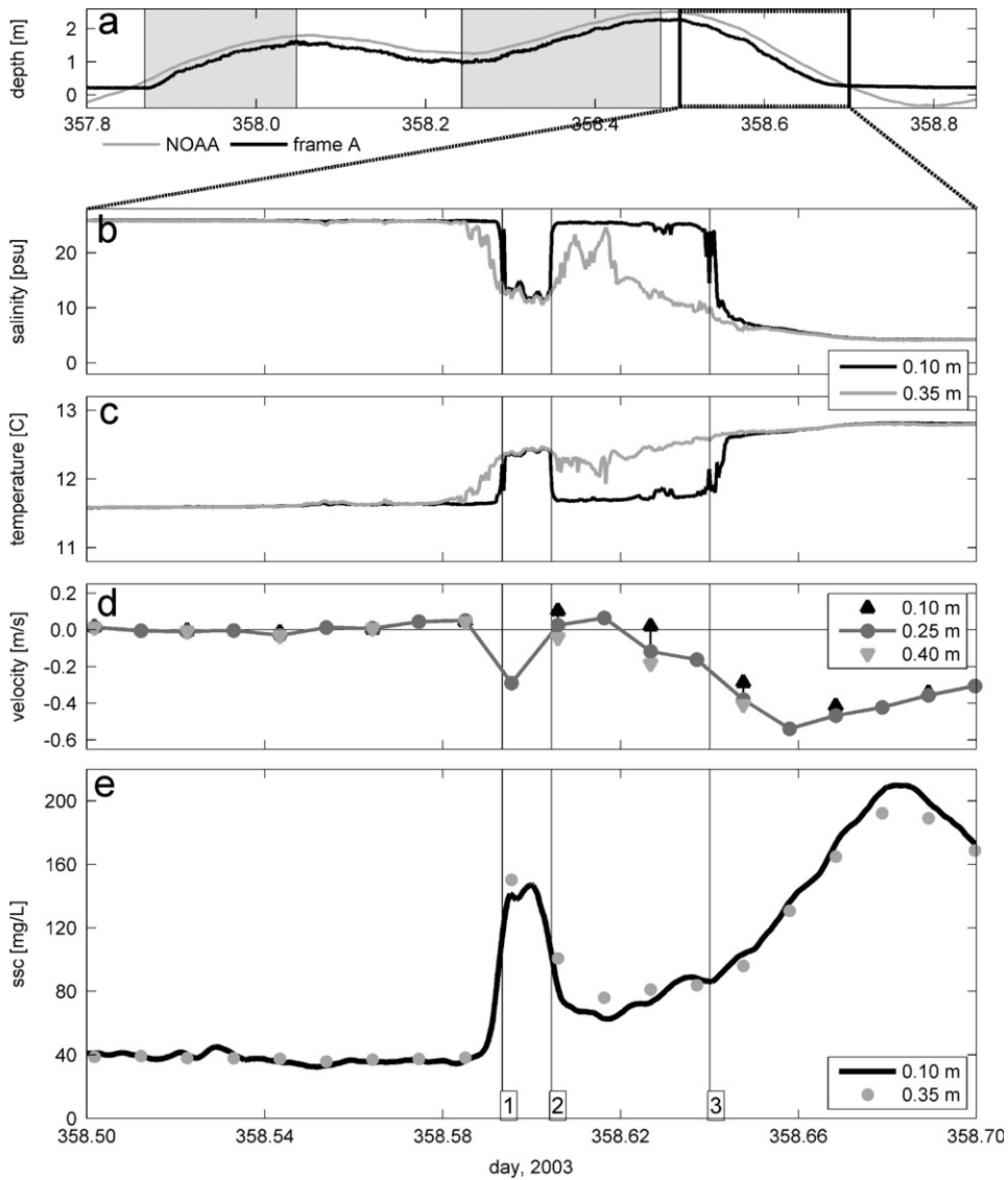
Fig. 8. Conditions in mudflat channel after moderate precipitation. (a) Depth and tidal stage for the entire inundation, with the period in the lower panels highlighted; (b) Salinity 0.10 and 0.35 m above the bed; (c) temperature 0.10 and 0.35 m above the bed; (d) along-channel velocity 0.10, 0.25, and 0.40 m above the bed; (e) suspended sediment 0.10 and 0.35 m above the bed.
