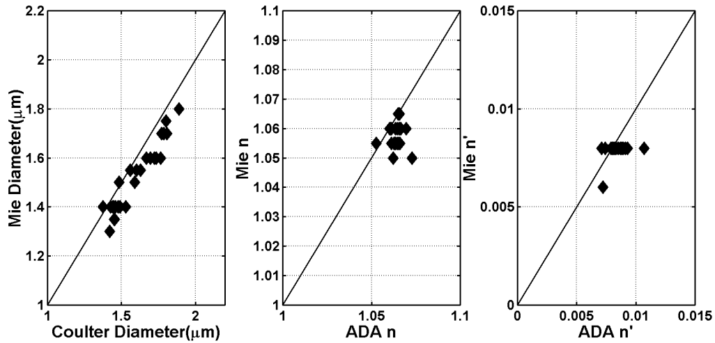
Figure 4. Comparison of cell properties estimated using the modified MBLT approach with independent estimates based on direct measurements of Micromonas pusilla sampled over a diel cycle.
