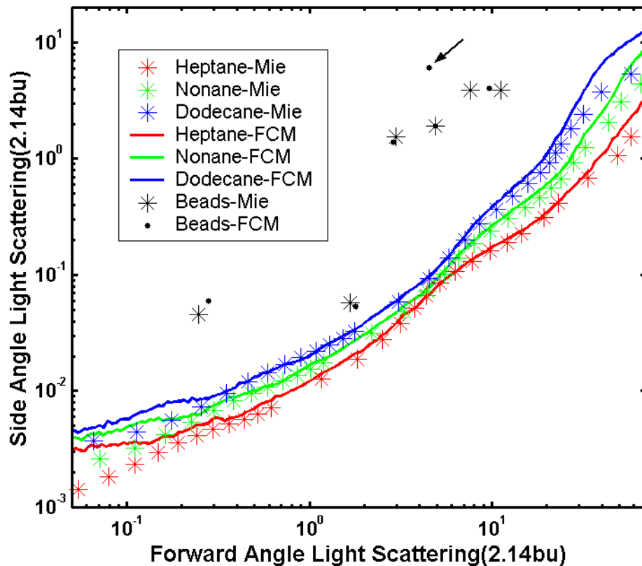
Figure 1. A comparison of theory-based estimates (stars) and flow cytometric measurements (lines and dots) of forward and side scattering for beads and oil dispersions. Several bead types were used in this comparison, including 0.66, 2.9, 3.79, 5.2, and 6.2 micron polystyrene beads and 1.58 micron silica beads. An arrow has been placed next to the 5.2 micron polystyrene bead which is the most poorly fit by this optimization. Oil dispersions of heptane, nonane, and dodecane are shown.
