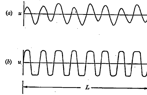
FIGURE 5. Evolution of amplitude function u(\xi, t) from the initial state.
