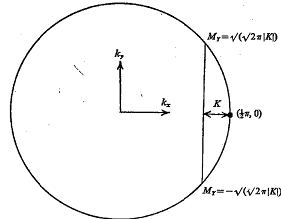
FIGURE 3. The circle k_x^2 + k_y^2 = \pi^2/2 , showing points of maximum oblique roll growth.
