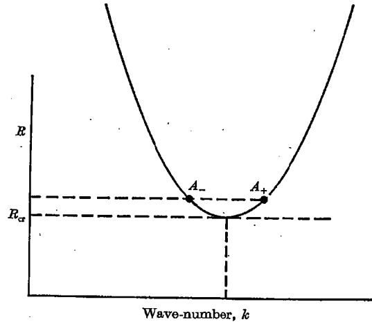
FIGURE 1. Stability diagram showing finite bandwidth of modes.
