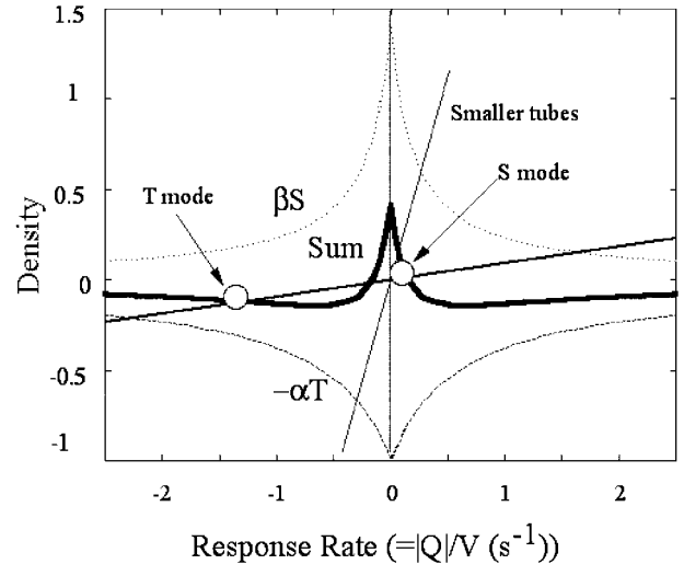
Figure 2. Curves expressing the behavior of Stommel’s conceptual box model. The hyperbolae labeled \beta S and -\alpha T are found ((4) and (5)) using a linear equation of state and parameters of the laboratory experiment. They indicate density deviations ( \rho - \rho_0 ) due to salinity and temperature, respectively. Their sum is shown by the dark curve. The dark straight line represents linear dynamics of flow. Intersection at the two circles gives two stable modes. The third intersection is unstable. For tubes with greater flow resistance (light straight line), only the S-mode is possible.
