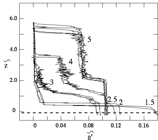
Figure 7. Density profiles after the experiment sketched in Figure 6 has achieved a steady state. The numbers near the curves denote values of \bar{H} . The vertical scale \bar{z} has been nondimensionalized by the channel height D = 0.1 m. The dashed line and the vertical origin give the level of the floor of the channel. Assorted profiles for the same values of \bar{H} were taken more than 5 min apart.
