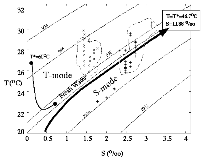
Figure 13. Temperature–salinity diagram of the experimental measurements and overmixed theory. The + symbols indicate values found in the S-mode, the x symbols indicate values found in the T-mode, and the flows in the multiple equilibrium range are enclosed by a dashed curve. The clusters for each mode are distinctly separated. This signifies that a Stommel transition separates the two modes. The S-mode branch from theory is shown on the right as a wide curve that closely follows the density of the reservoir (freshwater at 20^\circ\text{C} ). The branch extends off the diagram to the upper right to the values shown in the box. The T-mode branch from theory is shown on the left as a curve that starts at the value T^* = 27.04^\circ\text{C} shown by the solid dot, spirals clockwise, and approaches smaller S and larger T for increasing T^* . The values of the calculation at T^* = 60^\circ\text{C} terminate the branch shown in this figure although this branch extends for all larger values of T^* . The experimental data are for 29 \leq T^* \leq 36^\circ\text{C} .
