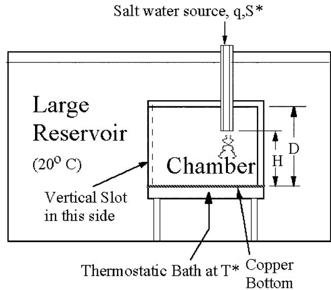
Figure 11. Sketch of the doubly driven apparatus with partial mixing.
