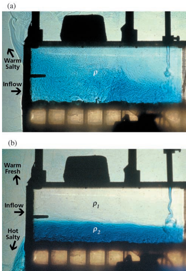
Figure 12. (a) Photograph of a shadowgraph of the chamber, sketched in Figure 11, in the T-mode. (b) In the S-mode. The arrows indicate the flow direction through the slot.
