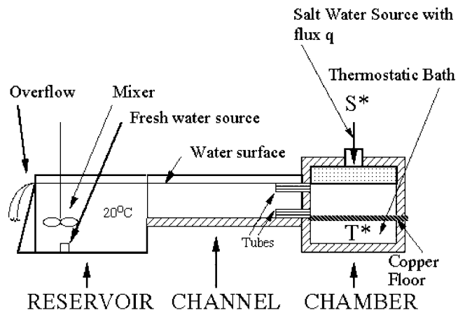
Figure 1. Sketch of the ‘‘inverse estuary’’ laboratory apparatus. Salt water of salinity S^* is pumped into the top of the chamber, which is heated from below at temperature T^* . Tubes at the top and bottom side of the chamber allow circulation into a channel. The other end of the channel is connected to a constant temperature freshwater reservoir on the left. The hatched region indicates thermal insulation.
