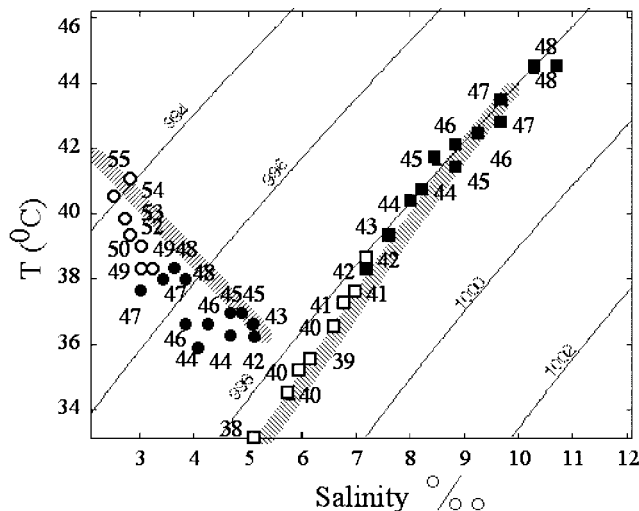
Figure 3. A T/S diagram showing experimental values of the salinity and temperature of water in the chamber in a range of multiple equilibria laboratory experiments where the external volume flux q and salinity S^* are held constant while T^* is varied. Contours indicate density (in MKS). The squares indicate mixed-water properties when the system is in the S-mode, and the circles when it is in the T-mode. The solid symbols denote the points with two stable modes. The value of T^* is shown next to each symbol, located to the right for experiments with a channel and to the left without the channel. The hatched broad lines are theoretical predictions using (3)–(6).
