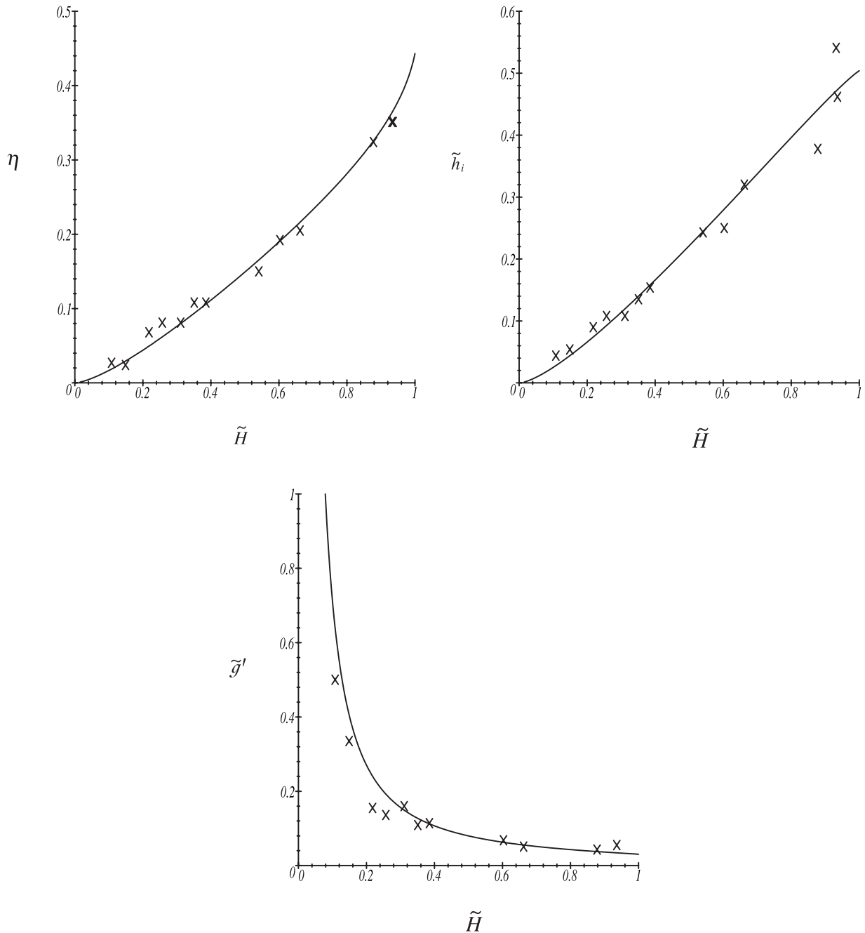
Figure 5. The relationship between the dimensionless depth \tilde{H} of a single freshwater source and (a) the mixed-layer thickness \eta in the contraction, (b) the mixed-layer thickness \tilde{h}_i in the chamber, and (c) the reduced gravity \tilde{g}' . The curves are the numerical solutions ( c = 0.22 ) and the crosses are experimental results.
