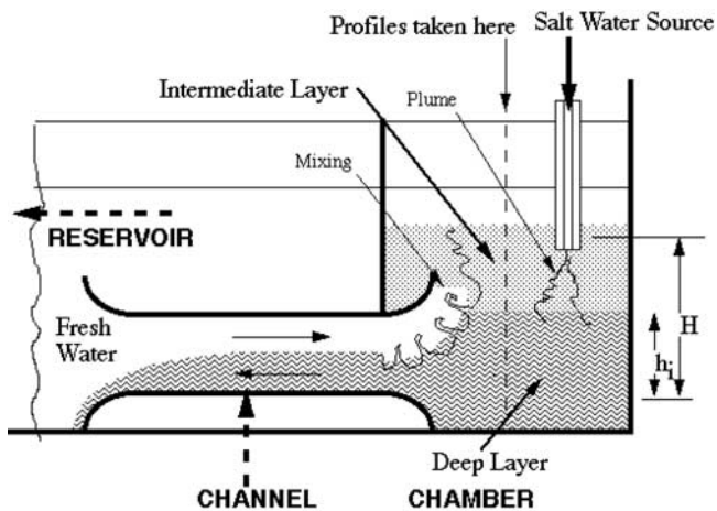
Figure 6. Sketch of the apparatus to investigate very large mixing.
