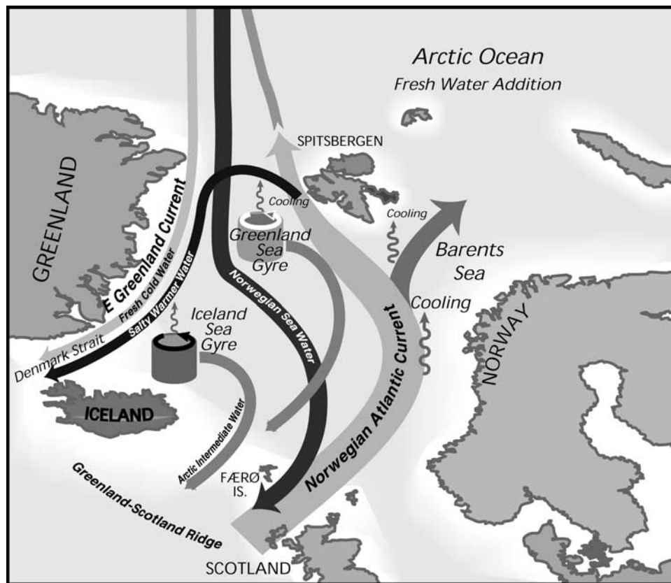
Figure 15. Sketch of the major currents between the North Atlantic and the Nordic Seas [after Mauritzen, 1996a, 1996b].
