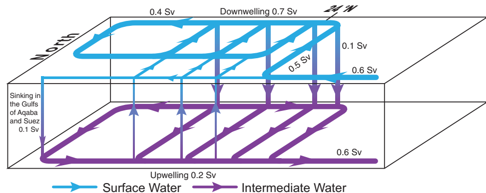
Figure 14. Schematic for the three-dimensional overturning circulation in the northern Red Sea. Most (0.5 Sv) of the surface western boundary current (0.6 Sv) crosses the basin at around 24^{\circ}\text{N} , and then either sinks along the eastern boundary at the crossing latitude (0.1 Sv) or switches to an eastern boundary current (0.4 Sv) and sinks along the eastern boundary through a cyclonic recirculation. The downwelled water at the intermediate depth is transported to the western boundary either through direct cross-basin flows or a rim current along the boundary. Meanwhile, the sinking along the eastern boundary is enhanced by a weaker cross-basin overturning circulation produced by the upwelling along the western boundary (0.2 Sv). A small portion of the western boundary current (0.1 Sv) sinks in the Gulf of Aqaba and Gulf of Suez and contributes to the intermediate and deep water.
