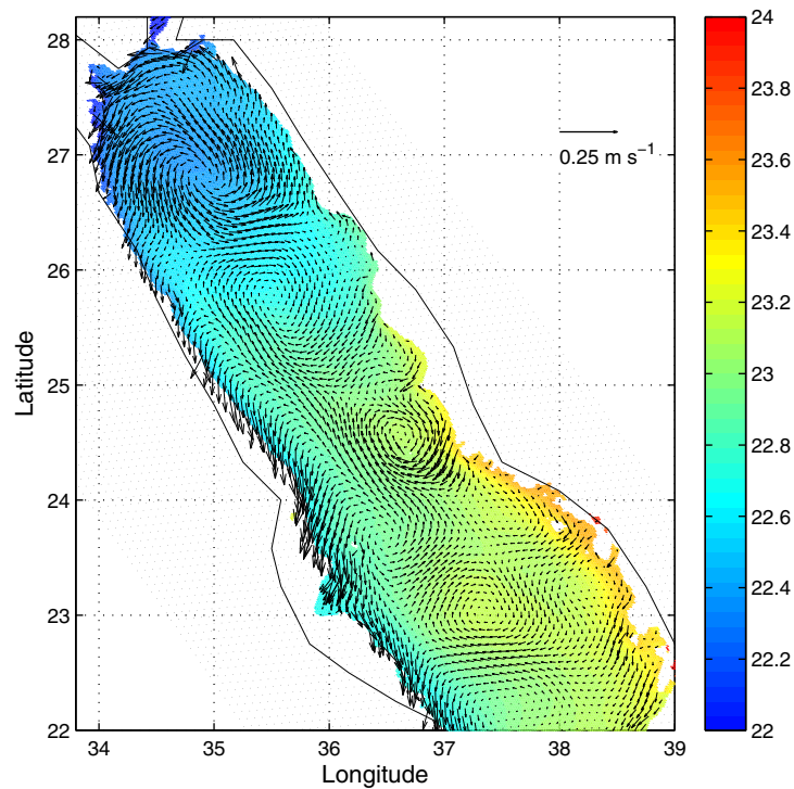
Figure 13b. Fields of current and temperature ( ^{\circ}\text{C} ) at 160 m in February for the climatological mean.
