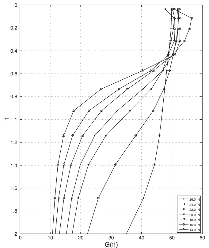
Figure 16. Scaled buoyancy profiles in February 1980, using h = 160 m and B_0 = 2.0 \times 10^{-8} \text{ m}^2 \text{ s}^{-3} .
