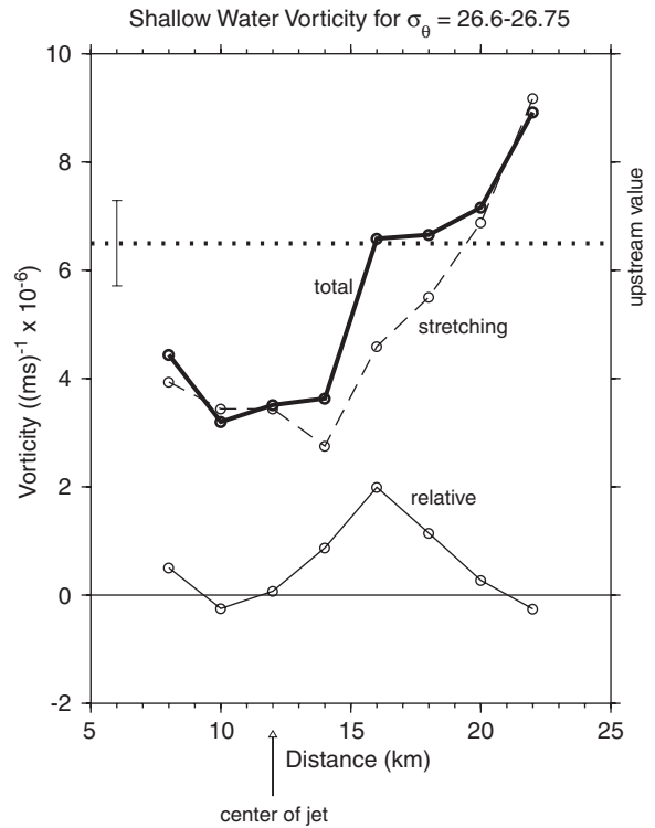
Fig. 9. Terms of the shallow-water vorticity at the mouth of Barrow Canyon, averaged over the density layer \sigma_\theta = 26.6\text{--}26.75 (see Eq. (3)). The center of the deep jet is marked by the arrow. The average value of Q at the head of the canyon ( 18\text{ km} < y < 28\text{ km} ) is shown by the thick dashed line (standard deviation indicated by the bar).
