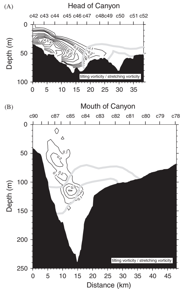
Fig. 7. Vertical sections of the ratio of tilting vorticity to stretching vorticity. The thick gray lines are as in Fig. 6. (A) Head of Barrow Canyon and (B) mouth of Barrow Canyon.
