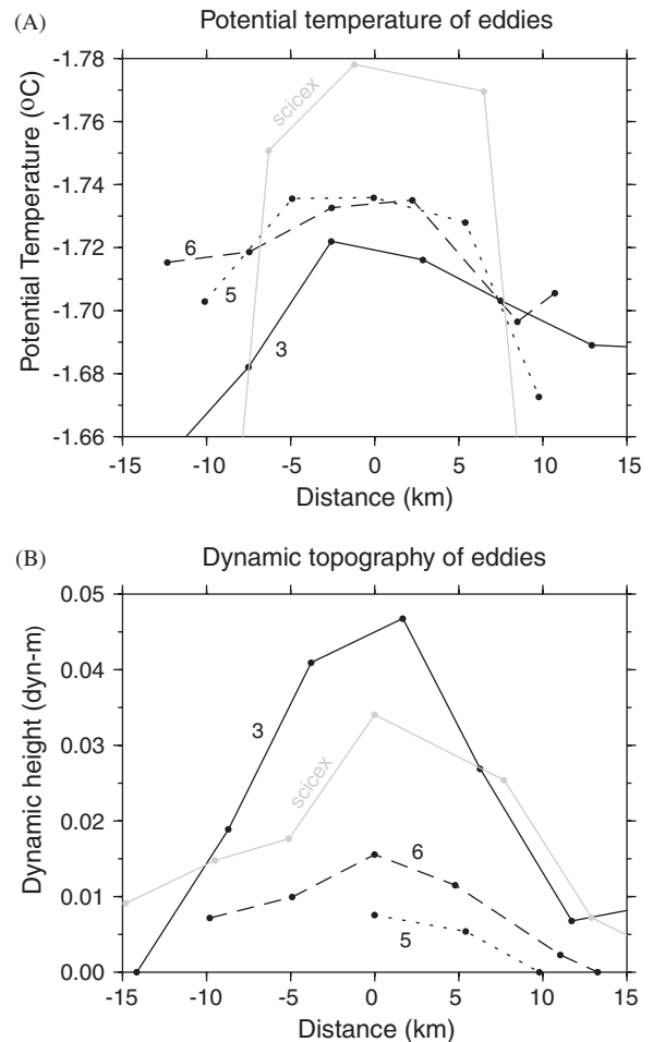
Fig. 13. Properties of the eddies observed on Sections 3, 5 and 6 (black lines), as well as the Scicex Eddy (gray line). The features have been aligned horizontally at the origin of the abscissa. (A) Potential temperature (°C) averaged within the density layer of the eddy (see Table 1). (B) Dynamic height of the eddy relative to its central pressure: Section 3 (30 db relative to 140 db); Section 6 (50 db relative to 115 db); Section 5 (50 db relative to 115 db); Scicex 97 (60 db relative to 200 db). For Section 5, only the offshore side of the eddy is shown (since it is still pinching off).
