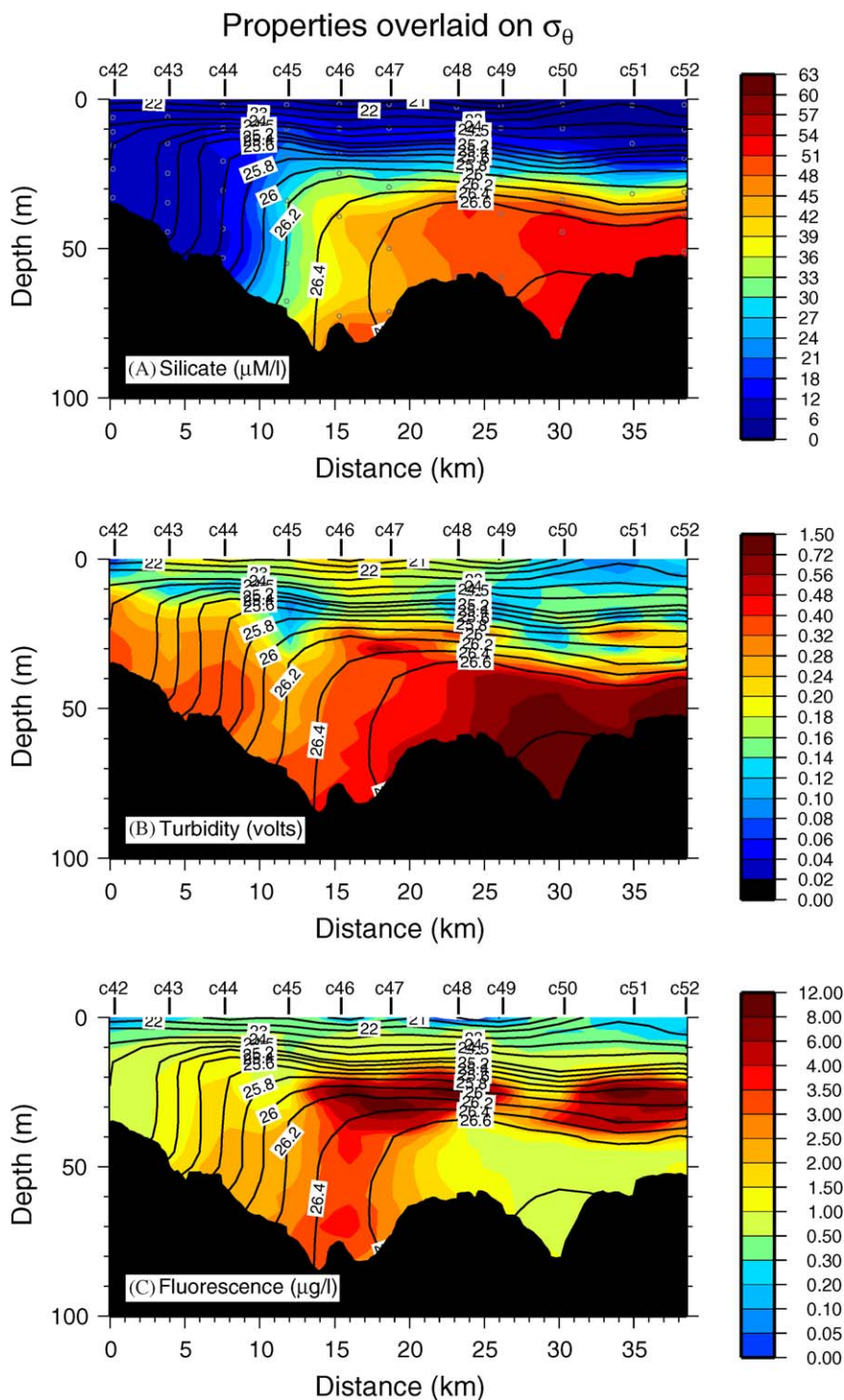
Fig. 5. Vertical sections at the head of Barrow Canyon. The contours are potential density ( \text{kg/m}^3 ): (A) Silicate (color, \mu\text{M/l} ); Water sample locations are indicated by the circles, (B) turbidity (color, volts) and (C) fluorescence (color, \mu\text{g/l} ).
