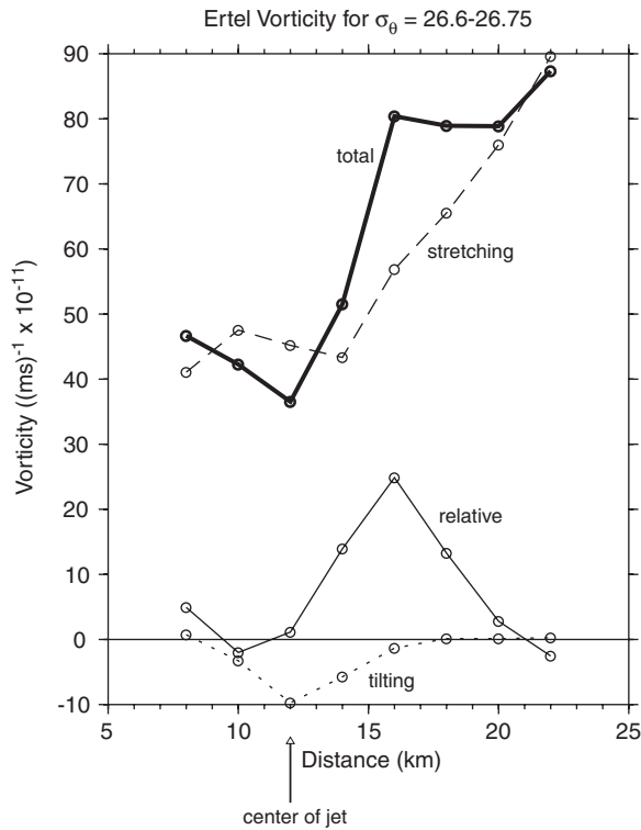
Fig. 8. Terms of the Ertel vorticity at the mouth of Barrow Canyon, averaged over the density layer \sigma_\theta = 26.6\text{--}26.75 (see Eq. (2)). The center of the deep jet is marked by the arrow.
