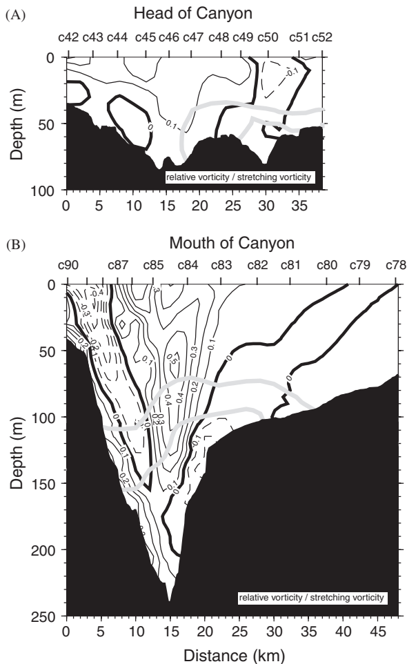
Fig. 6. Vertical sections of the ratio of relative vorticity to stretching vorticity (see Eq. (2)). Solid contours are cyclonic vorticity, dashed contours are anti-cyclonic. The thick gray lines show the density layer chosen for the vorticity analysis ( \sigma_\theta = 26.6\text{--}26.75 ). (A) Head of Barrow Canyon and (B) mouth of Barrow Canyon.
