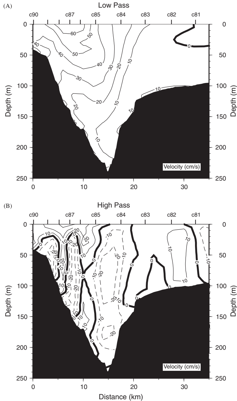
Fig. 2. (A) Filtered absolute geostrophic velocity (cm/s) at the mouth of Barrow Canyon (see text for a description of the filtering technique). Positive velocities (solid contours) are out of the canyon, negative velocities (dashed contours) are into the canyon. (B) High-passed residual velocity (same sign convention for positive and negative velocities).
