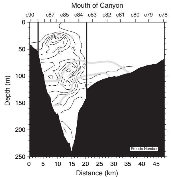
Fig. 10. Vertical section of Froude number (see text for definition) at the mouth of Barrow Canyon. The thick gray lines are as in Fig. 6. The vertical black lines denote the artificial edges of the canyon used to solve Eq. (4).
