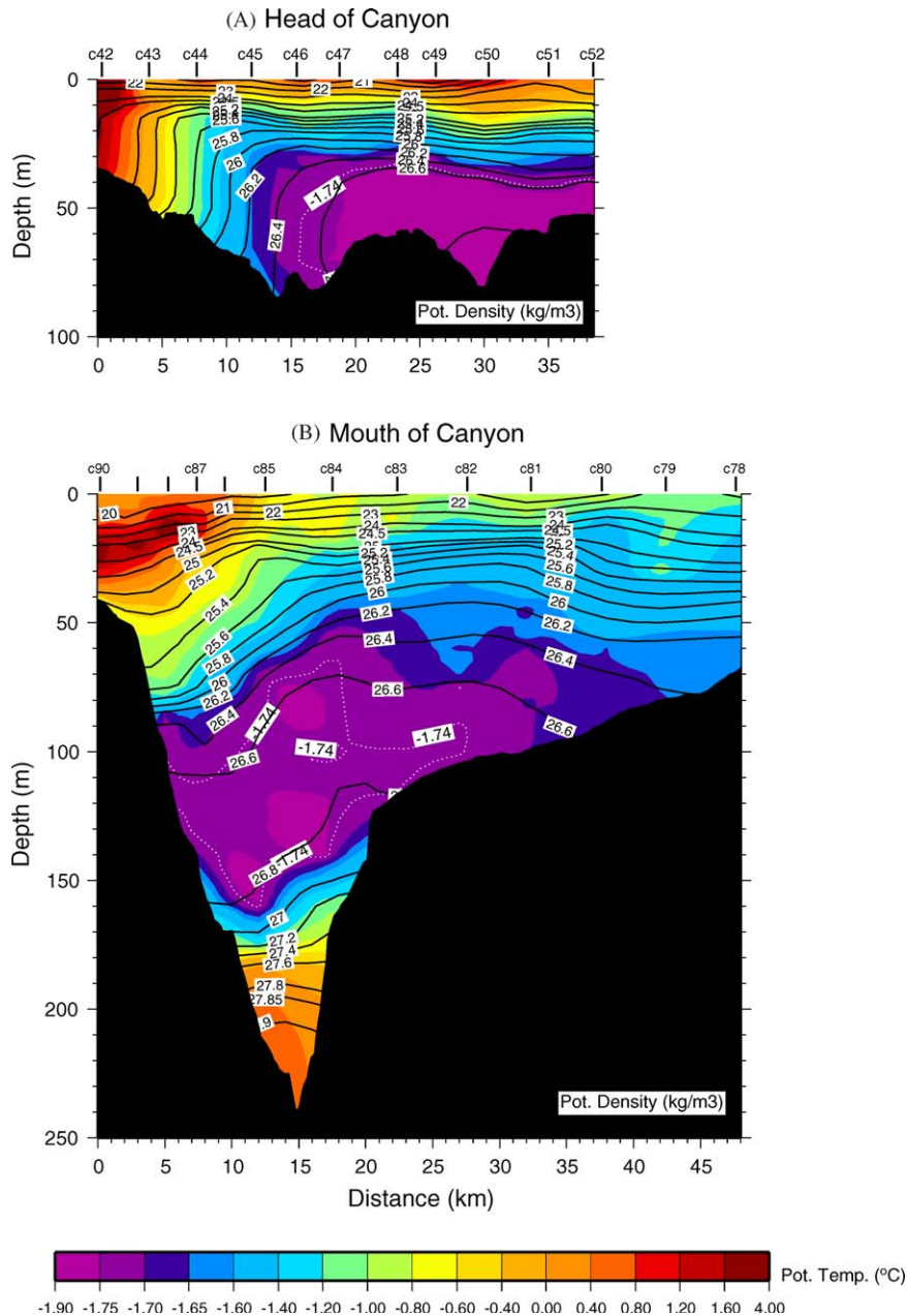
Fig. 4. Vertical sections of potential density (contours, kg/m 3 ) overlaid on potential temperature (color, °C). (A) Head of Barrow Canyon and (B) mouth of Barrow Canyon.
