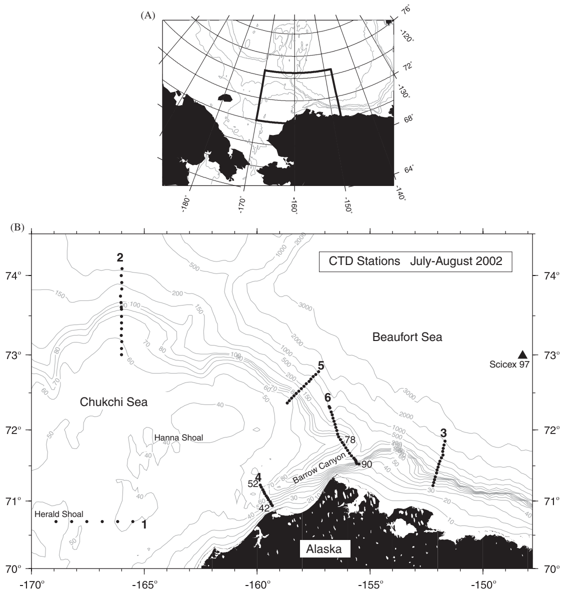
Fig. 1. (A) Study area in the Eastern Chukchi and Western Beaufort Seas. (B) Enlarged view of study area, showing the hydrographic stations occupied by USCGC Polar Star in summer 2002. The survey consisted of six sections. Station numbers are included on the two Barrow Canyon sections: the head of the canyon (stations 42–52) and the mouth of the canyon (stations 78–90). The location of the eddy observed during the 1997 Scicex expedition is indicated by the triangle.
