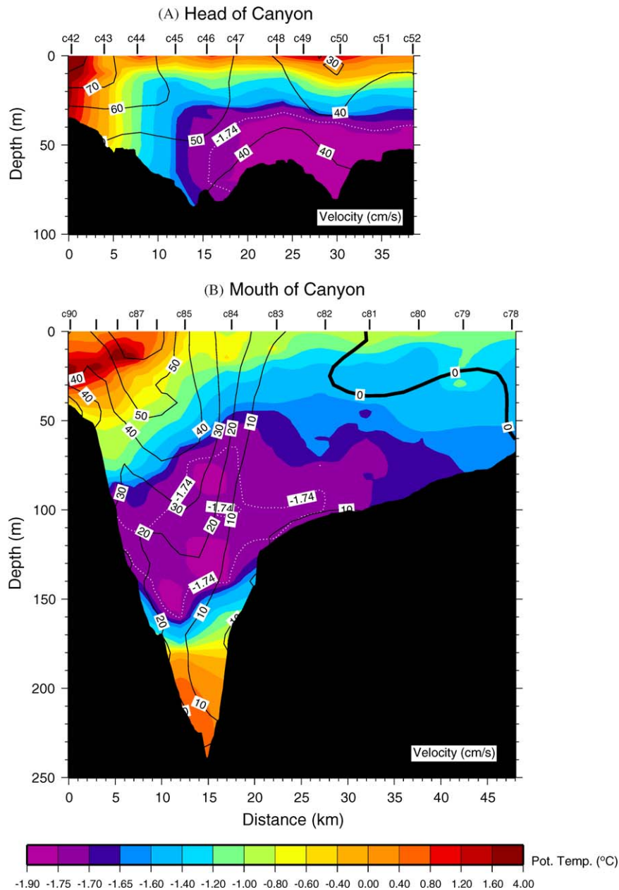
Fig. 3. Vertical sections of filtered velocity (contours, cm/s) overlaid on potential temperature (color, °C). The white dashed line is the -1.74 °C isotherm. (A) Head of Barrow Canyon and (B) mouth of Barrow Canyon.
