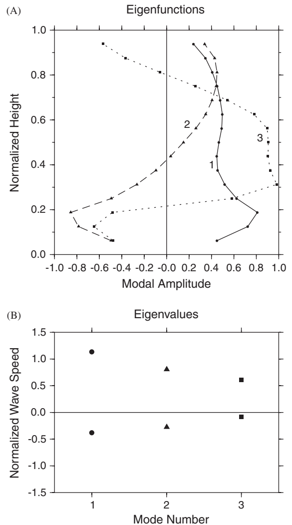
Fig. 11. Solution to the modified Taylor–Goldstein equation for the mouth of Barrow Canyon: (A) vertical structure of the first three dynamical modes and (B) wave speeds of the first three modes (symbols the same as in (A)).
