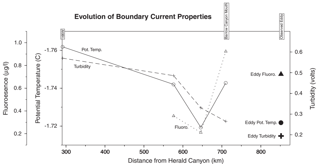
Fig. 14. Downstream evolution of boundary current properties, averaged within the density layer \sigma_\theta = 26.65\text{--}26.8 . Also shown are the properties at the core of the eastern eddy (see Table 1).
