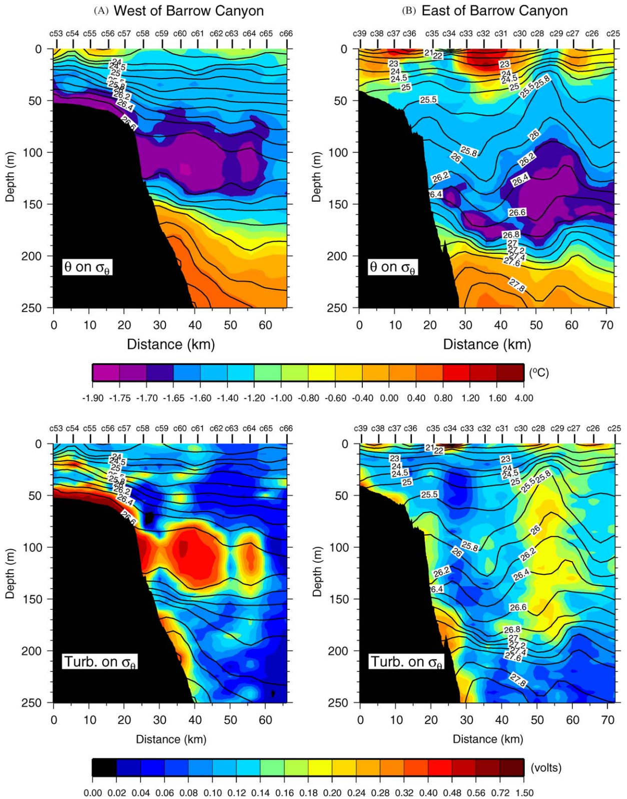
Fig. 12. Vertical sections of properties overlaid on potential density ( \text{kg/m}^3 ). The top panel shows potential temperature (color, ^{\circ}\text{C} ); the bottom panel shows turbidity (color, volts). (A) Section 5, west of Barrow Canyon and (B) Section 3, east of Barrow Canyon.
