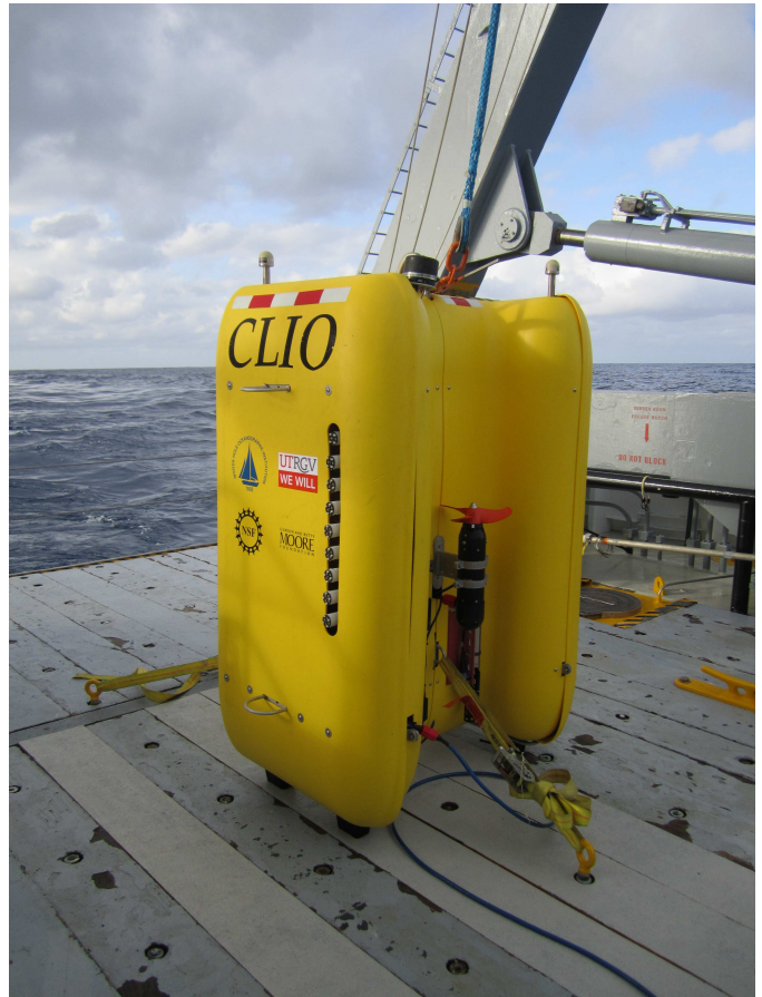
Fig. 1. Clio aboard the RV Atlantic Explorer in April 2018. The intake ports for one of two SUPRs are visible on the right-hand side of the panel bearing the vehicle’s name. One of two thrusters is visible between the hulls.
