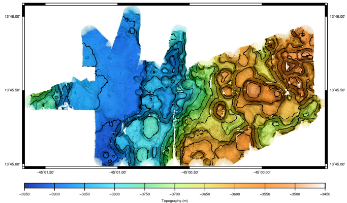
Fig. 7. Multibeam bathymetry from sentry474, baseline processing identical to that in Fig. 6 only with USBL artificially withheld to simulate the effect on map quality of leaving Sentry untended for the majority of its dive. The maps are qualitatively indistinguishable.
