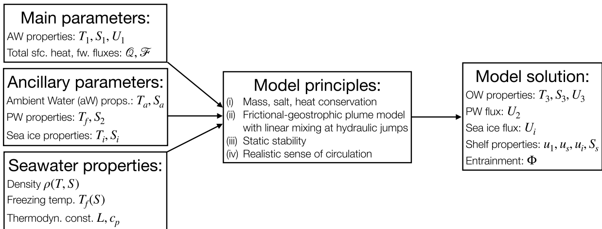
FIG. 2. (top) Schematic of the conceptual polar overturning model. The sign convention is that positive volume fluxes are toward the right. For realistic solutions \{U_2, U_3, U_i, u_s, u_i\} < 0 and u_1 > 0 , as the arrows show. The topographic bump at section A (nominally, the Fram Strait and Barents Sea Opening) is for illustrative purposes: the dashed line represents the Antarctic case. (bottom) Flowchart showing the model parameters, principles, and output variables. Table 1 defines the symbols.
