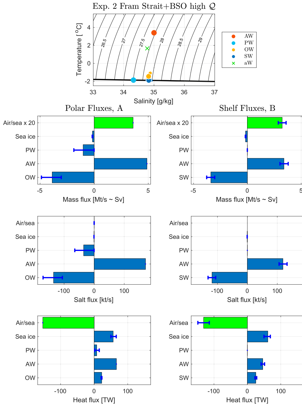
FIG. 5. As in Fig. 4, but for experiment 2. This solution has similar mass and salt fluxes to experiment 1 shown in Fig. 4, but weak entrainment ( \Phi \approx 0.13 ), strong shelf circulation, and cold OW. The total ocean heat loss flux \mathcal{Q} is 33% larger than for experiment 1. Notice the heat flux abscissa limits differ from Fig. 4.
