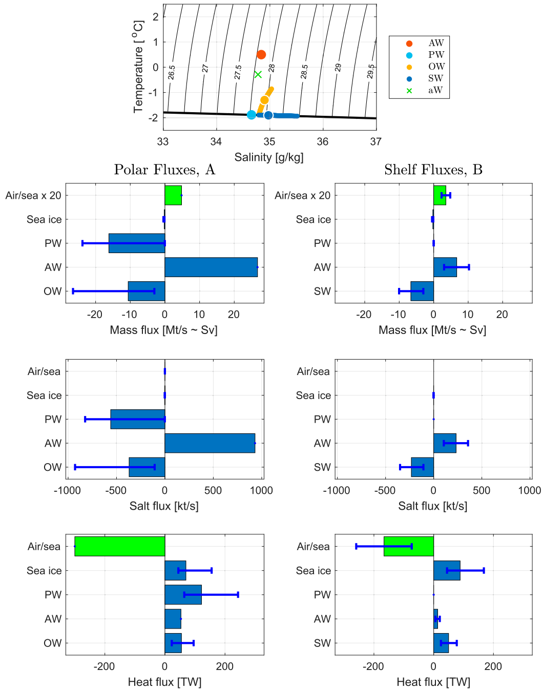
FIG. 9. As in Fig. 4, but for experiment 6 for the Antarctic.
