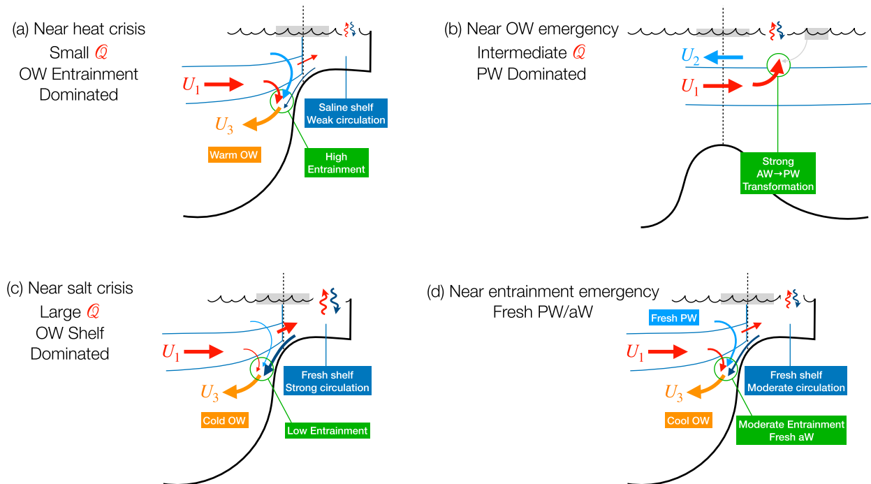
FIG. 10. Schematics of the four main solution modes: (a) heat crisis for small Q (like experiment 1), (b) OW emergency for intermediate Q (like experiment 6 and the middle of experiment 3), (c) salt crisis for large Q (like experiment 2), and (d) entrainment emergency for fresh PW and/or aW (like the small PW salinity end of experiment 5). These main solutions are determined by the forcing, indicated by the ocean heat loss flux Q (Figs. 6 and 8), and by the aW salinity (Fig. S2). See also Fig. S3.
