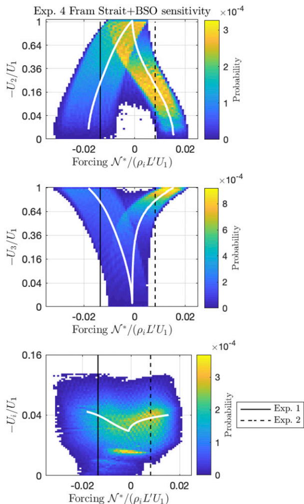
FIG. 8. Results for experiment 4 for the Arctic. Normalized distributions of U_2 , U_3 , and U_i against the forcing parameter N^* = Q + L'F + (1 - S_i/S_1) + c_p \rho_i (S_i/S_1 - 1) T_1 U_1 for many solutions with different parameters \{F, Q, U_1, T_1, S_1\} (see Table 2). In each case, the distribution is taken of the solutions with entrainment closest to the mean entrainment, like the bars in Fig. 4. The solid and dashed vertical lines indicate experiments 1 and 2, shown in Figs. 4 and 5, respectively. The white curves show the results from experiment 3, as in Fig. 6, which are a subset of the results from experiment 4. There are 525 199 valid solutions in experiment 4.
