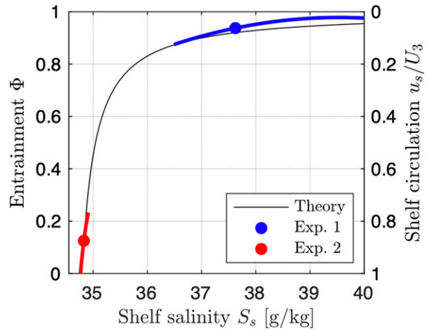
FIG. 7. Trade-off between entrainment \Phi and shelf salinity S_s for fixed OW flux. Strong (weak) entrainment implies weak (strong) shelf circulation u_s , from (6). Results from experiments 1 and 2, including the range of possible solutions, are shown. The theory curve is from (12).
