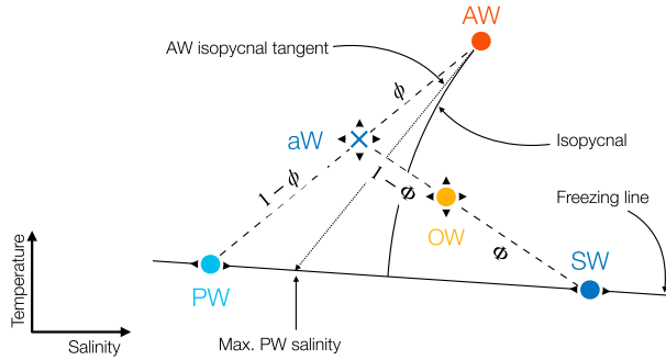
FIG. 3. Schematic of the processes affecting OW properties. The Atlantic Water (AW) properties are specified. The Polar Water (PW) properties are freezing temperature and salinity less than the maximum value given by the dotted line tangent to the AW isopycnal. The ambient Water (aW) properties are a mixture of PW and AW determined by \phi . The Overflow Water (OW) properties are a mixture of aW and SW determined by entrainment \Phi .
