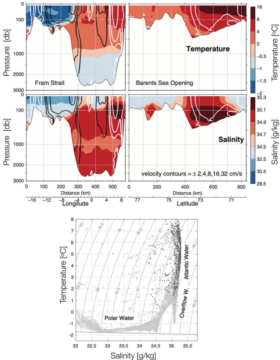
FIG. 1. (top) Observations of temperature, salinity, and normal geostrophic current across the Fram Strait and Barents Sea Opening. Modified from Klinger and Haine (2019) and based on results from Tsubouchi et al. (2012) . (bottom) Temperature and salinity data from Fram Strait in August 2002 (light gray) and from the Barents Sea Opening in August 2017 (dark gray; from the World Ocean Database, Boyer et al. 2018 ).
