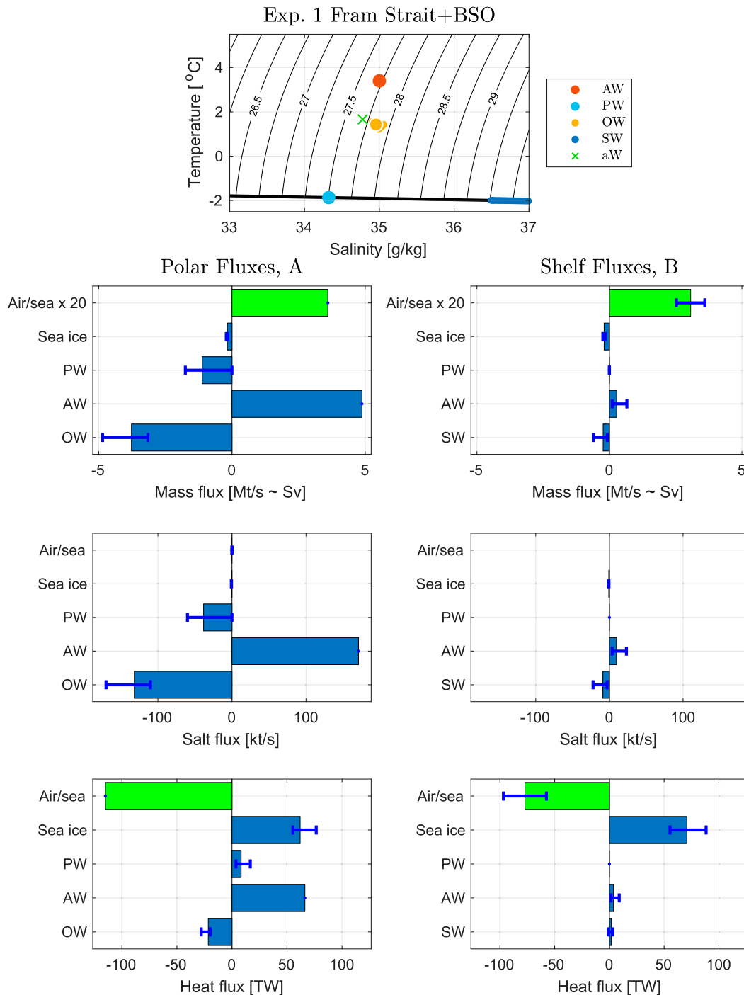
FIG. 4. Results for experiment 1, with parameters appropriate for the Arctic (Fram Strait and Barents Sea Opening, BSO). (top) Temperature–salinity properties, as in Fig. 3. Curved black contours are the density anomaly \rho(T, S) - 1000 \text{ kg m}^{-3} , and the thick black line is the freezing temperature. (bottom) The left (right) column of panels show mass, salt, and heat fluxes crossing section A (B) in Fig. 2. The individual terms in (S1) and (S2) are shown with the horizontal bars. The blue error bars indicate the range of possible solutions (see text). This solution is entrainment dominated with \Phi \approx 0.94 , warm OW, and a weak shelf circulation.
