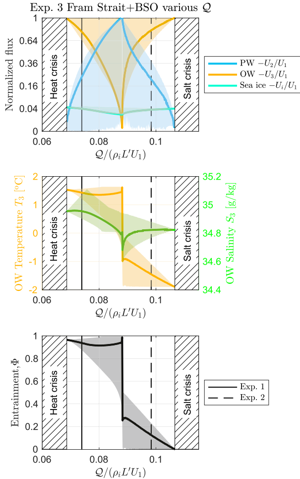
FIG. 6. Results for experiment 3 for the Arctic. (top) The normalized volume fluxes U_2 , U_3 , and U_i . (middle) The OW properties T_3 and S_3 . (bottom) The entrainment \Phi . In each case, the abscissa is the normalized ocean heat loss flux Q . The solid and dashed vertical lines indicate experiments 1 and 2, shown in Figs. 4 and 5, respectively. The hatched regions indicate no solutions are possible because U_2 \not\leq 0 ; see text for details.
