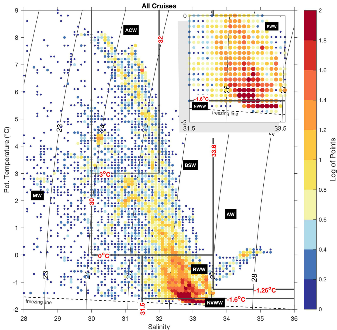
Fig. 3. Temperature-salinity diagram for all of the DBO5 occupations. The color corresponds to the frequency of occurrence of water within bins of 0.1^{\circ}\text{C} in temperature by 0.1 in salinity. The water mass boundaries are indicated by the grey lines. The inset shows an enlarged view of the winter water. The different water masses are: NVWW = newly ventilated winter water; RWW = remnant winter water; BSW = Bering Summer Water; ACW = Alaskan Coastal Water; MW = meltwater/runoff; and AW = Atlantic water. (For interpretation of the references to color in this figure legend, the reader is referred to the web version of this article.)
