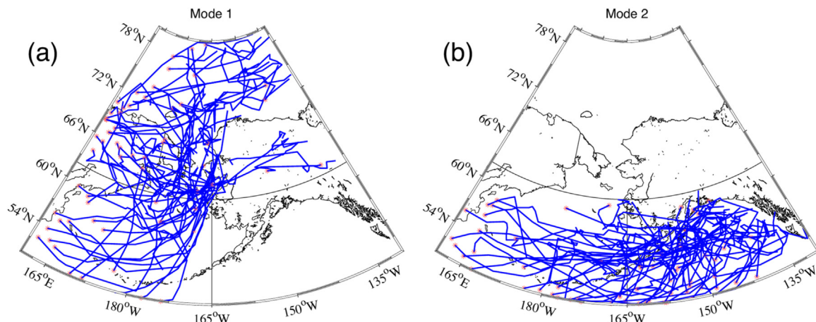
Fig. 14. Two dominant modes of storm tracks during the study period. (a) mode 1; (b) mode 2. The red asterisks denote where the storm was first identified in the study domain, and the blue lines are the tracks. The three sub-regions discussed in the text are marked by black lines. (For interpretation of the references to color in this figure legend, the reader is referred to the web version of this article.)
