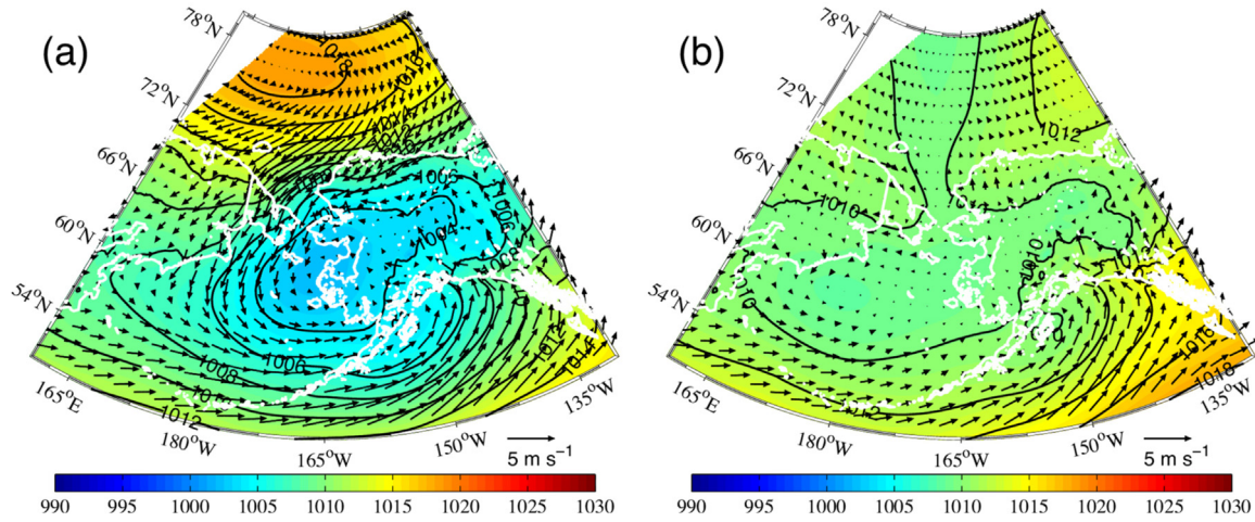
Fig. 13. Composites of sea level pressure (color, mb) and 10 m wind (vectors, \text{m s}^{-1} ) from NARR for (a) upwelling, and (b) non-upwelling periods. (For interpretation of the references to color in this figure legend, the reader is referred to the web version of this article.)
