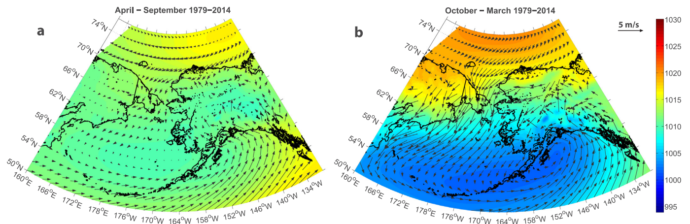
Fig. 6. Maps of climatological mean sea level pressure (mb, color) and 10-m winds (vectors) from NARR for the period 1979–2014. (a) the warm season (April–September); (b) the cold season (October–March). (For interpretation of the references to color in this figure legend, the reader is referred to the web version of this article.)
