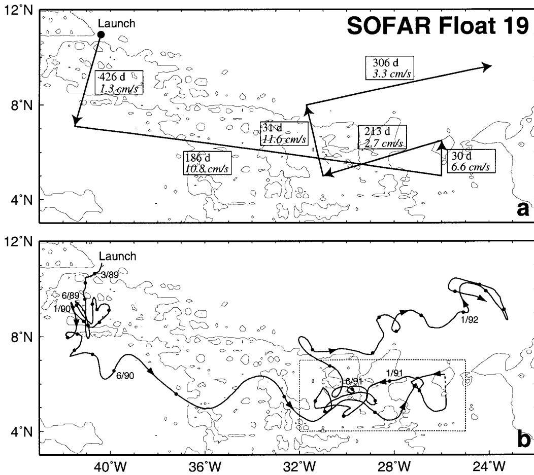
FIG. 5. (a) The trajectory of float 19 subdivided into six segments of generally distinct dynamical character. (b) The complete trajectory of float 19. Missing data is indicated by a dashed line. Solid dots are spaced at one-month intervals. The dashed box indicates the subregion of cyclonic looping examined in section 4 (see Fig. 10).
