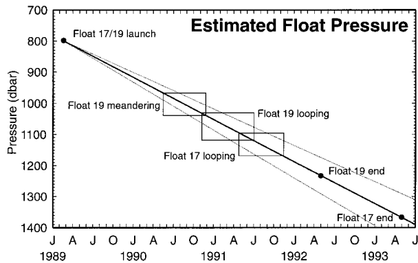
FIG. 2. Estimated pressure in dbar of floats 17 and 19 as a function of time (solid line). Dashed lines indicate an uncertainty estimate corresponding to one standard error of the float sink rate. A mean sink rate of 0.37 \pm 0.05 dbar/day was determined by Richardson et al. (1994a) for a sample of 10 aluminum-hulled floats similar to floats 17 and 19. The periods of float looping and meandering are indicated for reference. The uncertainty in the initial float depth is estimated to be approximately 50 dbar based on earlier experiments.
