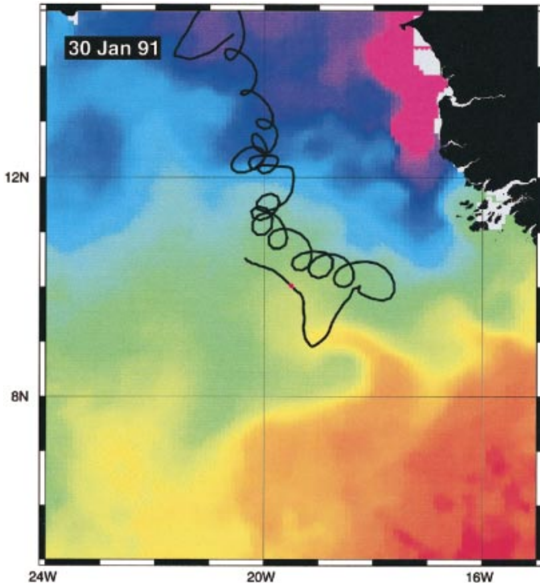
FIG. 13. Fourteen-day composite sea surface temperature image centered on 30 January 1991 in the eastern tropical Atlantic. The cold core, cyclonic recirculation near 8.5^{\circ}\text{N} , 19.7^{\circ}\text{W} within the crest of a breaking wave is approximately 100 km in diameter. The trajectory of float 17 during 1991 is shown. The location of the float on the date corresponding to the image is indicated by the red dot. The wave crests in this figure subsequently moved westward at about 8\text{ cm s}^{-1} . The color palette is the same as that used in Fig. 11.
