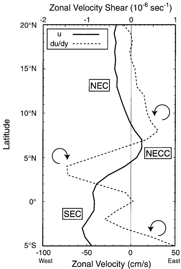
FIG. 12. The meridional variation of zonal velocity in the low-latitude eastern Atlantic Ocean. Curves depict the annual mean, zonally averaged ( 40^{\circ} – 15^{\circ} W) zonal velocity (solid: \text{cm s}^{-1} ) and the meridional gradient of zonal velocity (dashed: 10^{-6} \text{ s}^{-1} ) as a function of latitude. Values were computed from the global ship-drift climatology of Mariano et al. (1995). The approximate location of major zonal currents are indicated. Note in particular the region of positive (cyclonic; anticlockwise) shear between the NECC and the NEC with a maximum near 8^{\circ} N. This shear is relatively constant in the eastern Atlantic but varies seasonally in the western Atlantic (Richardson and McKee 1984).
