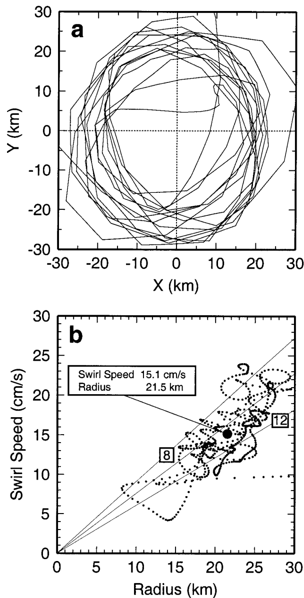
FIG. 8. (a) Residual rotational component of float 17 position (in kilometers relative to the eddy center) after the low-frequency translational component was removed by application of a low-pass Gaussian-shaped filter. (b) Scatterplot of swirl speed (defined as rms velocity about the low-passed velocity) versus radial distance from the eddy center. The general positive correlation suggests an eddy in solid-body rotation. Straight lines indicate slope corresponding to a solid-body rotation period of 8, 10, and 12 days. The mean swirl speed and radius are identified.
