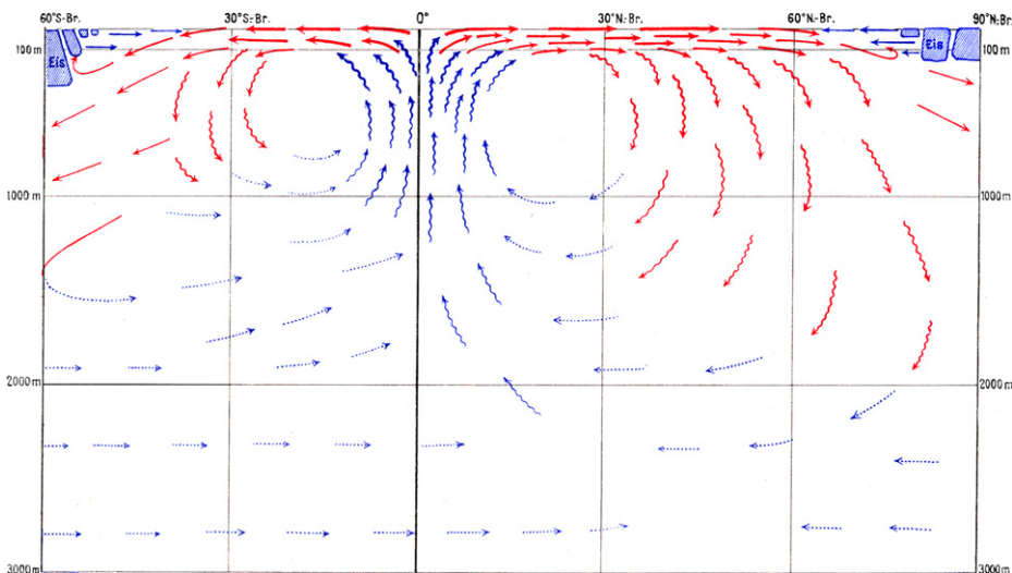
Fig. 3. Meridional overturning circulation scheme shown by Schott (1902).
