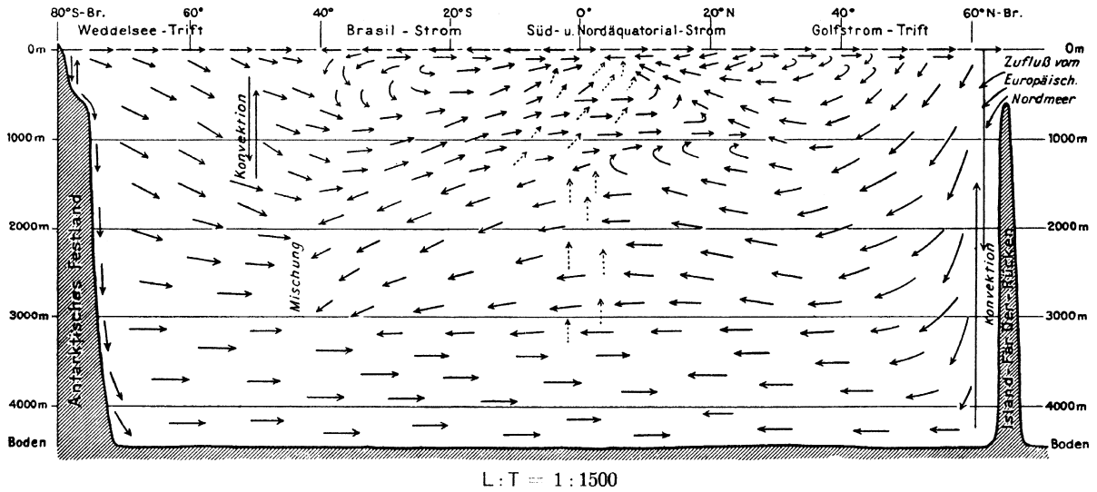
Fig. 5. Meridional circulation scheme mainly along the western Atlantic by Brennecke (1921). This figure clearly shows subsurface cross-equatorial flow by northward arrows near 1000 m and southward arrows centered near 3000 m.
