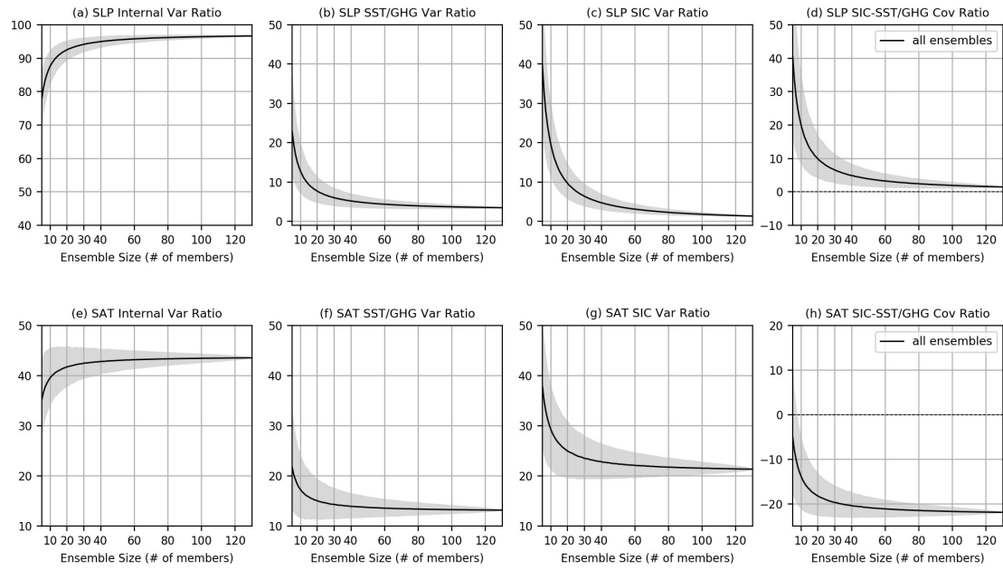
Figure S2. Ensemble size dependency for the ratio of estimated variances for each component to the total variance in percentage. The top row is for the Arctic Circle-averaged (65°N-90°N) DJF SLP decomposed into (a) internal atmospheric variability, (b) SST/GHG-driven variability, (c) SIC-driven variability, and (d) covariability between the SIC-driven and SST/GHG-driven components. For each given ensemble size, the ensemble members are randomly sampled without replacement 10,000 times. The color shadings indicate the 95-percentile range from 10,000 random selection and the average is plotted with the solid curves. (e)-(h) The same as (a)-(d) but for the near-surface air temperature in the same domain. The dashed lines in (d) and (h) are ratios for the residual components, which the 95-percentile ranges are also labeled but too small to be shown with the scale used here.
