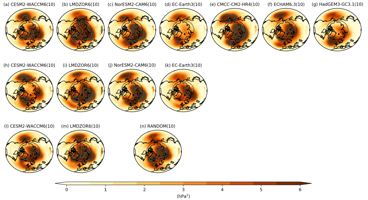
Figure S1. Arctic SIC-driven variance of DJF SLP using first ten members for (a) CESM2-WACCM6, (b) LMDZOR6, (c) NorESM2-CAM6, (d) EC-Earth3, (e) CMCC-CM2-HR4, (f) ECHAM6.3, and (g) HadGEM3-GC3.1. (h)-(k) The same as (a)-(d) but using second ten members. (l)-(m) The same as (a)-(b) but using third ten members. (n) The same as others but using 10 members randomly selected out of 130 members across seven AGCMs. The number in the parenthesis denotes ensemble size used. The cyan contour lines denote values larger than 6 \text{ hPa}^2 with interval 2 \text{ hPa}^2 . The black circle corresponds to 65^\circ\text{N} to denote the Arctic Circle.
